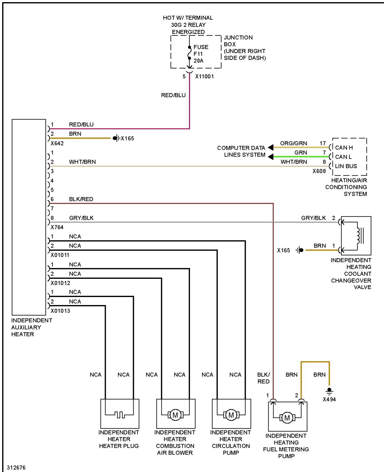
Fig. 10: Independent Heating Circuit
