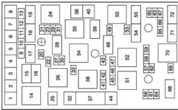
Chevrolet HHR – fuse box – engine compartment fuse
