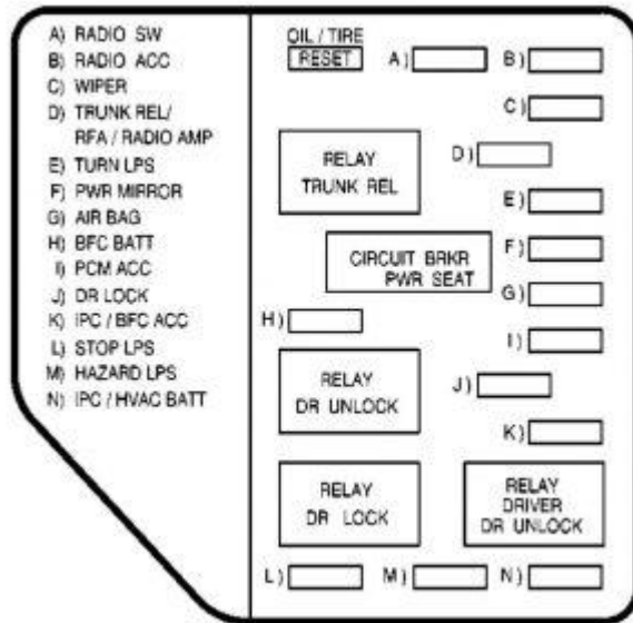
Pontiac Grand Am – fuse box – instrument panel (driver's side)
