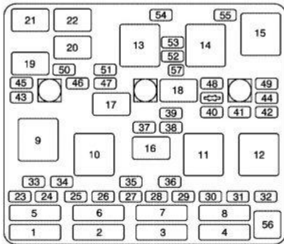
Pontiac Grand Am – fuse box – engine
