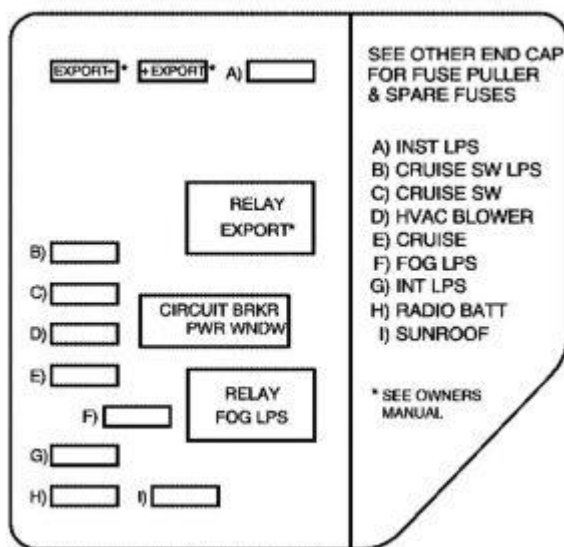
Pontiac Grand Am – fuse box – instrument panel (passenger's side)
