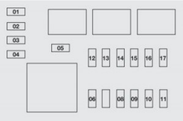
Fiat Grande Punto – fuse box – boot compartment
