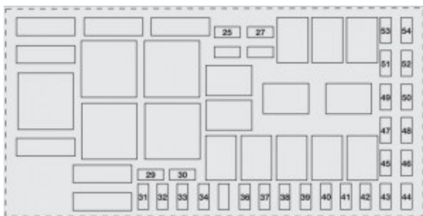
Fiat Grande Punto – fuse box – engine
