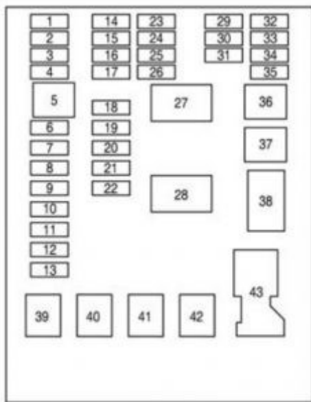
Chevrolet Aveo – fuse box – instrument panel
