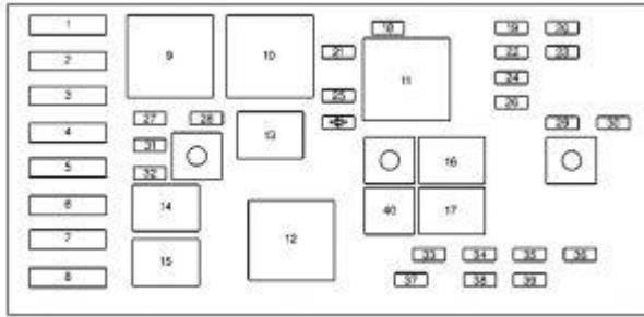
Pontiac Grand Prix – fuse box – engine compartment
