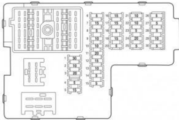
Lincol Aviator – fuse box – passenger
