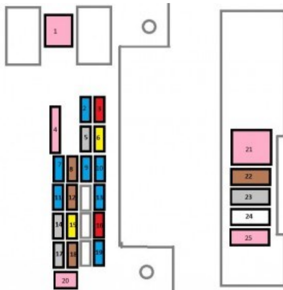
Citroen C4 Aircross – fuse box – under dashboard
