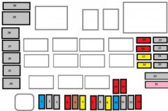
Citroen C4 Aircross – fuse box – engine
