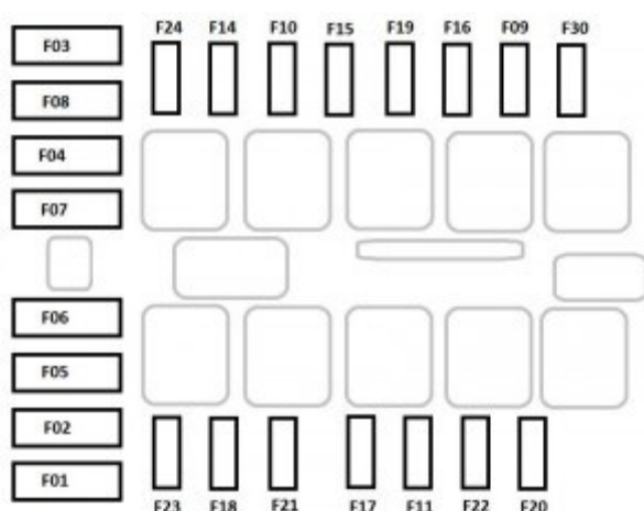
Fiat Ducato mk3 FL – fuse box – engine
