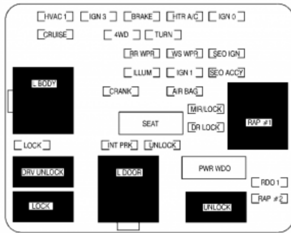
Chevrolet Tahoe – fuse box – instrument panel
