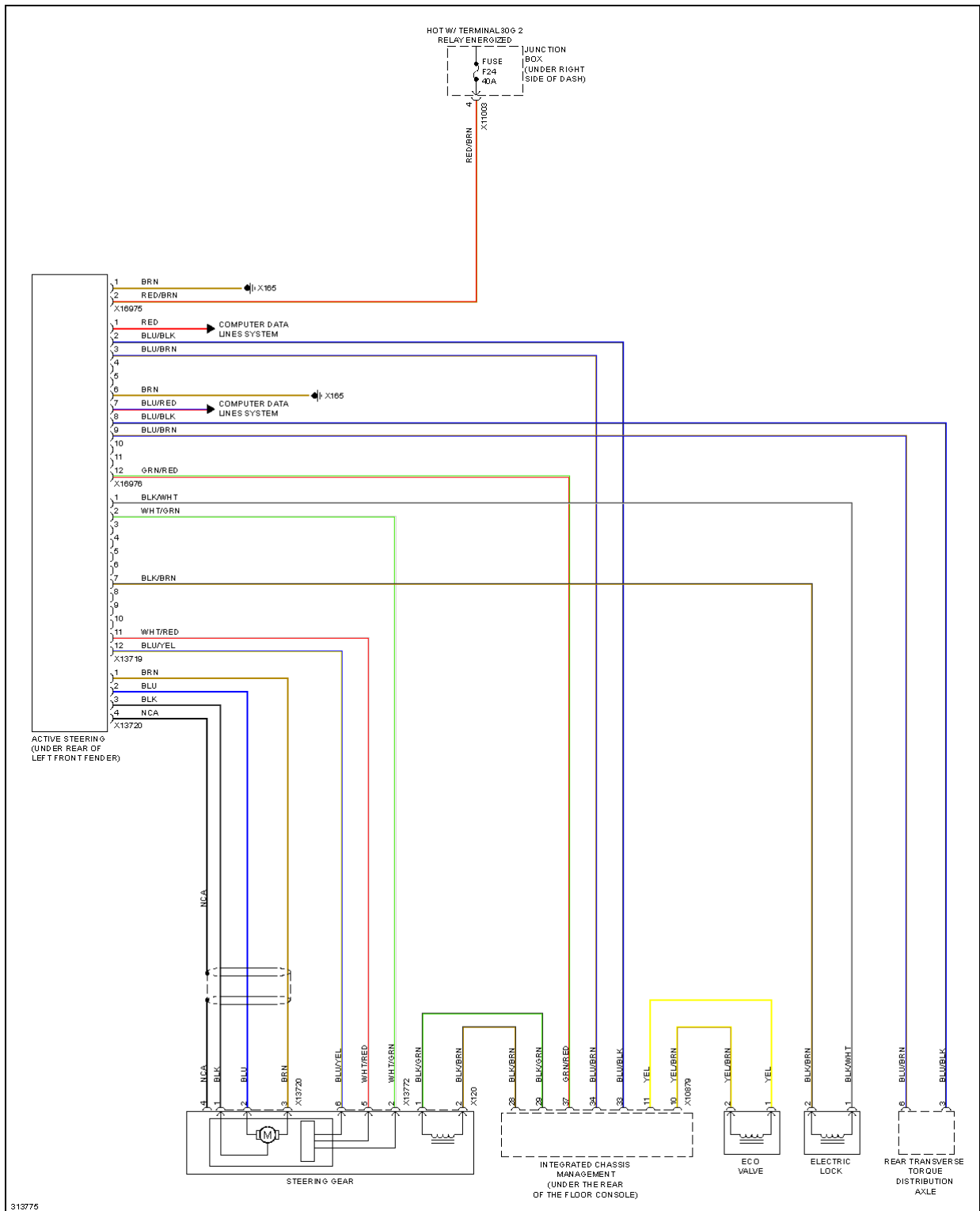
Fig. 27: Electronic Power Steering Circuit, W/ AL Active Steering
