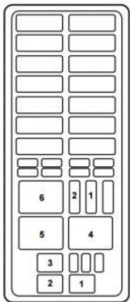
Mercury Mountaineer First Generation – fuse box – relays
