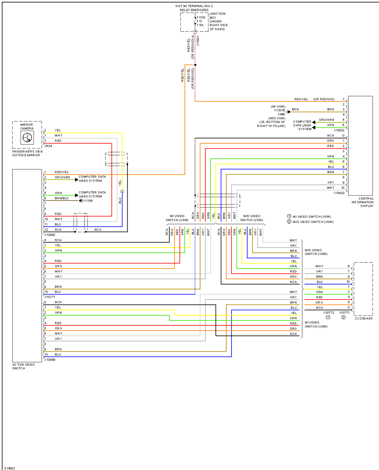
Fig. 78: Outside Mirror Camera Circuit
