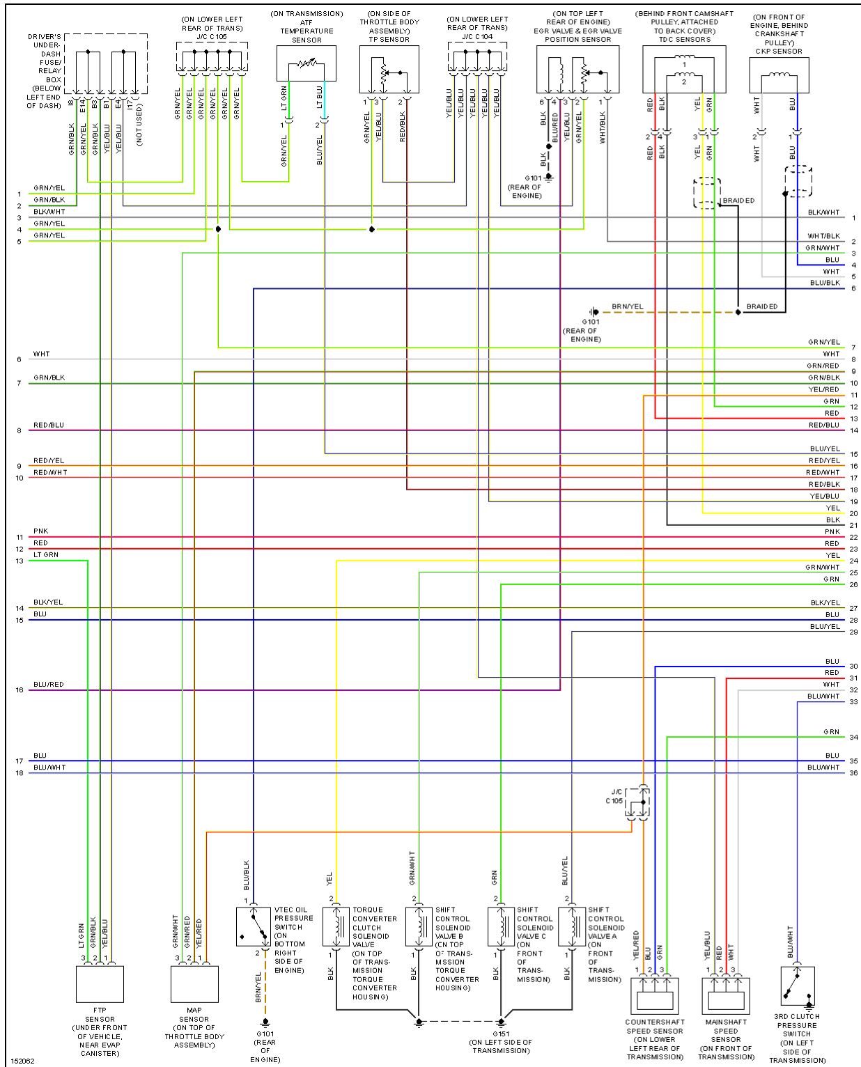
Fig. 26: 3.5L, Engine Performance Circuits (4 of 6)
