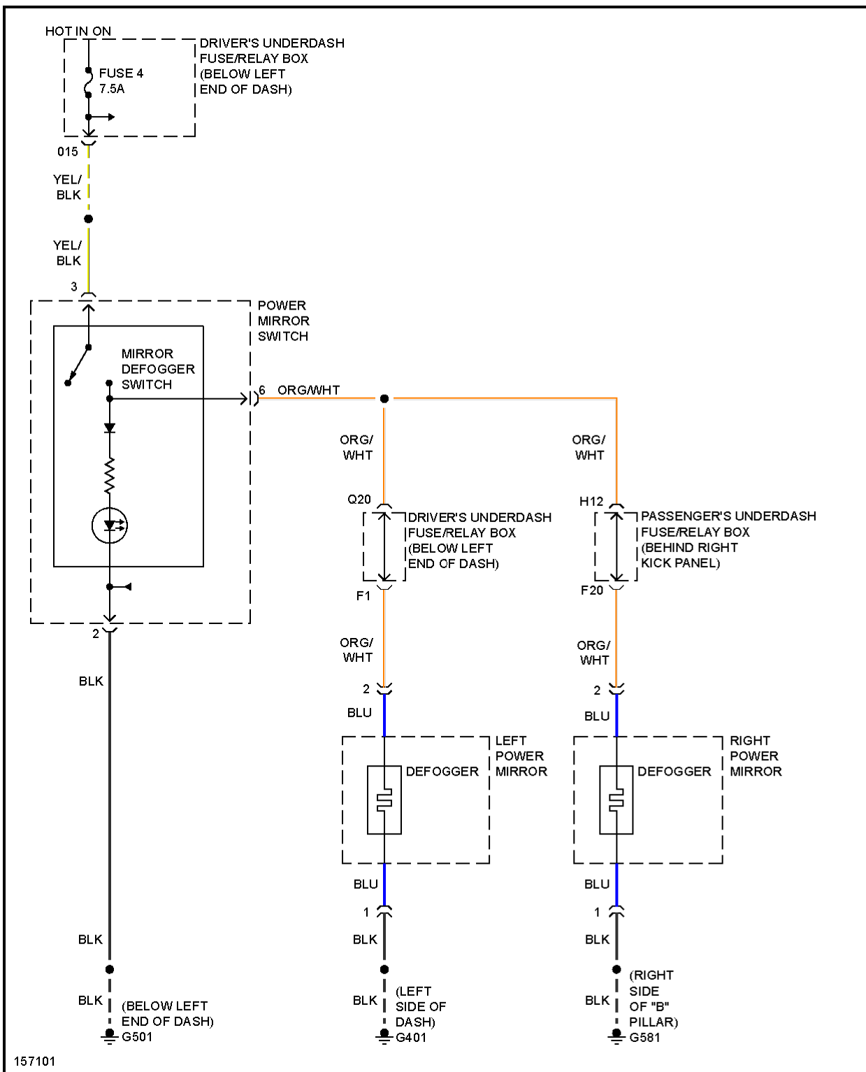
Fig. 21: Heated Mirrors Circuit
