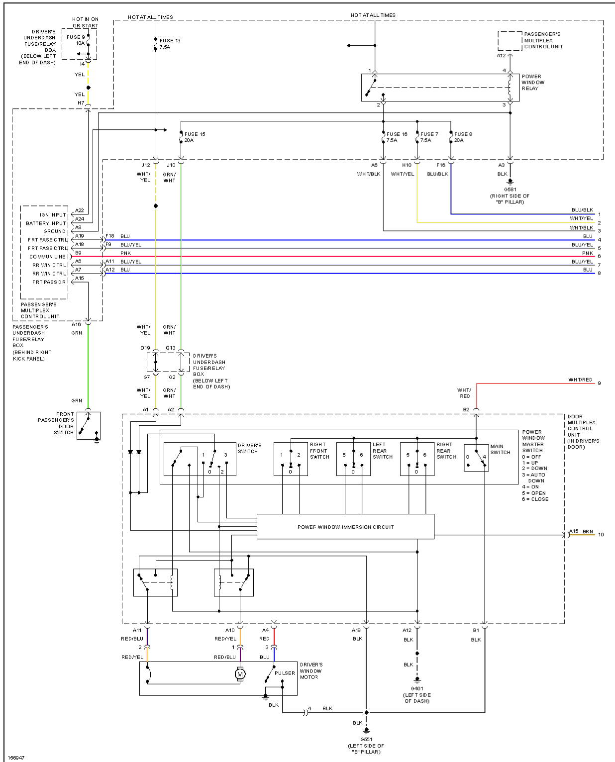
Fig. 62: Power Window Circuit (1 of 2)
