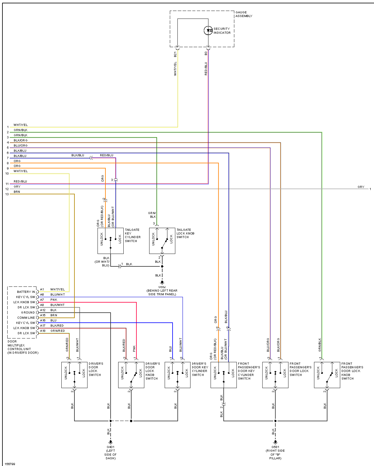
Fig. 11: Anti-theft Circuit, Except LX (2 of 3)
