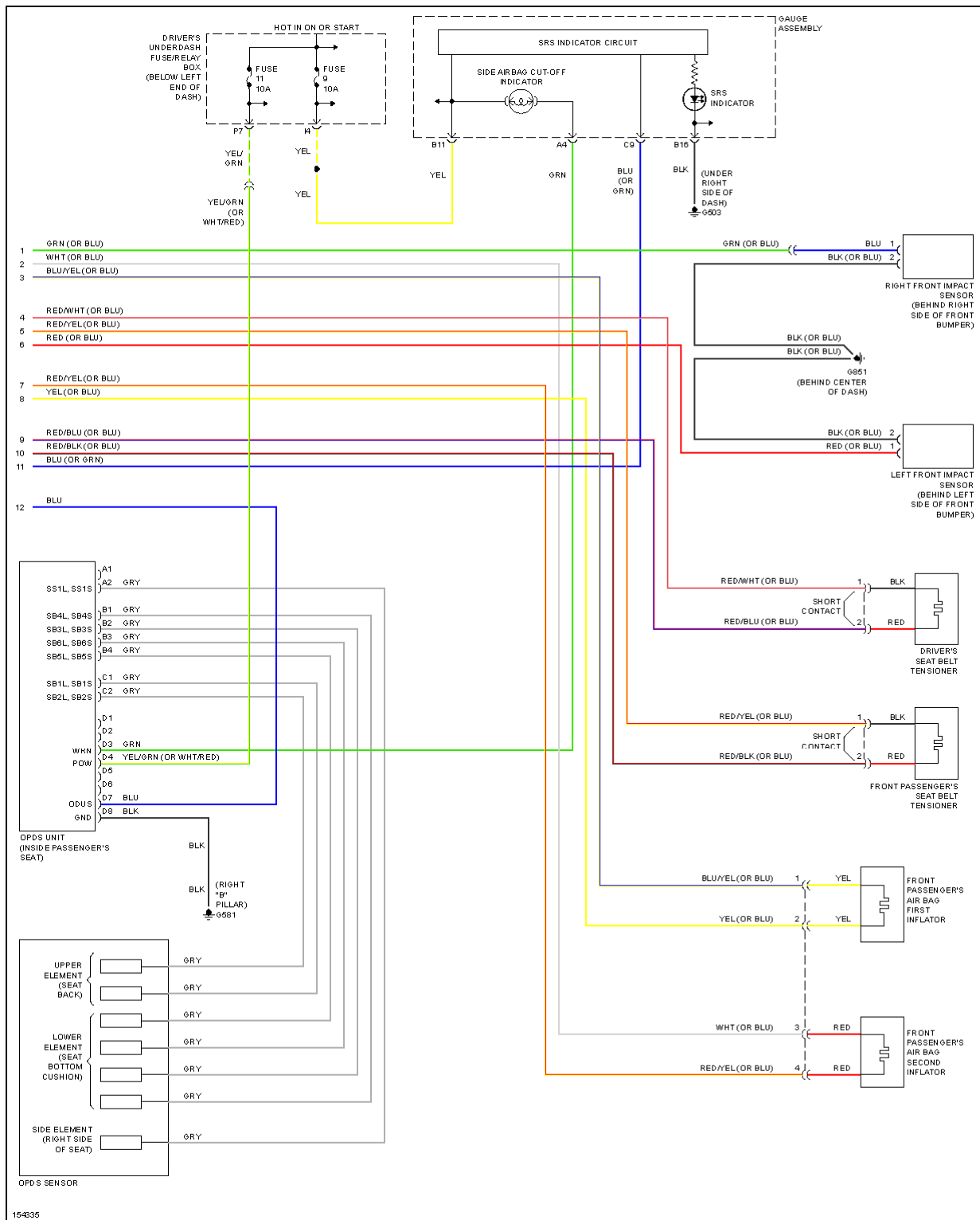
Fig. 74: Supplemental Restraint Circuit (2 of 2)
