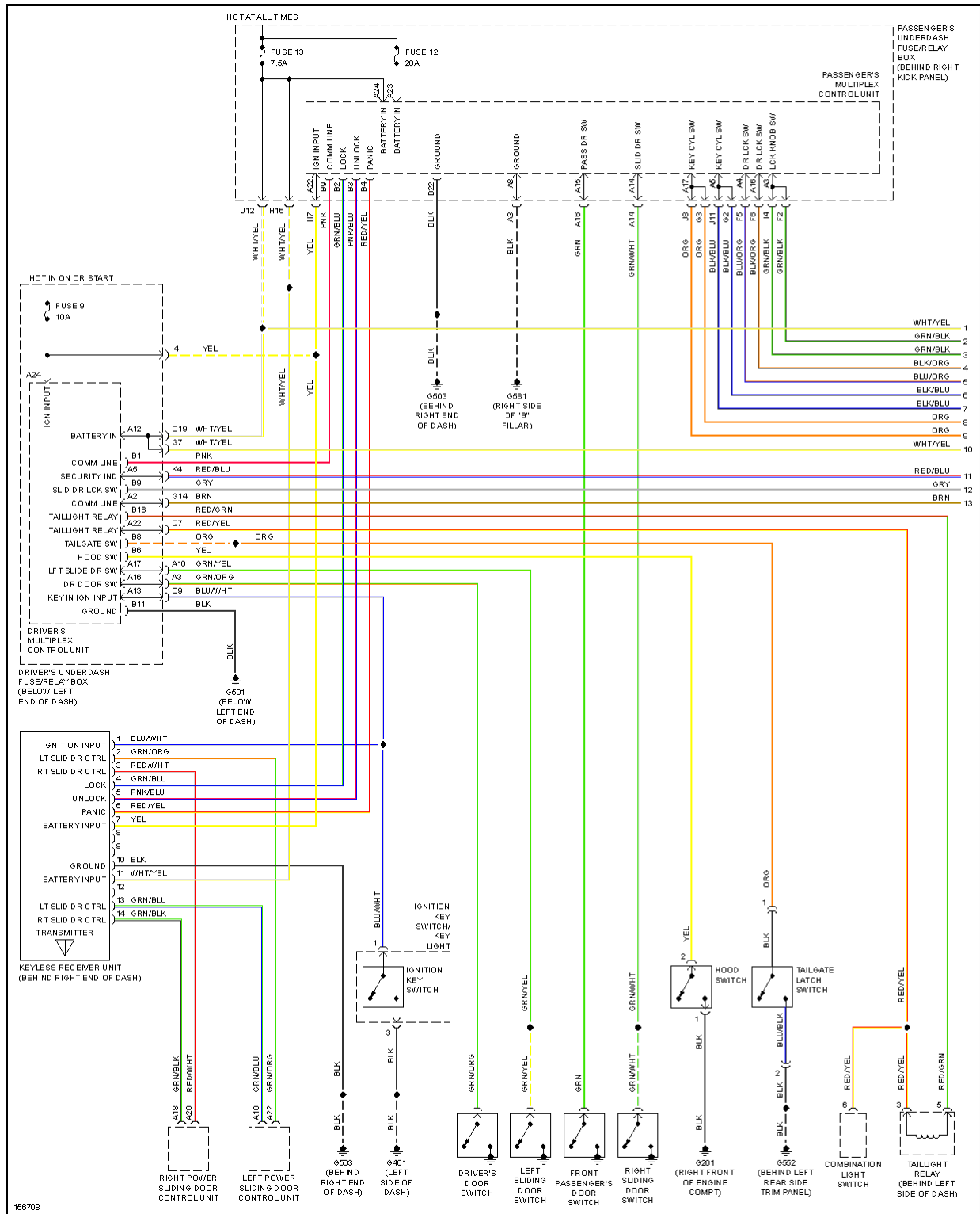
Fig. 51: Power Door Lock Circuit, Except LX (1 of 3)
