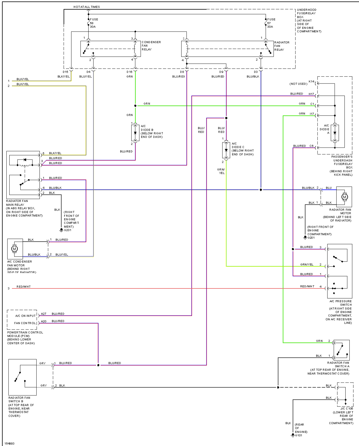
Fig. 4: Automatic A/C Circuit, W/O Navigation (2 of 2)
