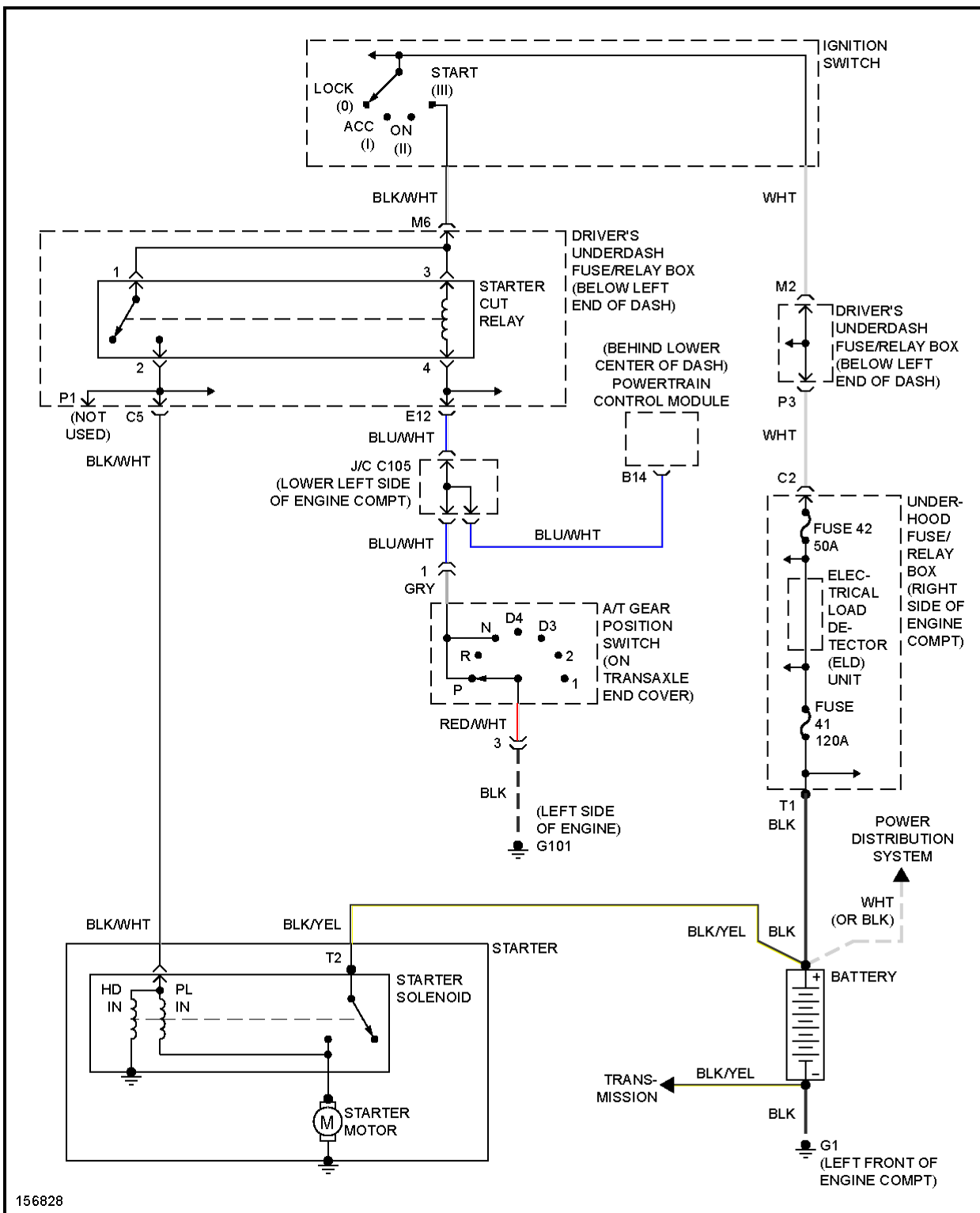
Fig. 72: Starting Circuit
