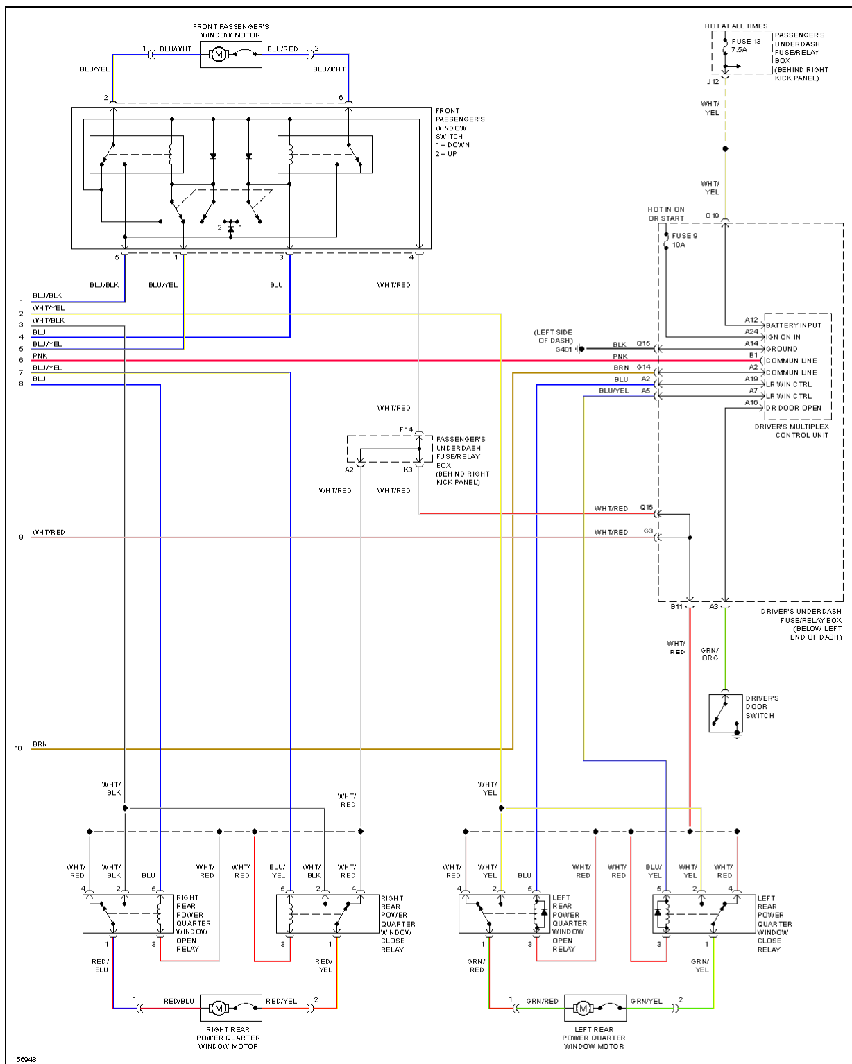
Fig. 63: Power Window Circuit (2 of 2)
