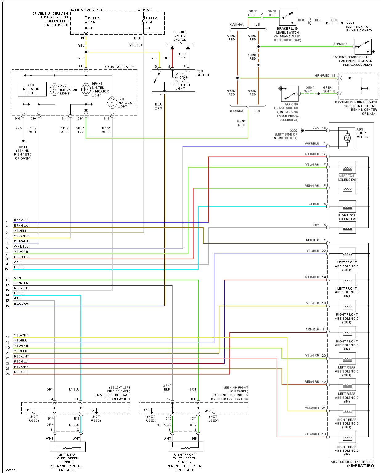
Fig. 9: Anti-lock Brake Circuits (2 of 2)
