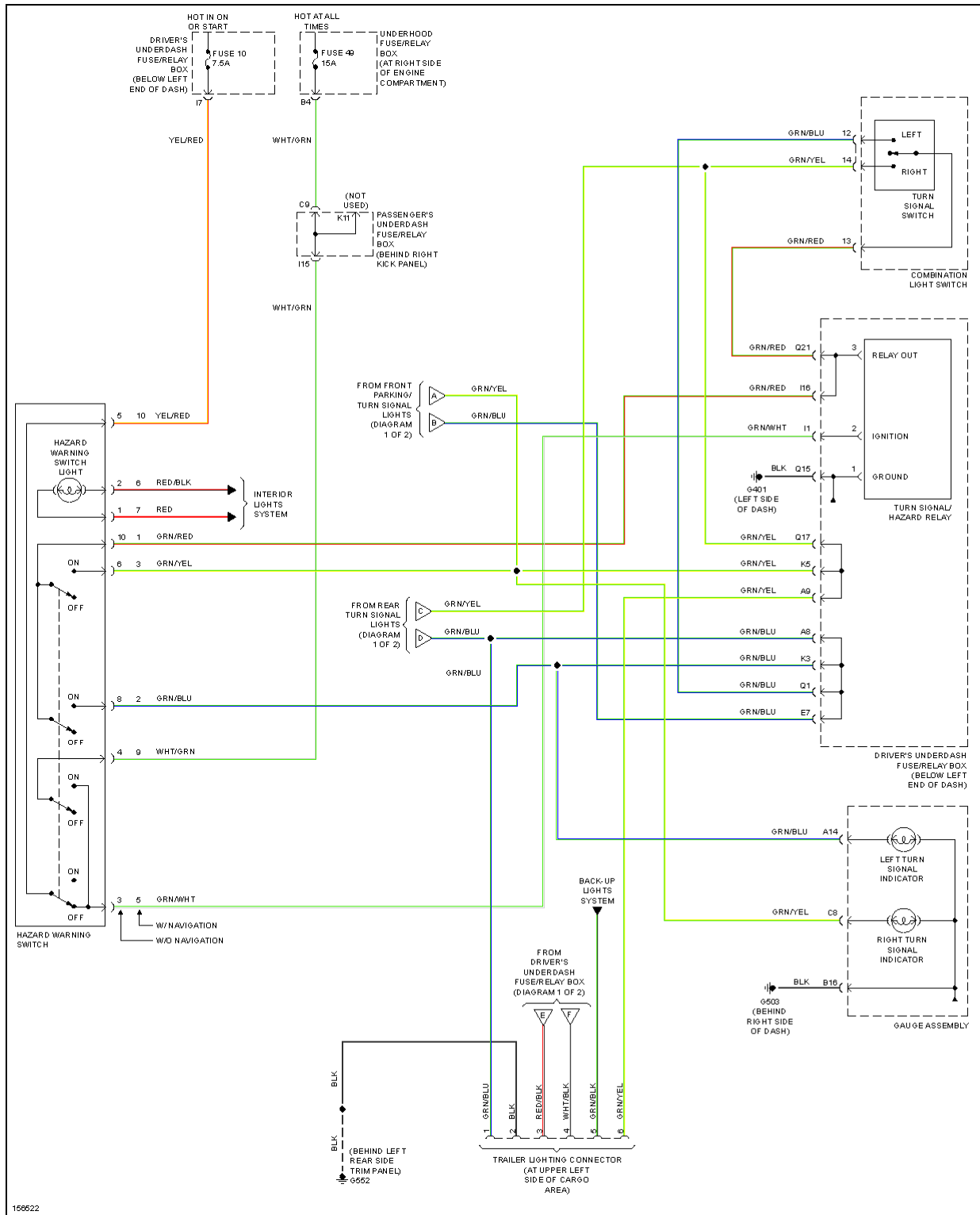
Fig. 31: Exterior Lamps Circuit (2 of 2)
