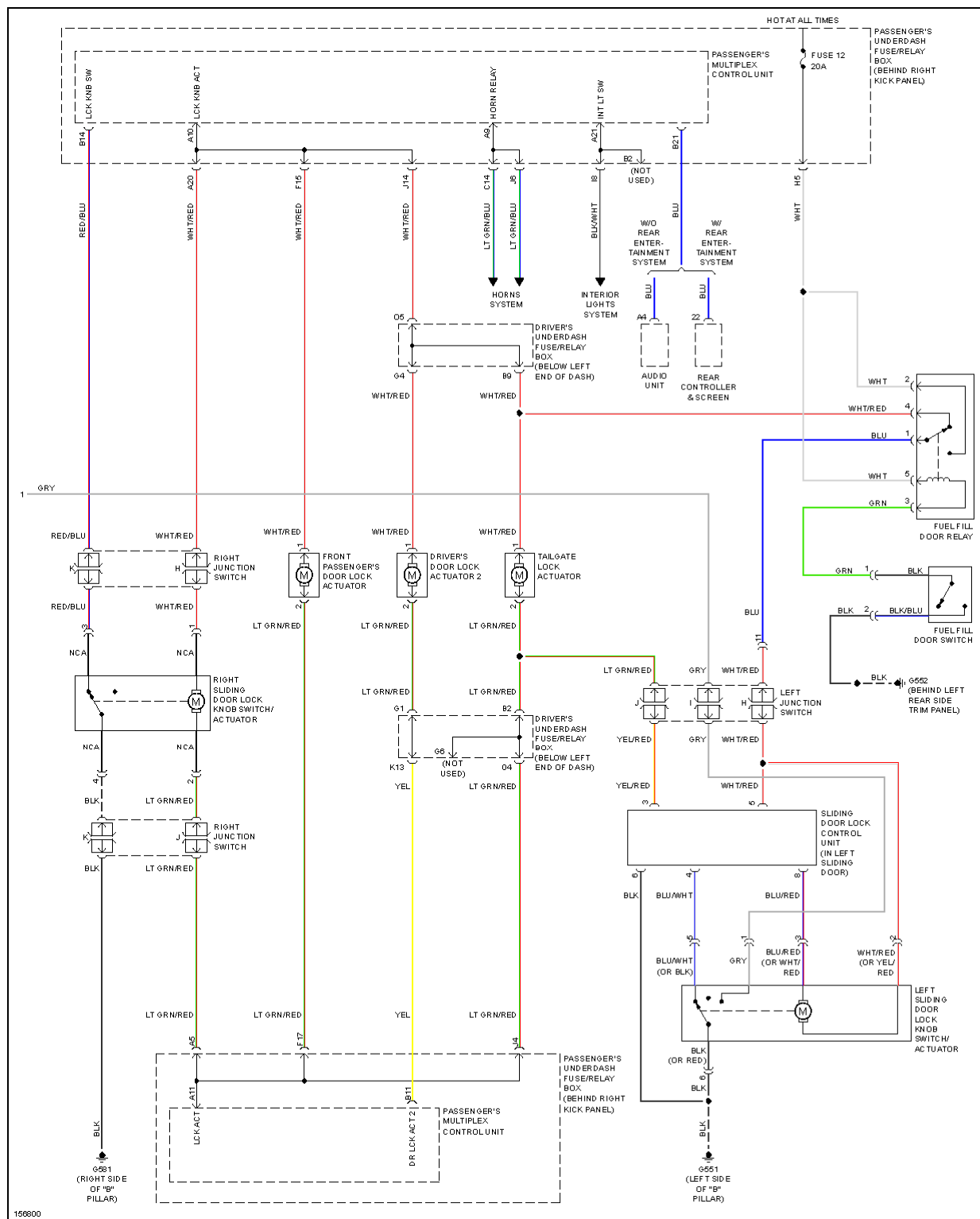
Fig. 12: Anti-theft Circuit, Except LX (3 of 3)
