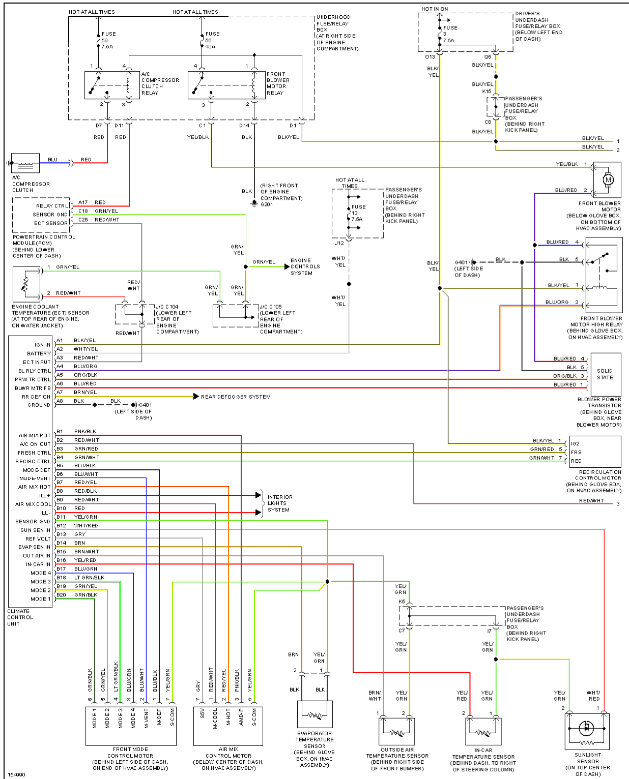
Fig. 3: Automatic A/C Circuit, W/O Navigation (1 of 2)
