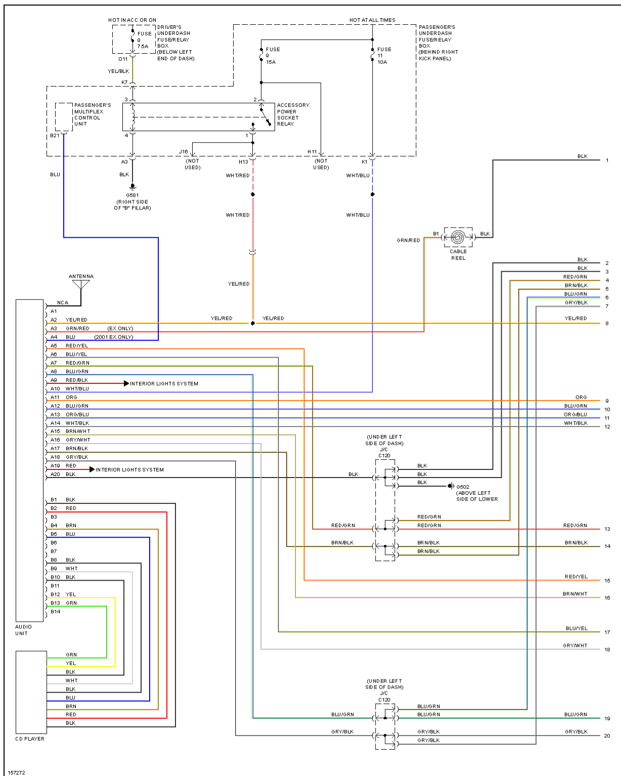
Fig. 68: Radio Circuits, W/ Subwoofer (1 of 2)
