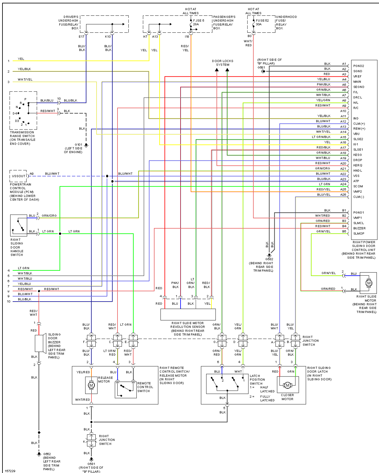
Fig. 78: Power Sliding Door Circuit (2 of 2)
