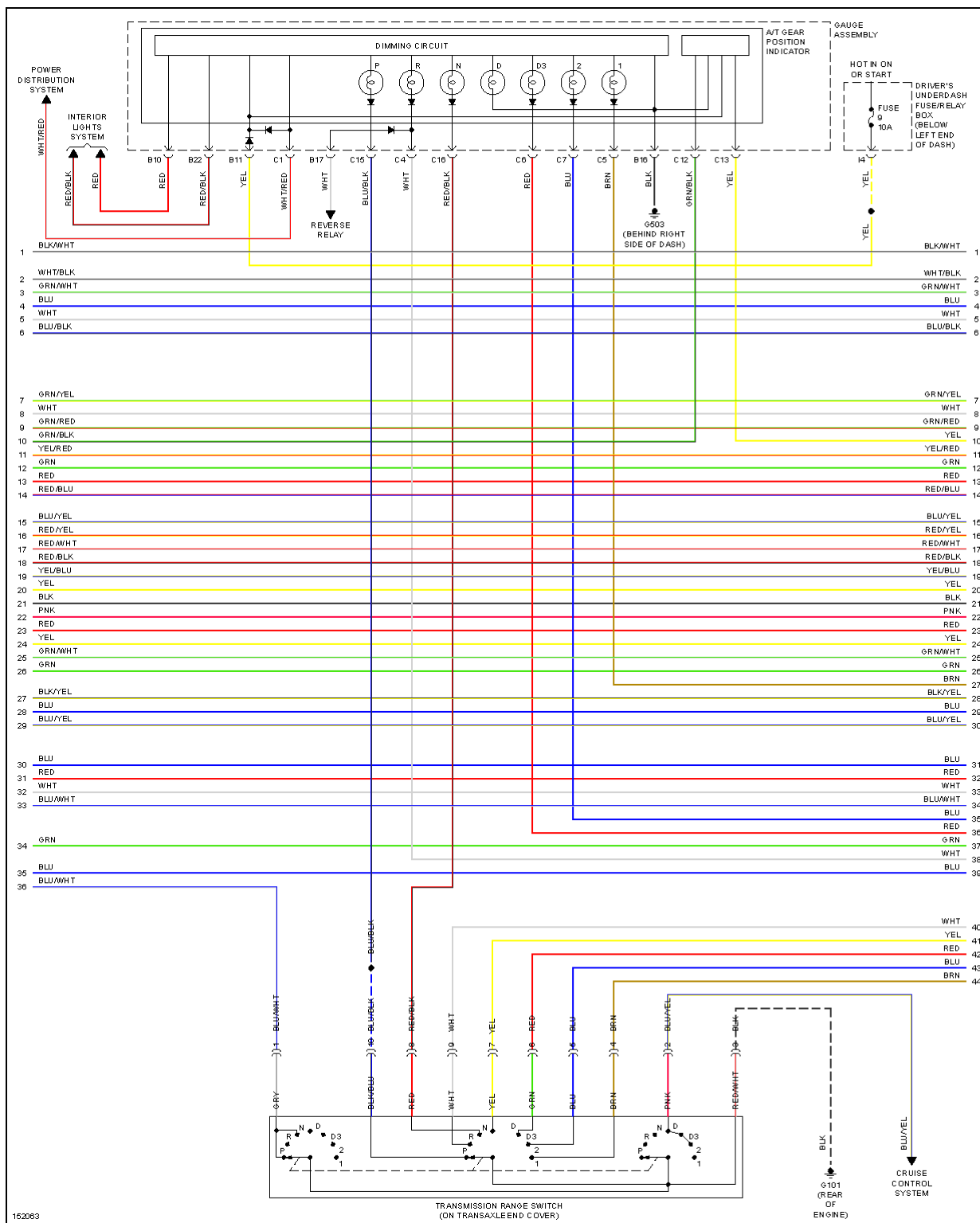
Fig. 27: 3.5L, Engine Performance Circuits (5 of 6)
