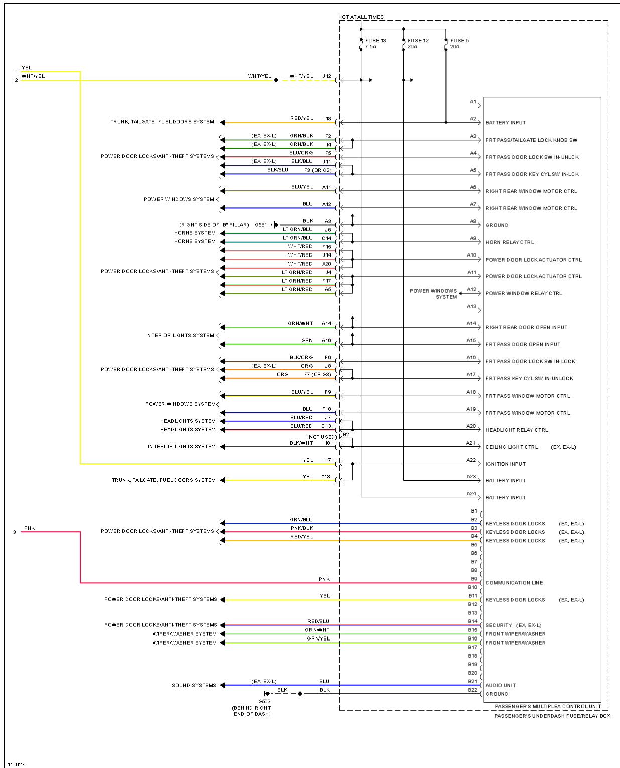
Fig. 17: Multiplex Control Circuit (2 of 2)
