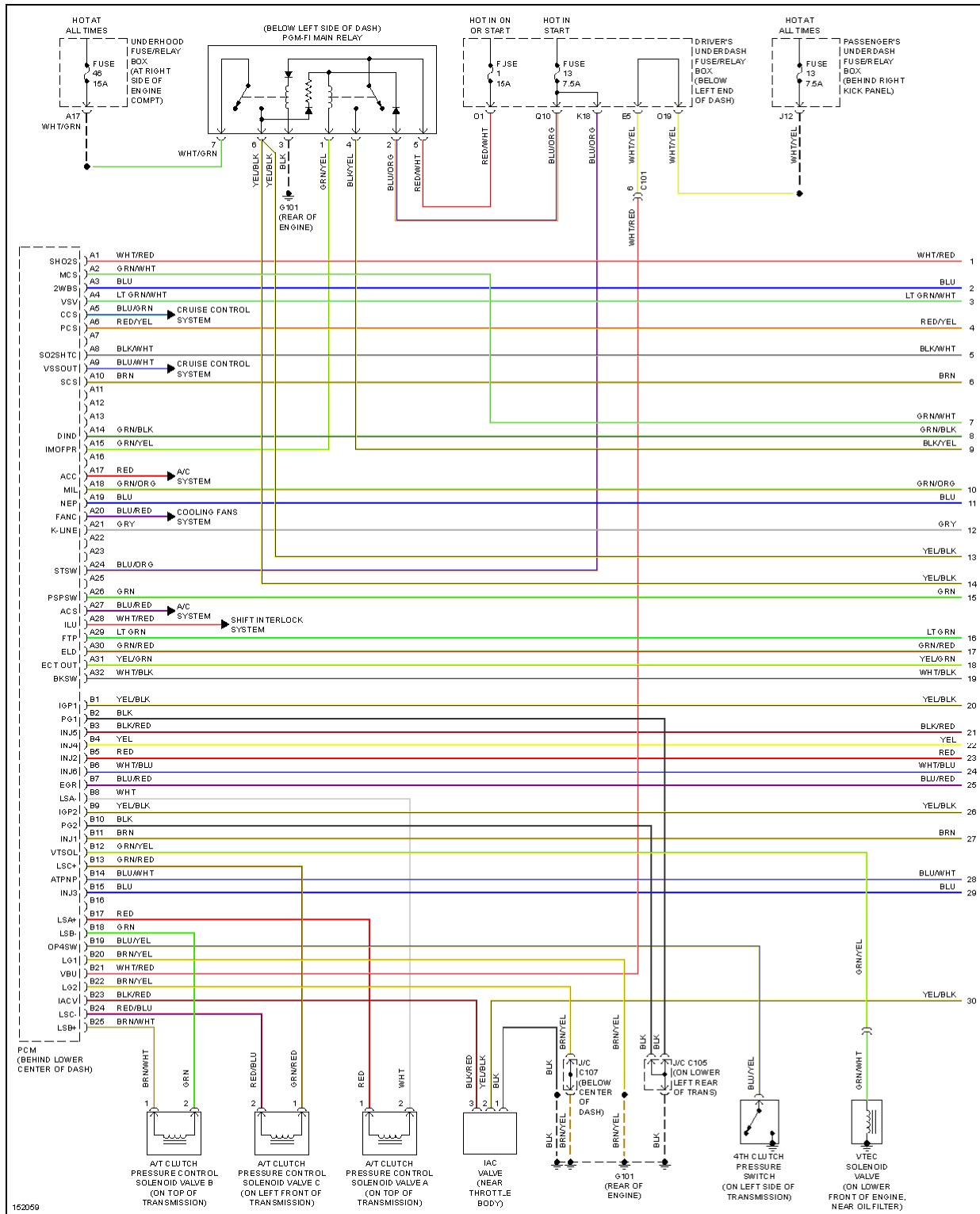
Fig. 23: 3.5L, Engine Performance Circuits (1 of 6)
