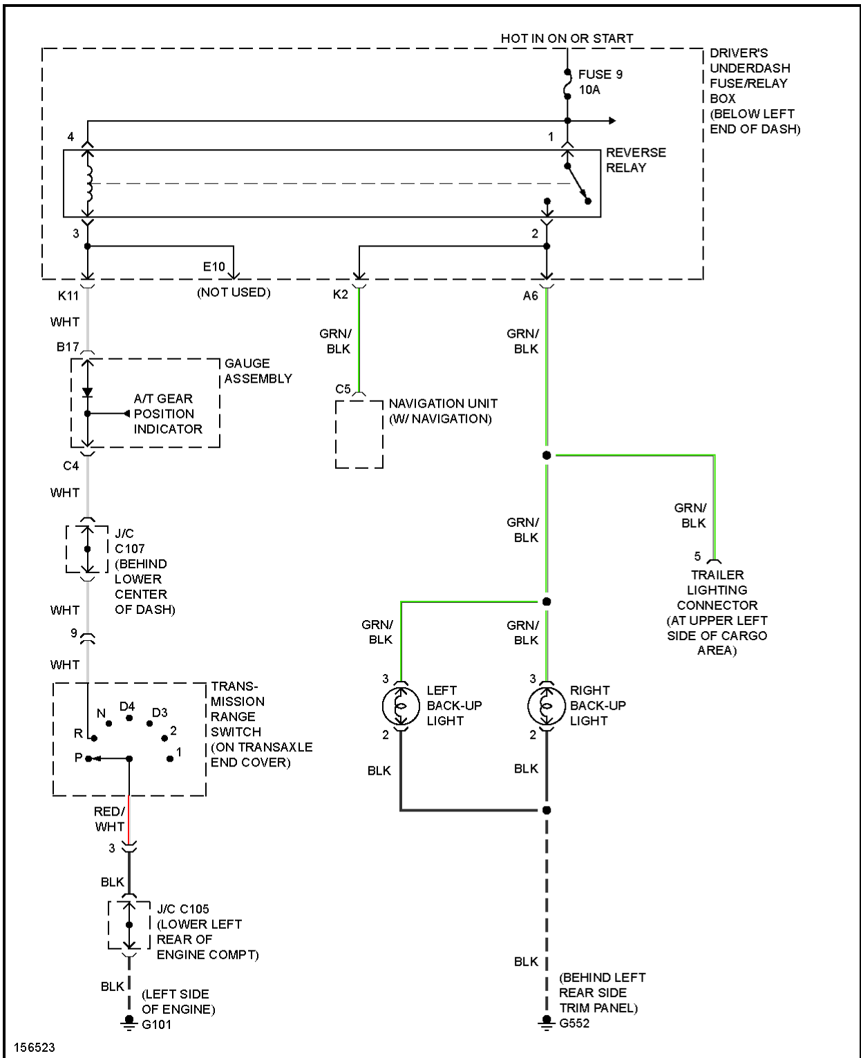
Fig. 29: Back-up Lamps Circuit
