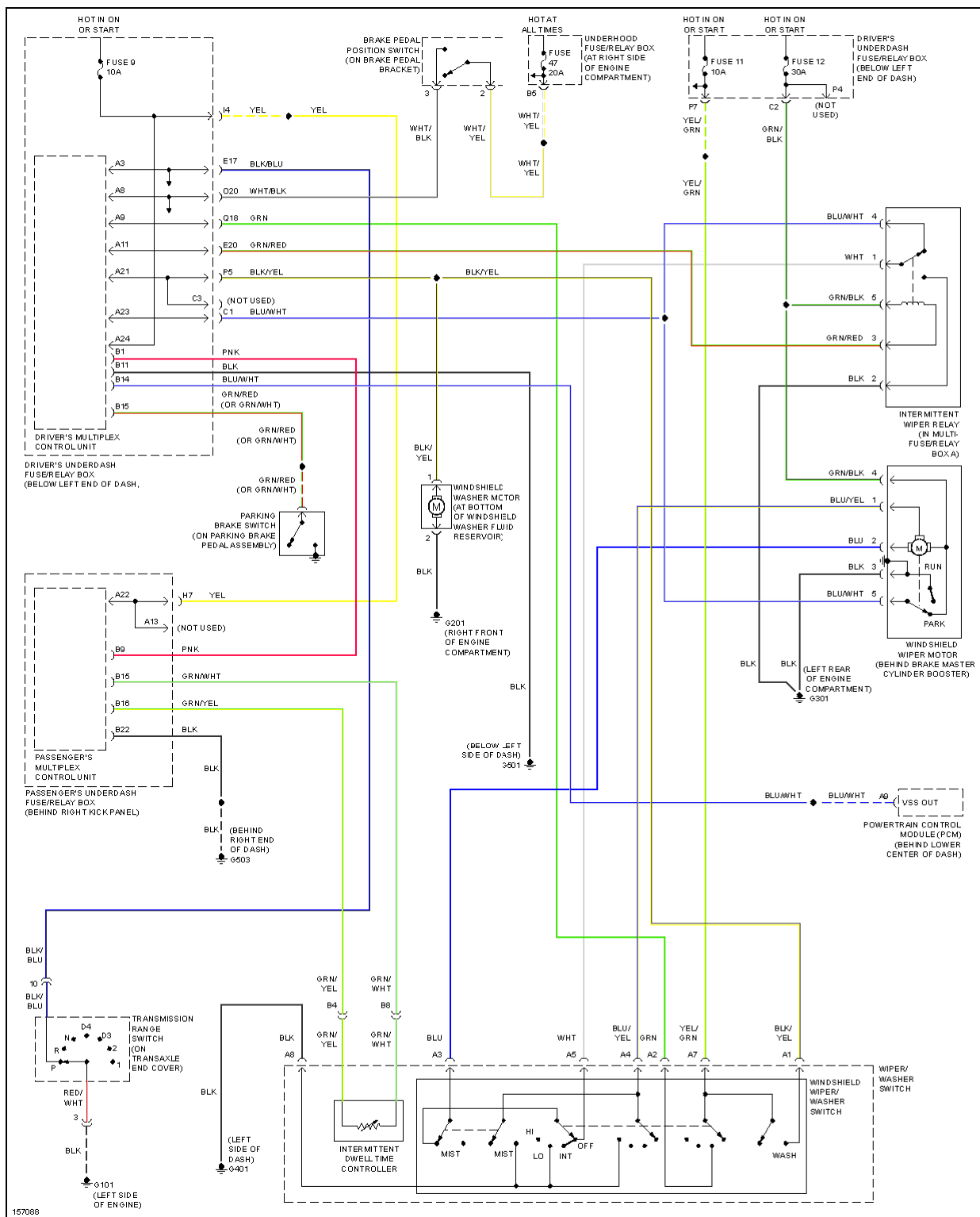
Fig. 80: Front Washer/Wiper Circuit
