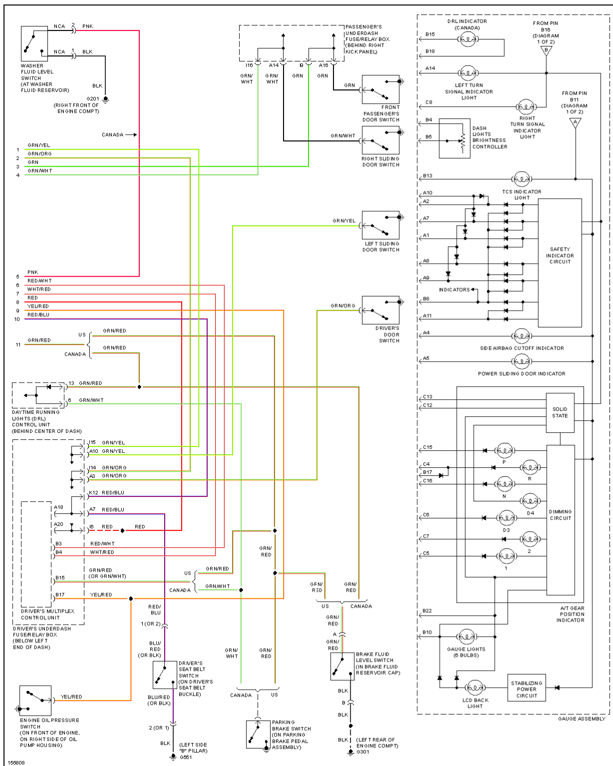
Fig. 41: Instrument Cluster Circuit (2 of 2)
