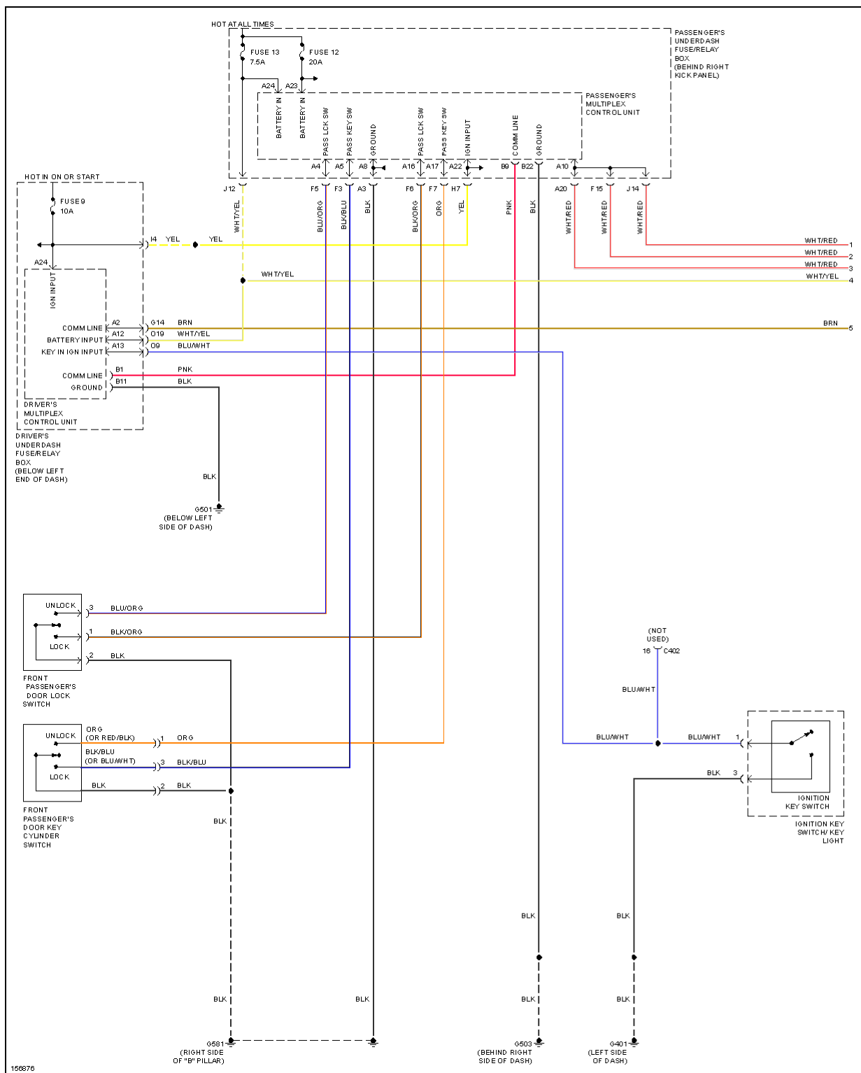
Fig. 56: Power Door Lock Circuit, LX W/O Keyless Entry (1 of 2)
