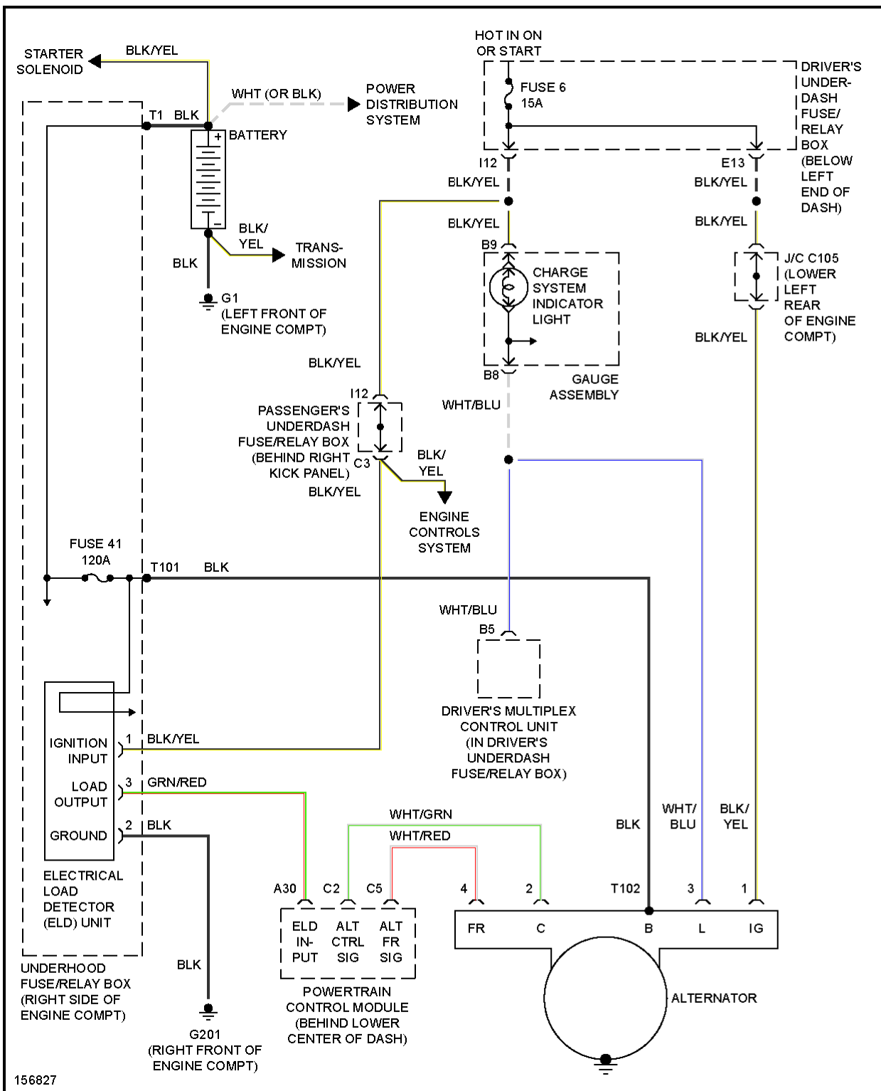
Fig. 71: Charging Circuit
