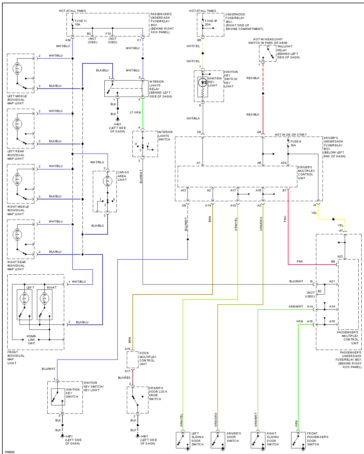
Fig. 43: Entry Light Timer Circuit
