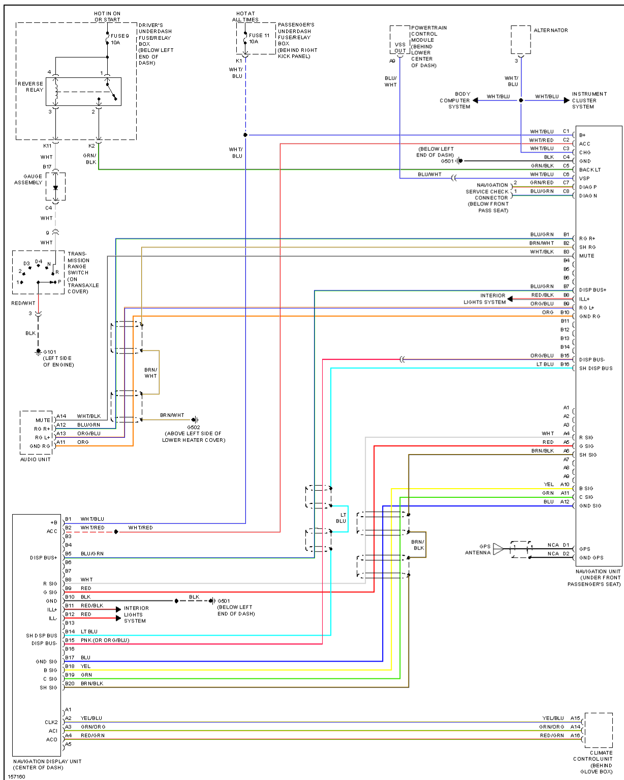
Fig. 46: Navigation Circuit
