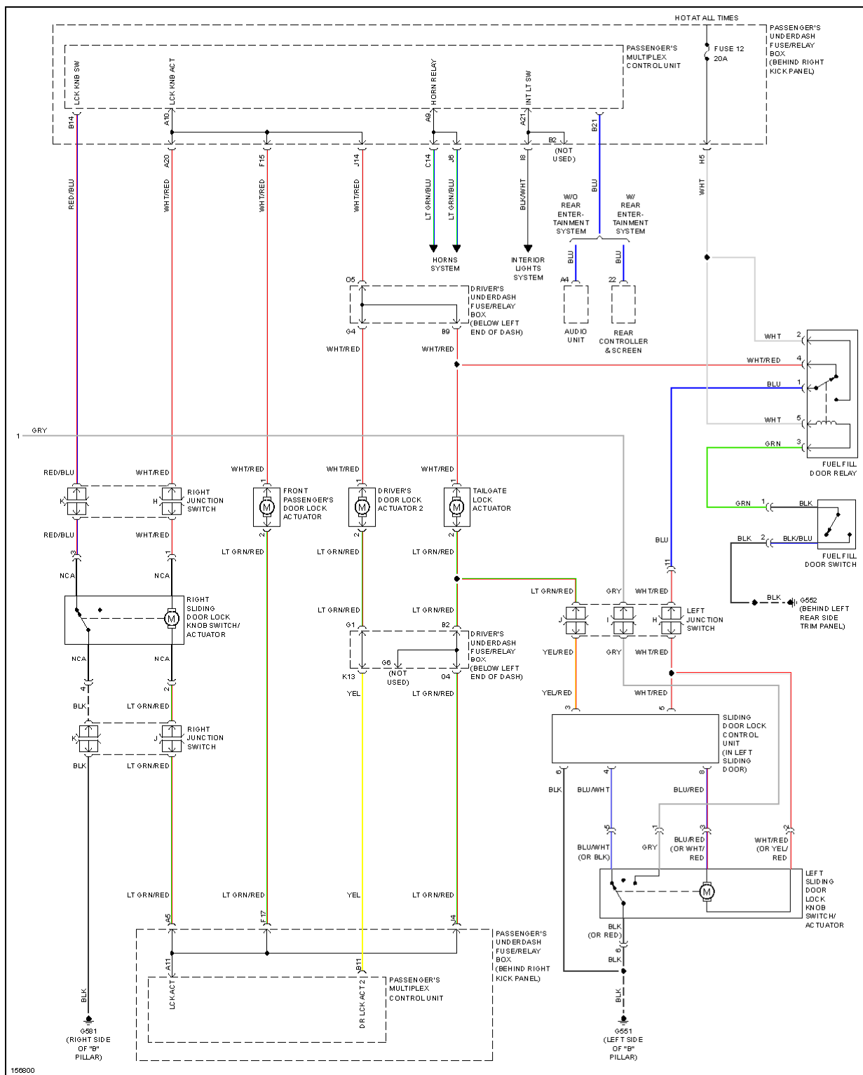
Fig. 53: Power Door Lock Circuit, Except LX (3 of 3)
