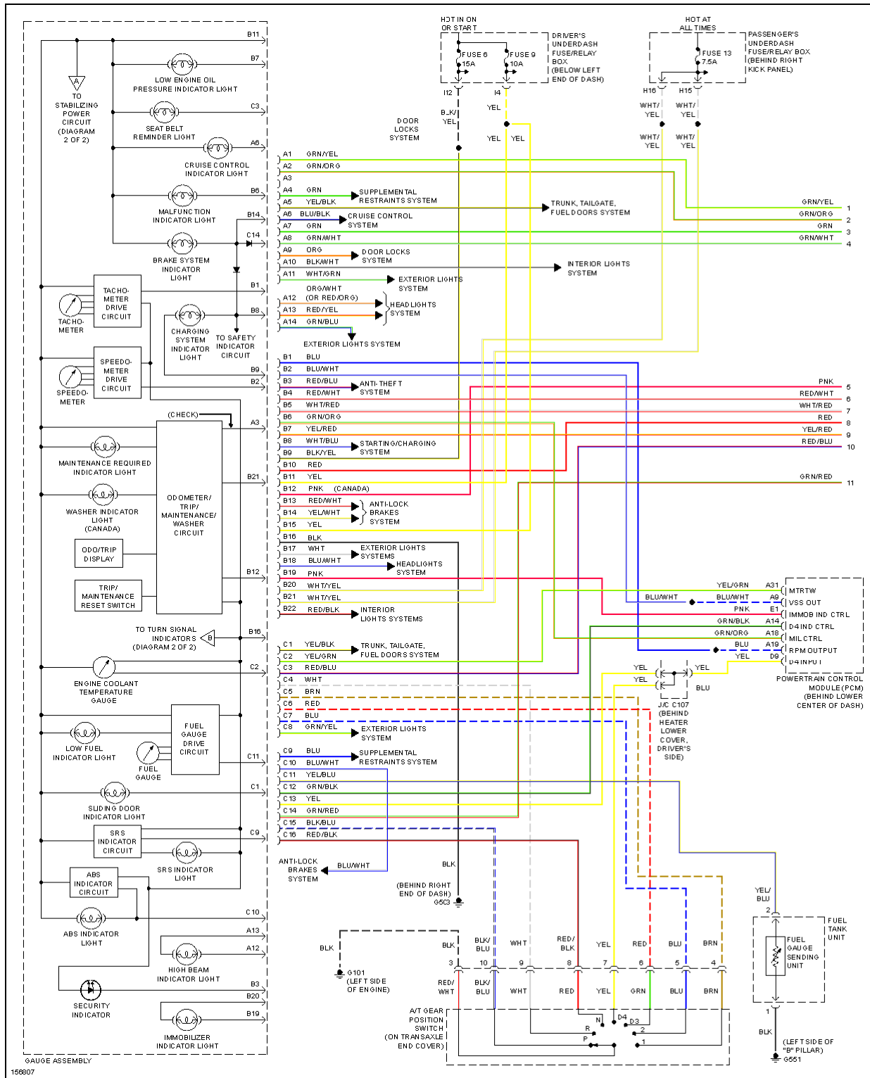
Fig. 40: Instrument Cluster Circuit (1 of 2)
