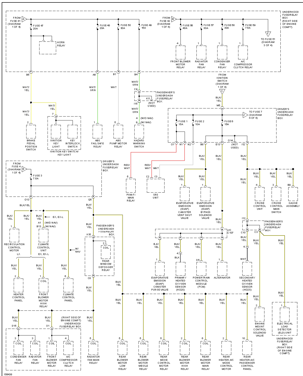
Fig. 48: Power Distribution Circuit (2 of 4)
