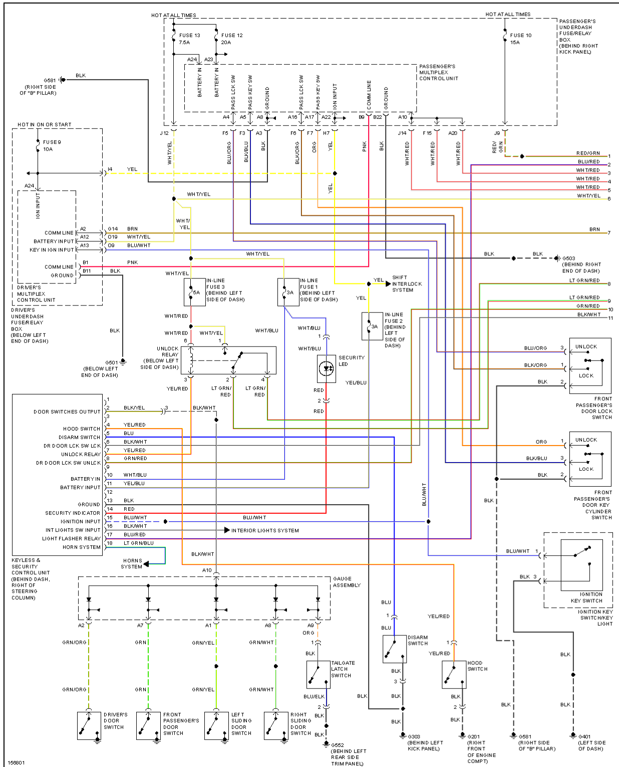
Fig. 54: Power Door Lock Circuit, LX W/ Keyless Entry (1 of 2)
