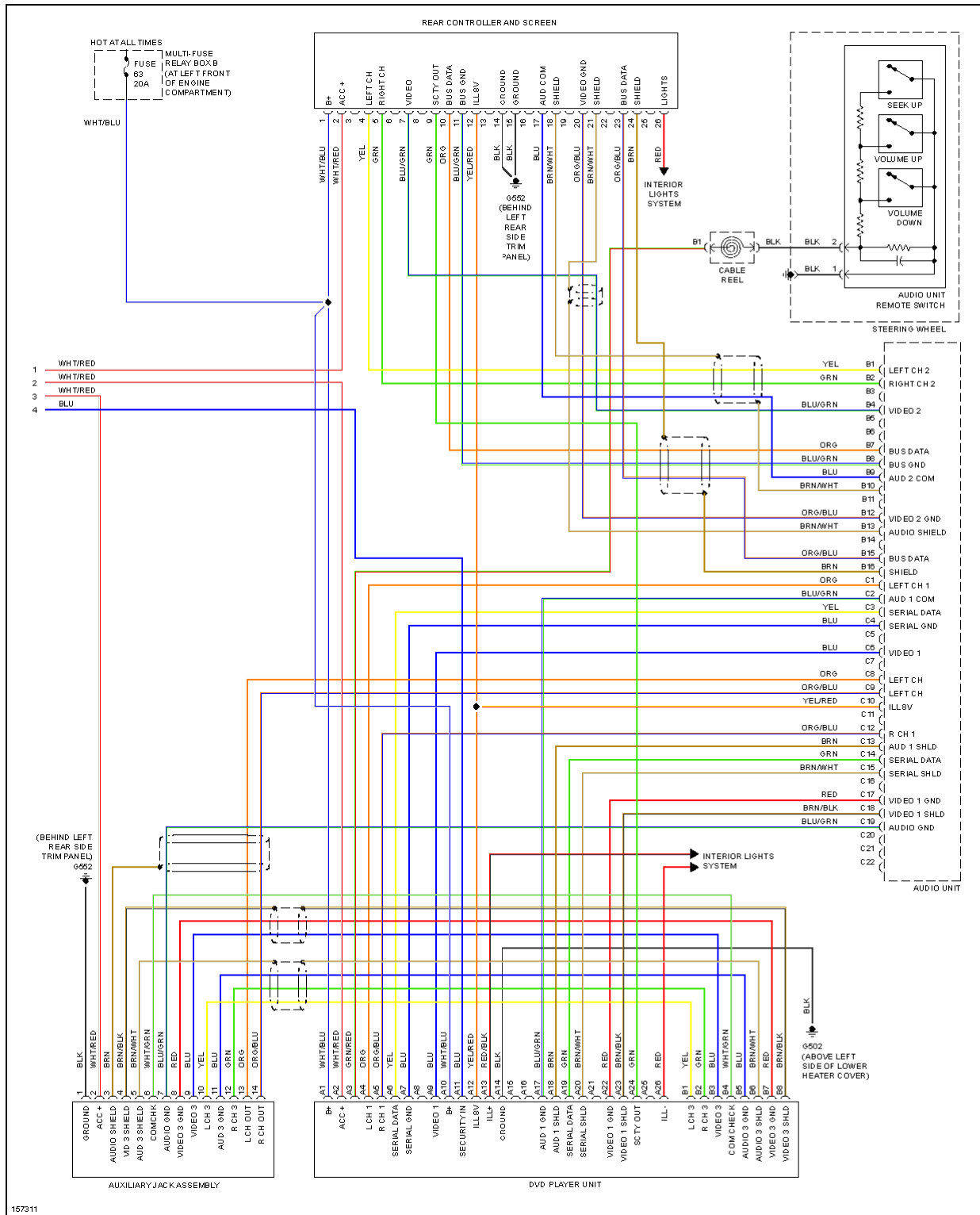
Fig. 67: Radio Circuits, W/ DVD (2 of 2)
