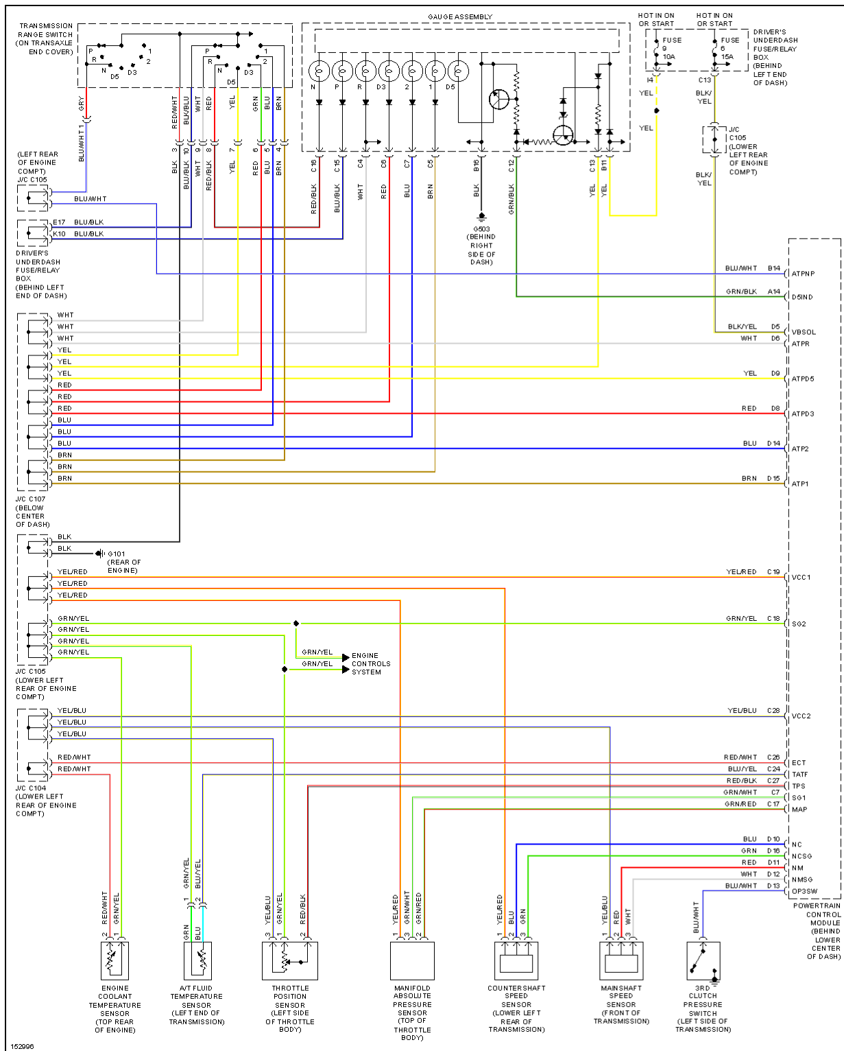
Fig. 76: A/T Circuit (2 of 2)
