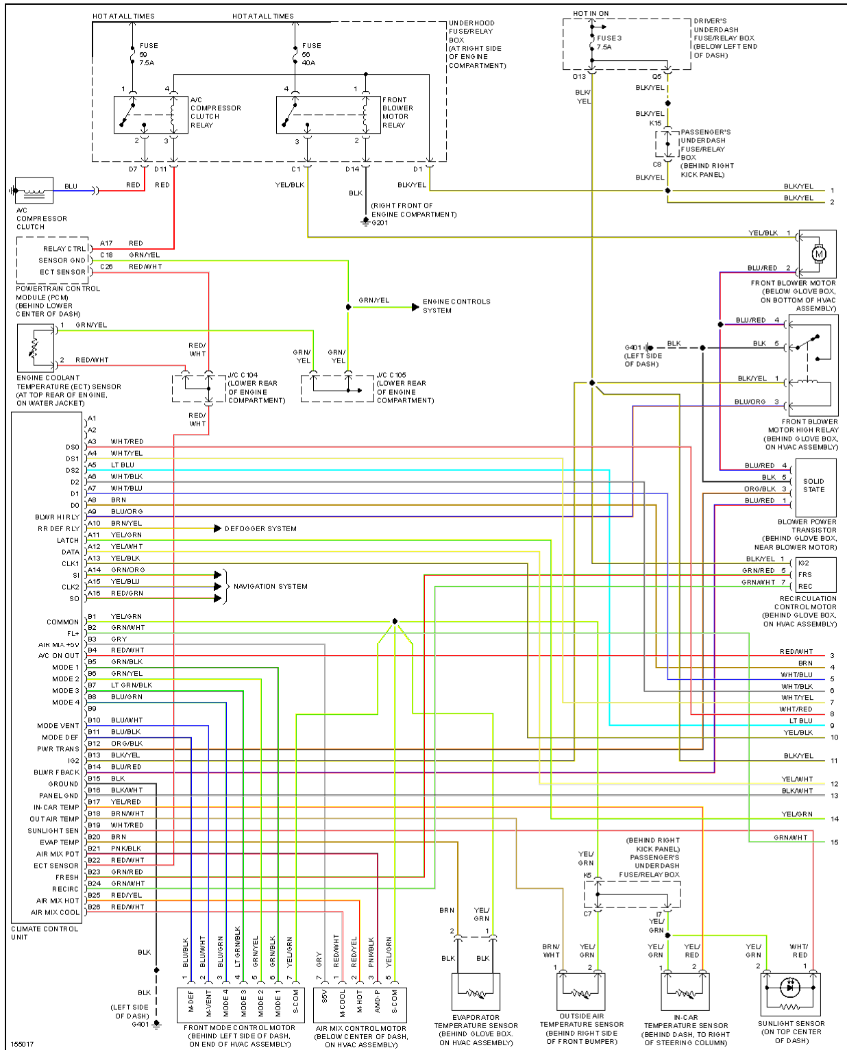
Fig. 1: Automatic A/C Circuit, W/ Navigation (1 of 2)
