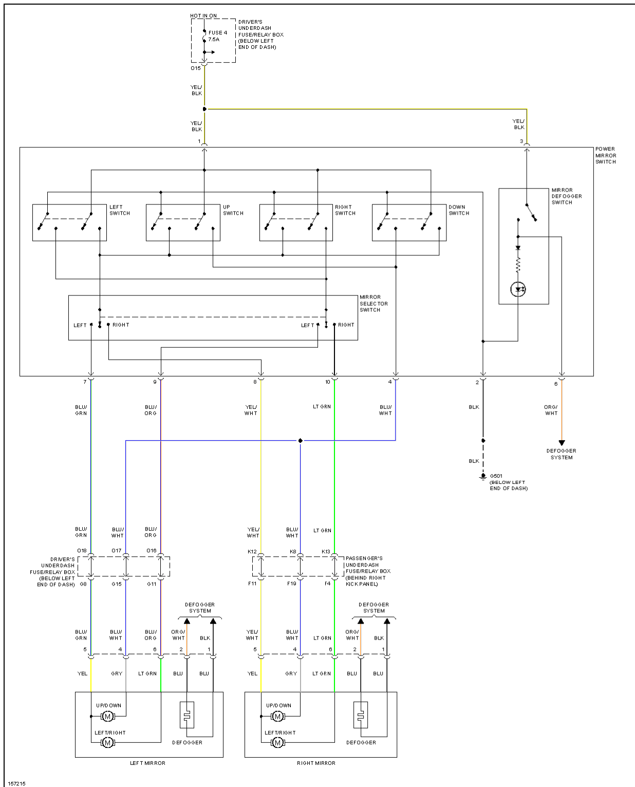
Fig. 58: Power Mirror Circuit, Canada
