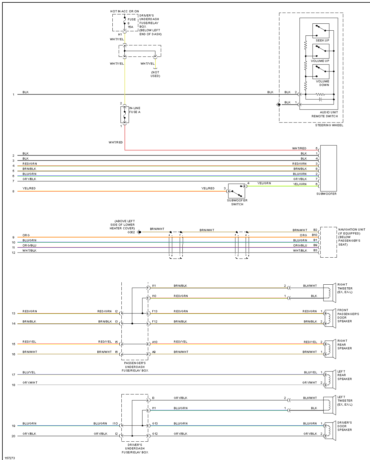
Fig. 69: Radio Circuits, W/ Subwoofer (2 of 2)
