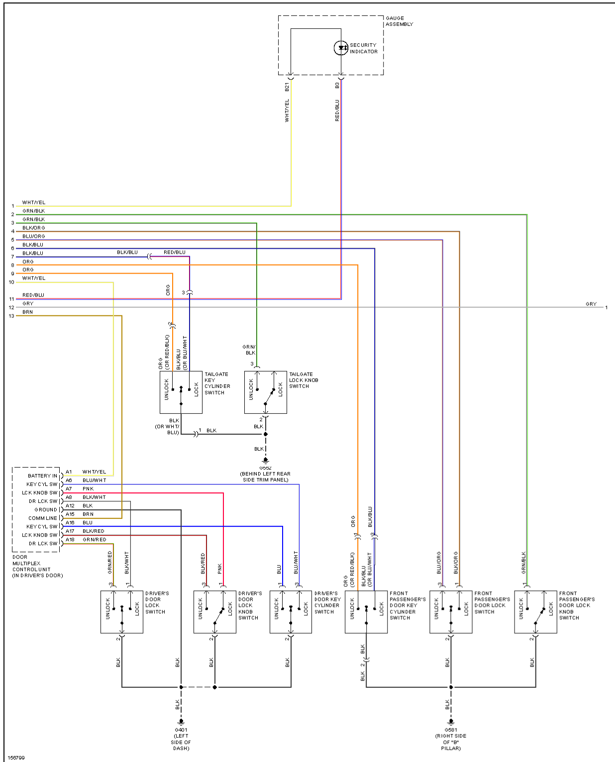
Fig. 52: Power Door Lock Circuit, Except LX (2 of 3)
