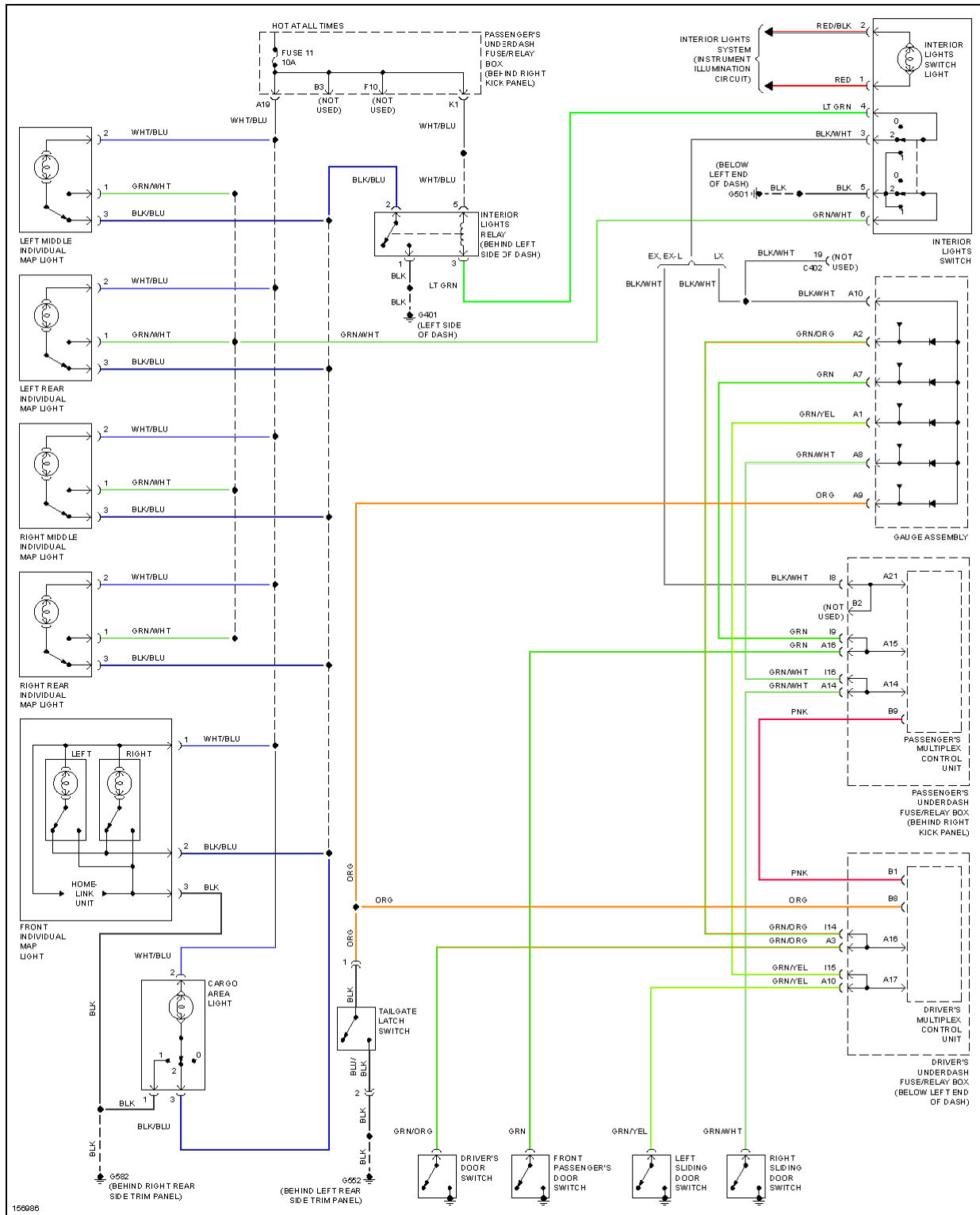
Fig. 42: Courtesy Lamps Circuit
