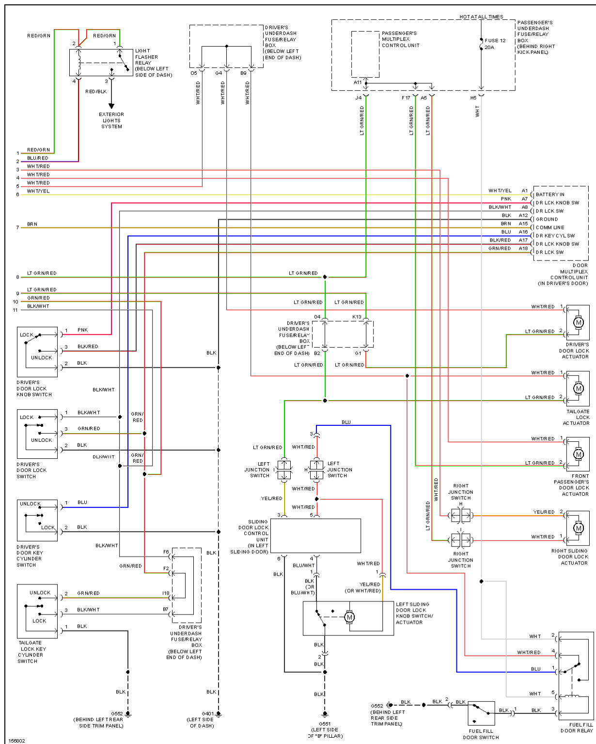
Fig. 14: Anti-theft Circuit, LX (2 of 2)
