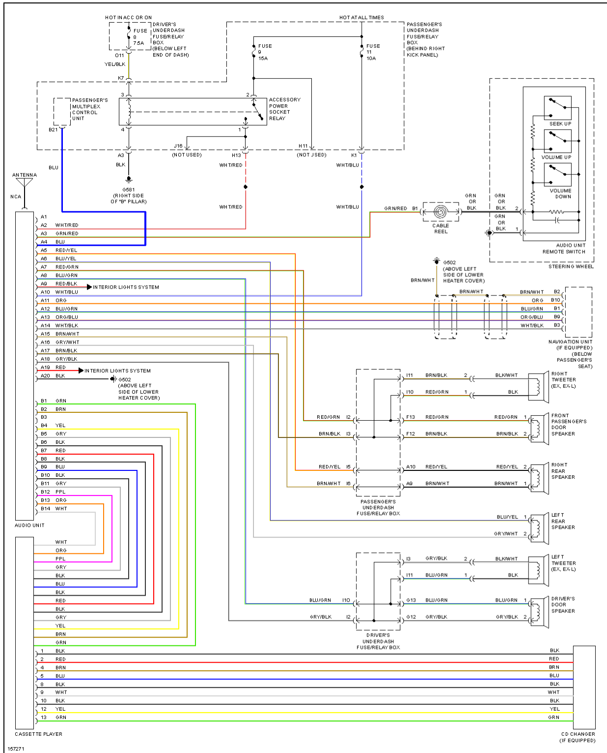
Fig. 65: Radio Circuits, W/ Cassette Deck
