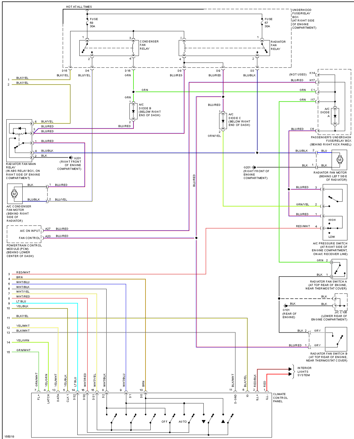
Fig. 2: Automatic A/C Circuit, W/ Navigation (2 of 2)
