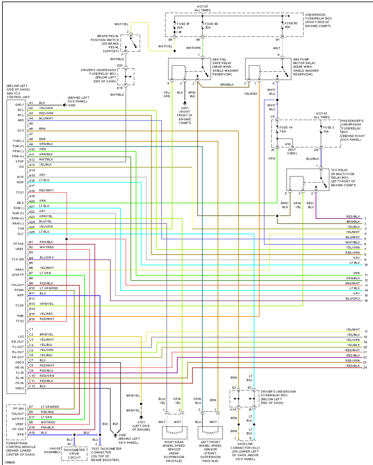
Fig. 8: Anti-lock Brake Circuits (1 of 2)
