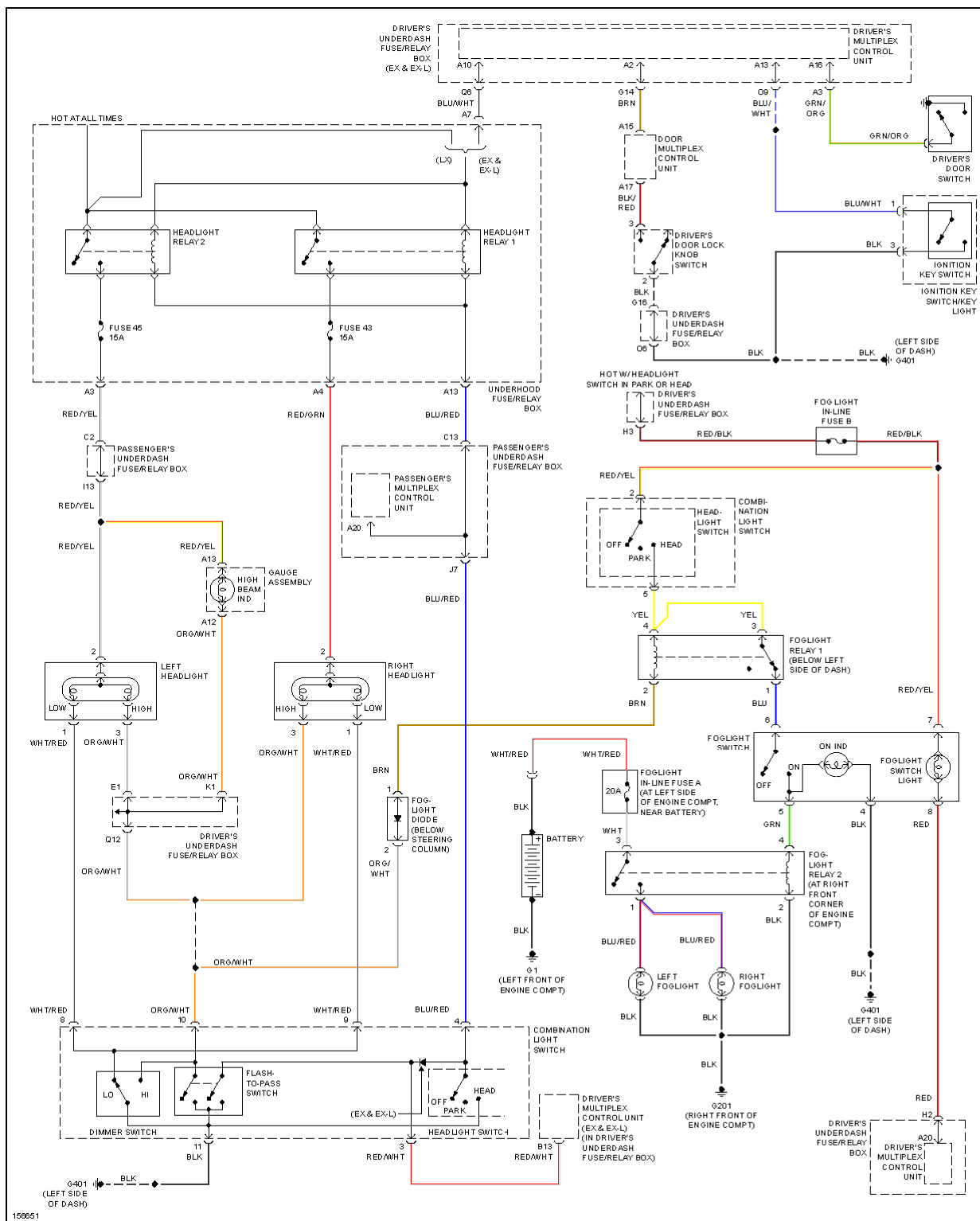
Fig. 38: Headlight Circuit, W/O DRL
