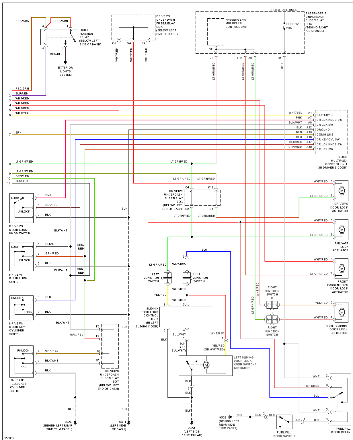
Fig. 55: Power Door Lock Circuit, LX W/ Keyless Entry (2 of 2)
