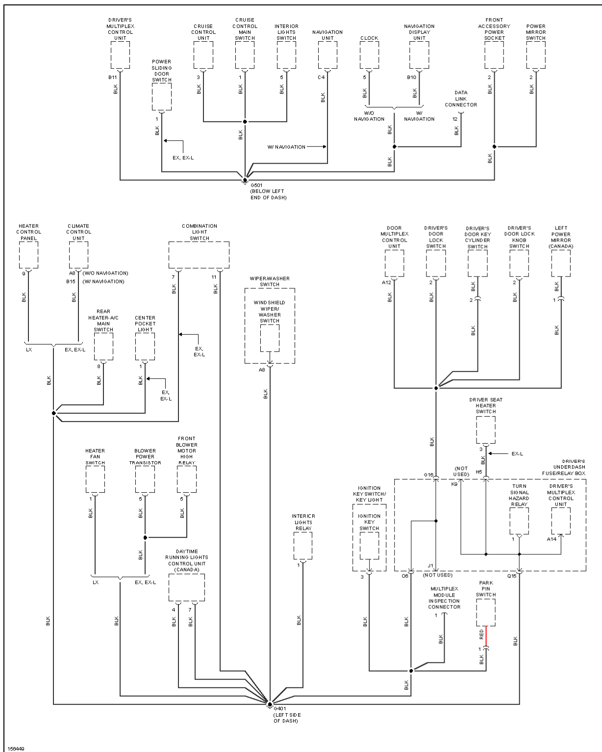
Fig. 34: Ground Distribution Circuit (3 of 4)
