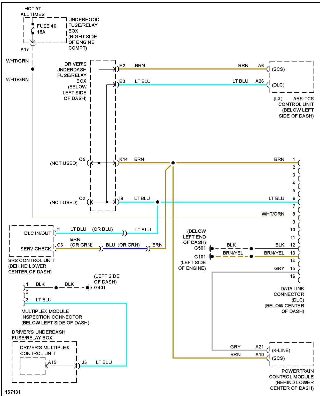
Fig. 18: Computer Data Lines
