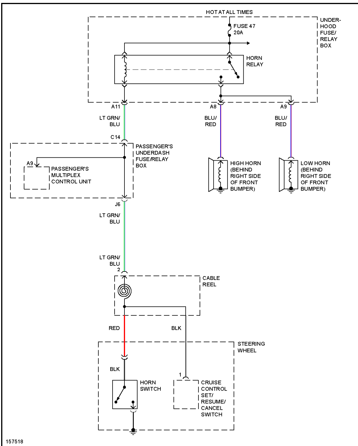
Fig. 39: Horn Circuit
