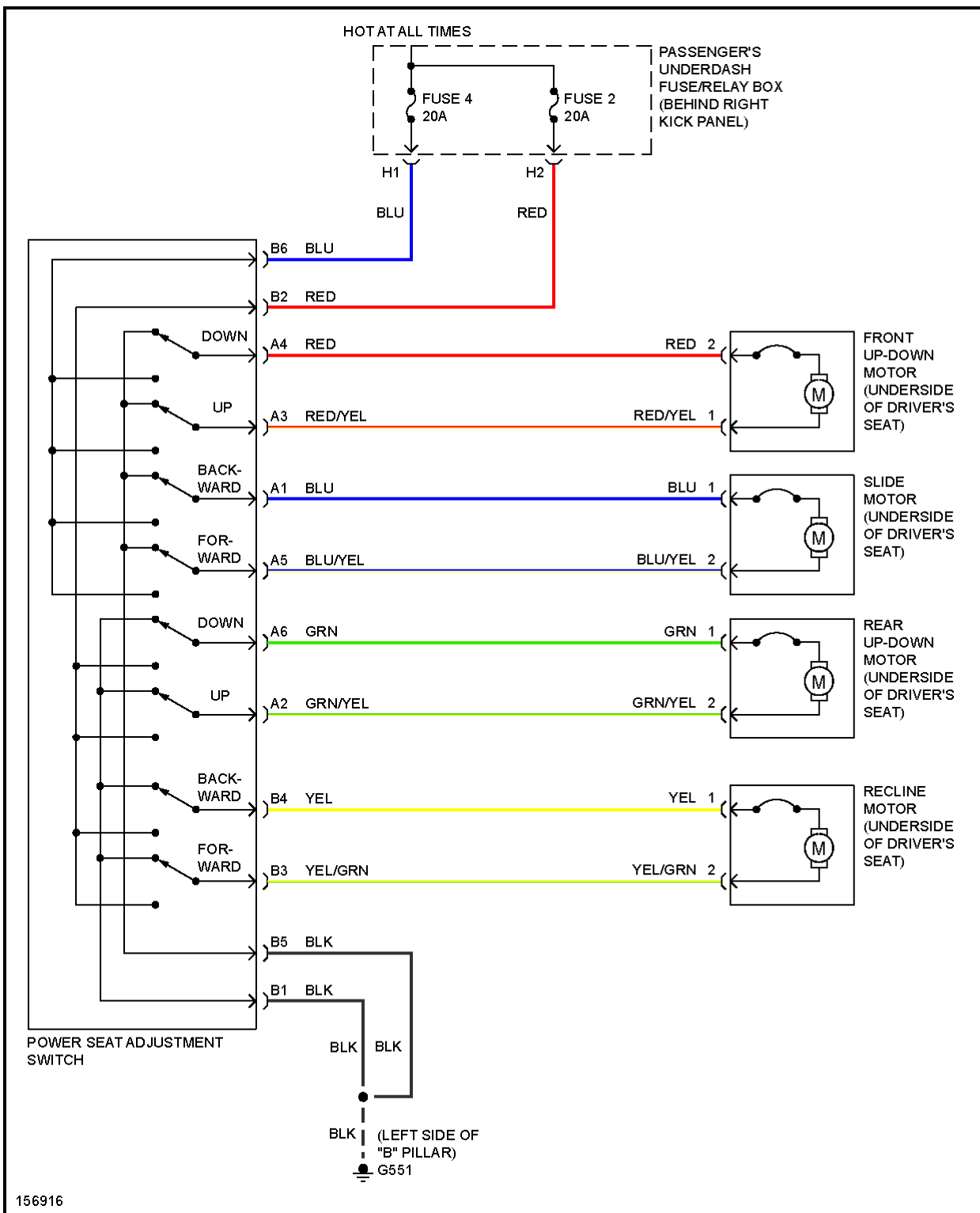
Fig. 61: Power Seat Circuit
