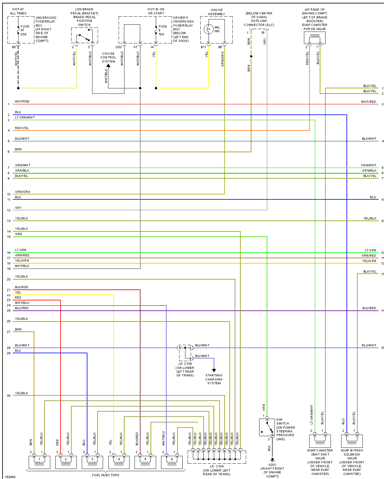
Fig. 24: 3.5L, Engine Performance Circuits (2 of 6)
