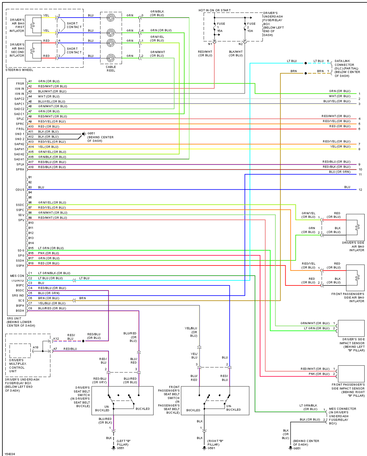
Fig. 73: Supplemental Restraint Circuit (1 of 2)
