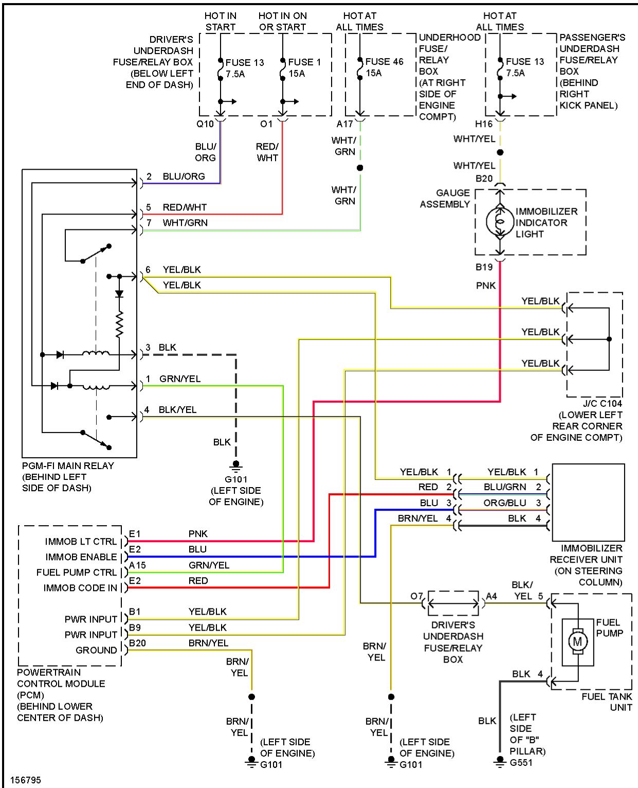
Fig. 15: Immobilizer Circuit
