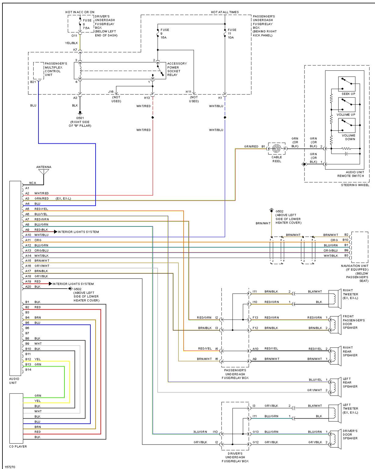
Fig. 64: Radio Circuits, W/ CD
