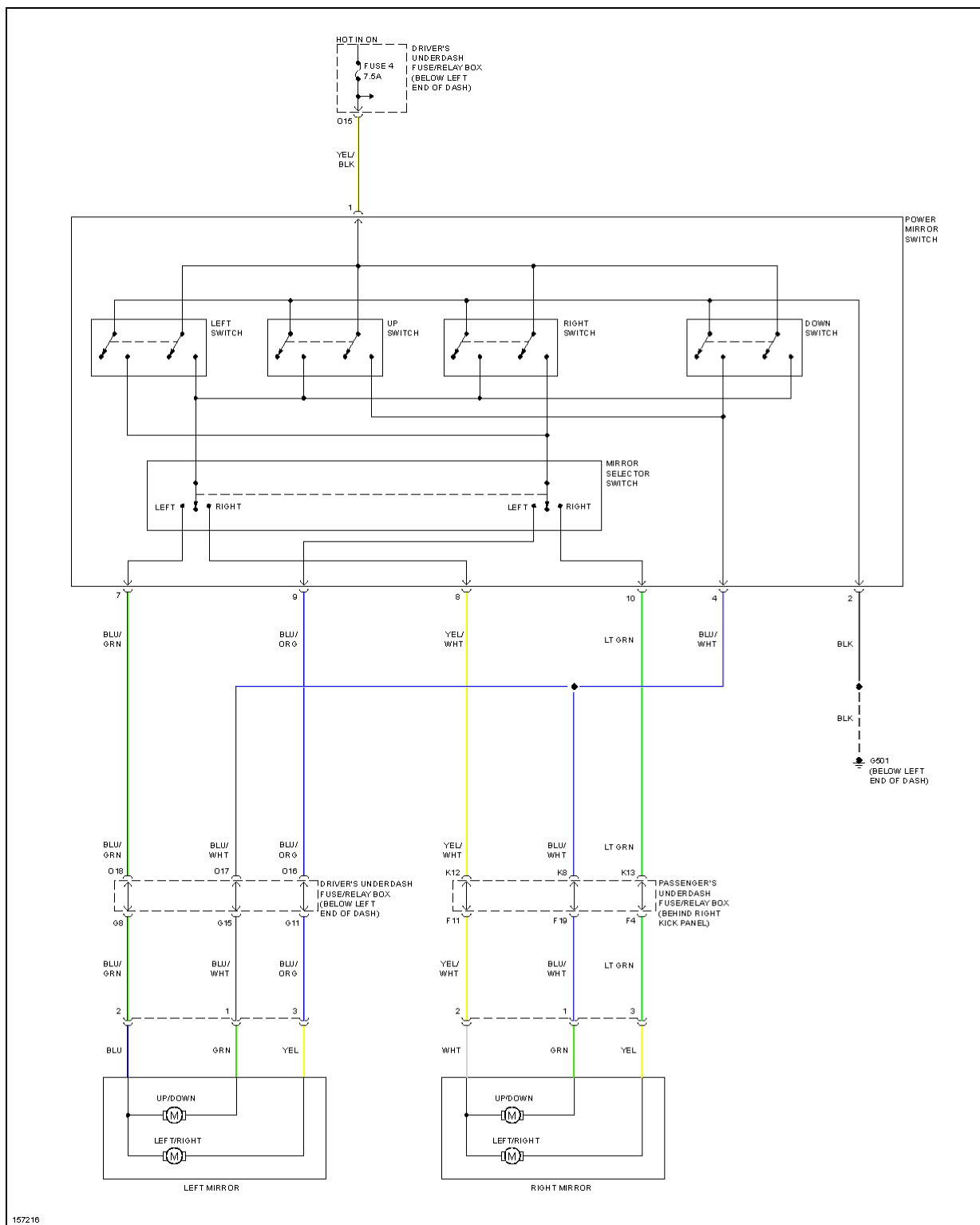
Fig. 59: Power Mirror Circuit, USA
