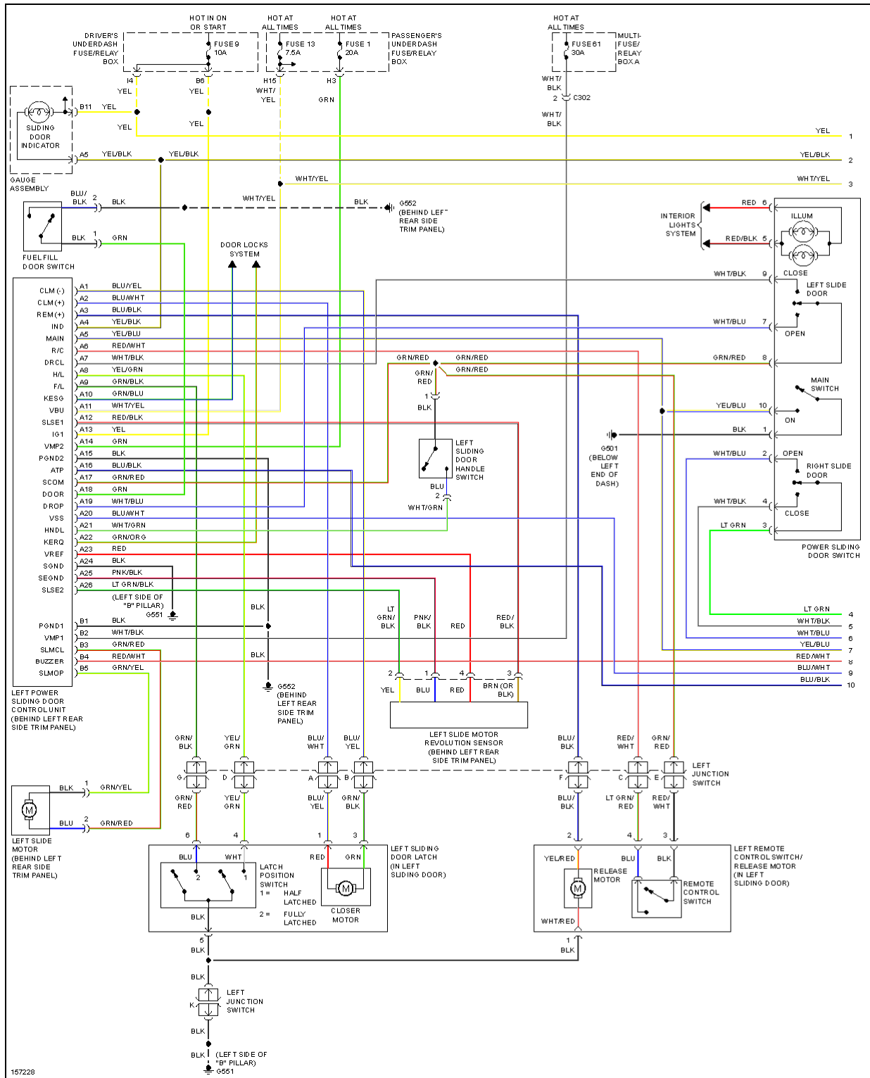
Fig. 77: Power Sliding Door Circuit (1 of 2)
