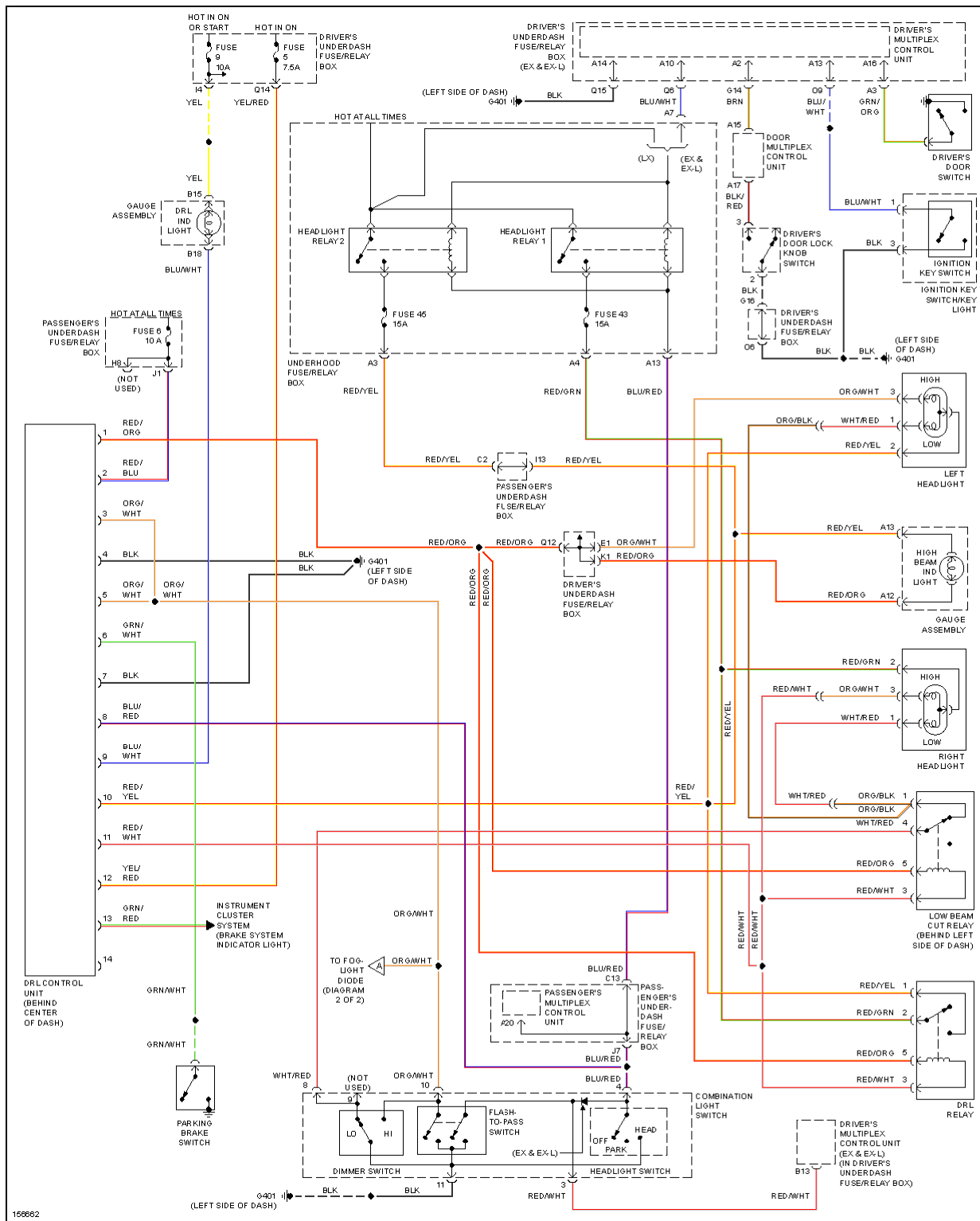
Fig. 36: Headlight Circuit, W/ DRL (1 of 2)
