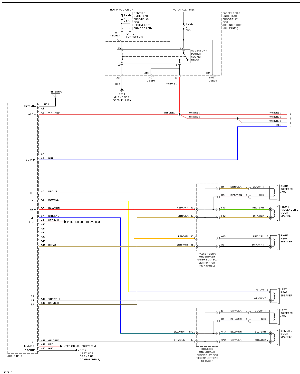
Fig. 66: Radio Circuits, W/ DVD (1 of 2)
