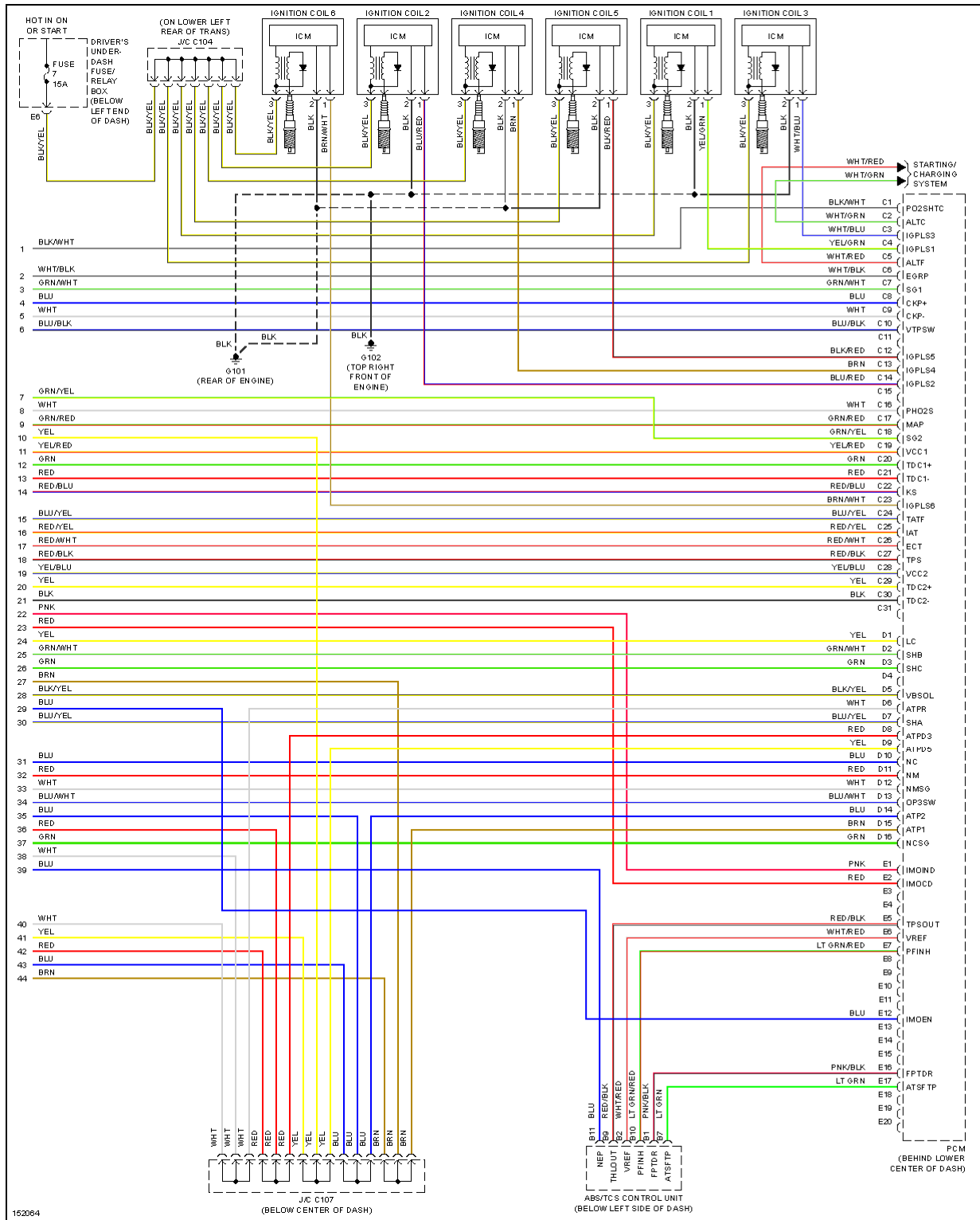
Fig. 28: 3.5L, Engine Performance Circuits (6 of 6)
