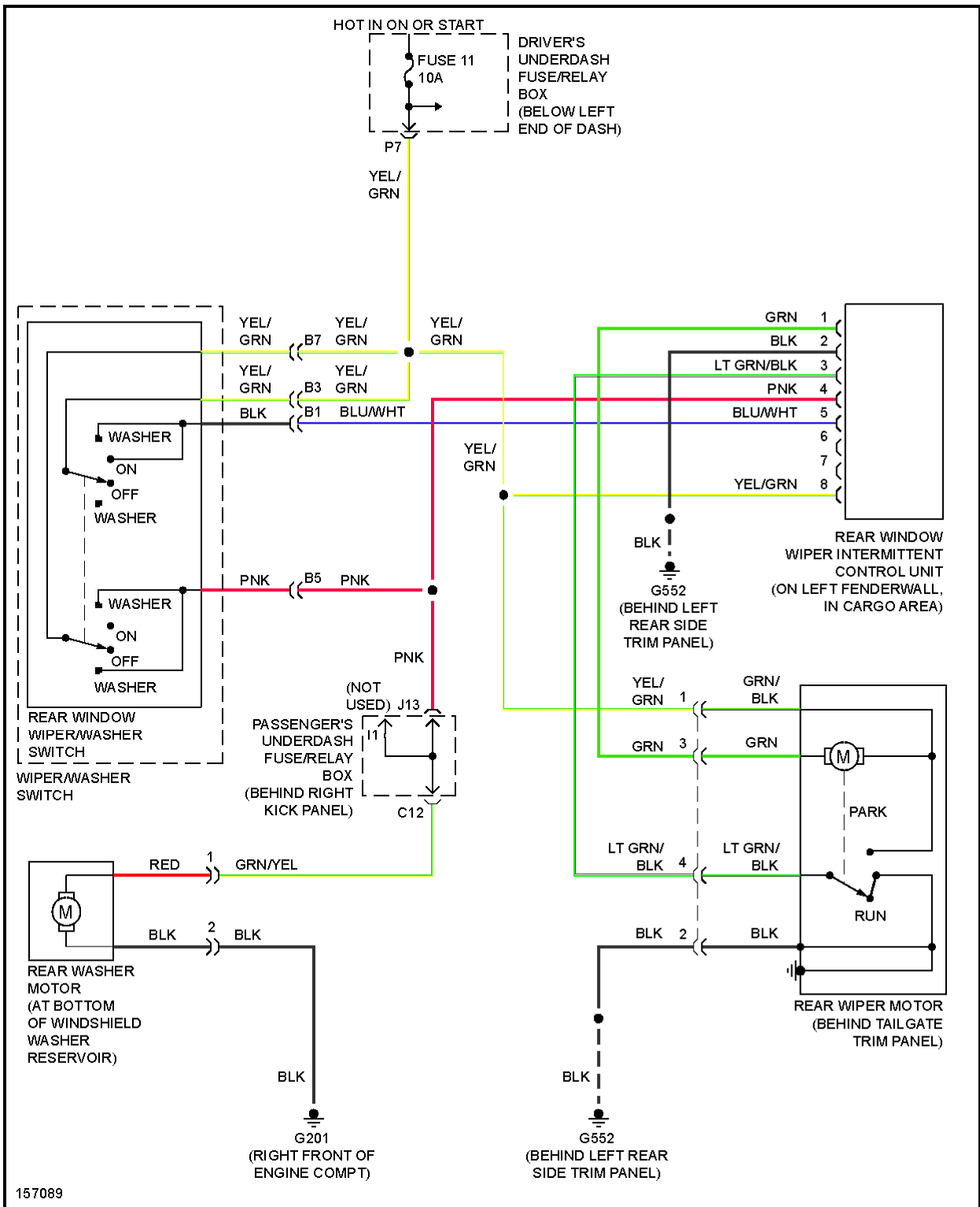
Fig. 81: Rear Washer/Wiper Circuit
