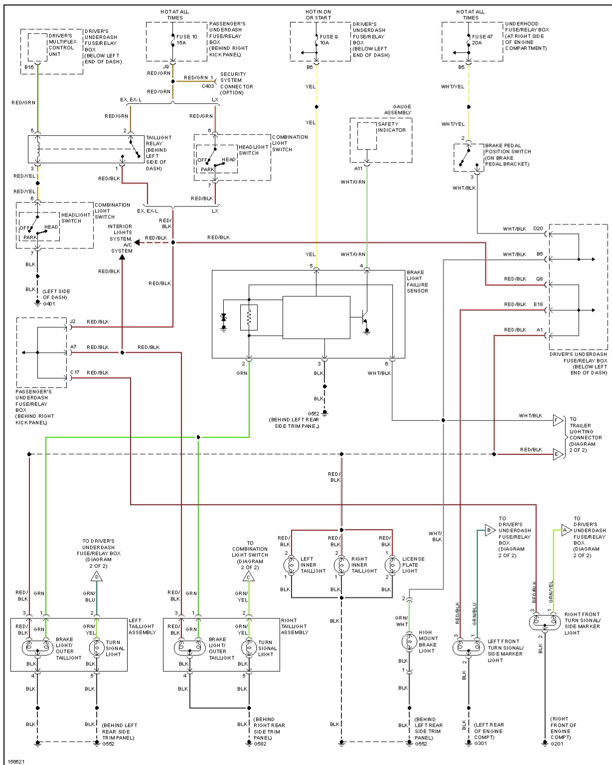
Fig. 30: Exterior Lamps Circuit (1 of 2)
