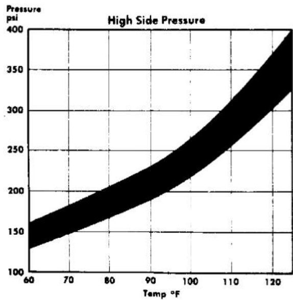
Fig. 1: Ambient Temperature/Pressure (R-12)
