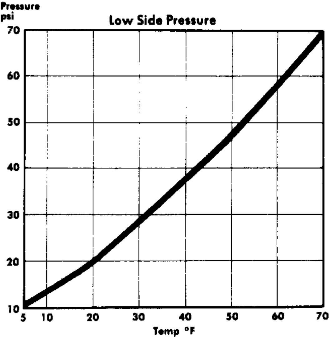
Fig. 2: Evaporator Temperature/Pressure (R-12)
