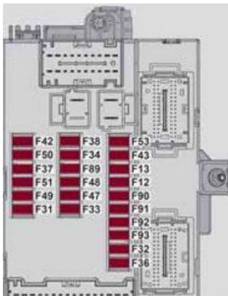
Alfa Romeo Giulietta – fuse box diagram –
