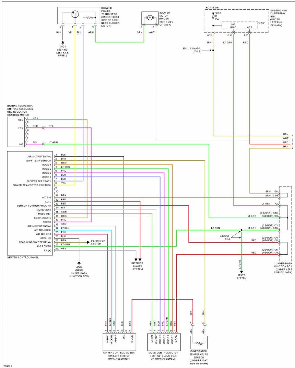
Fig. 3: Manual A/C Circuit, Except Hybrid (1 of 2)
