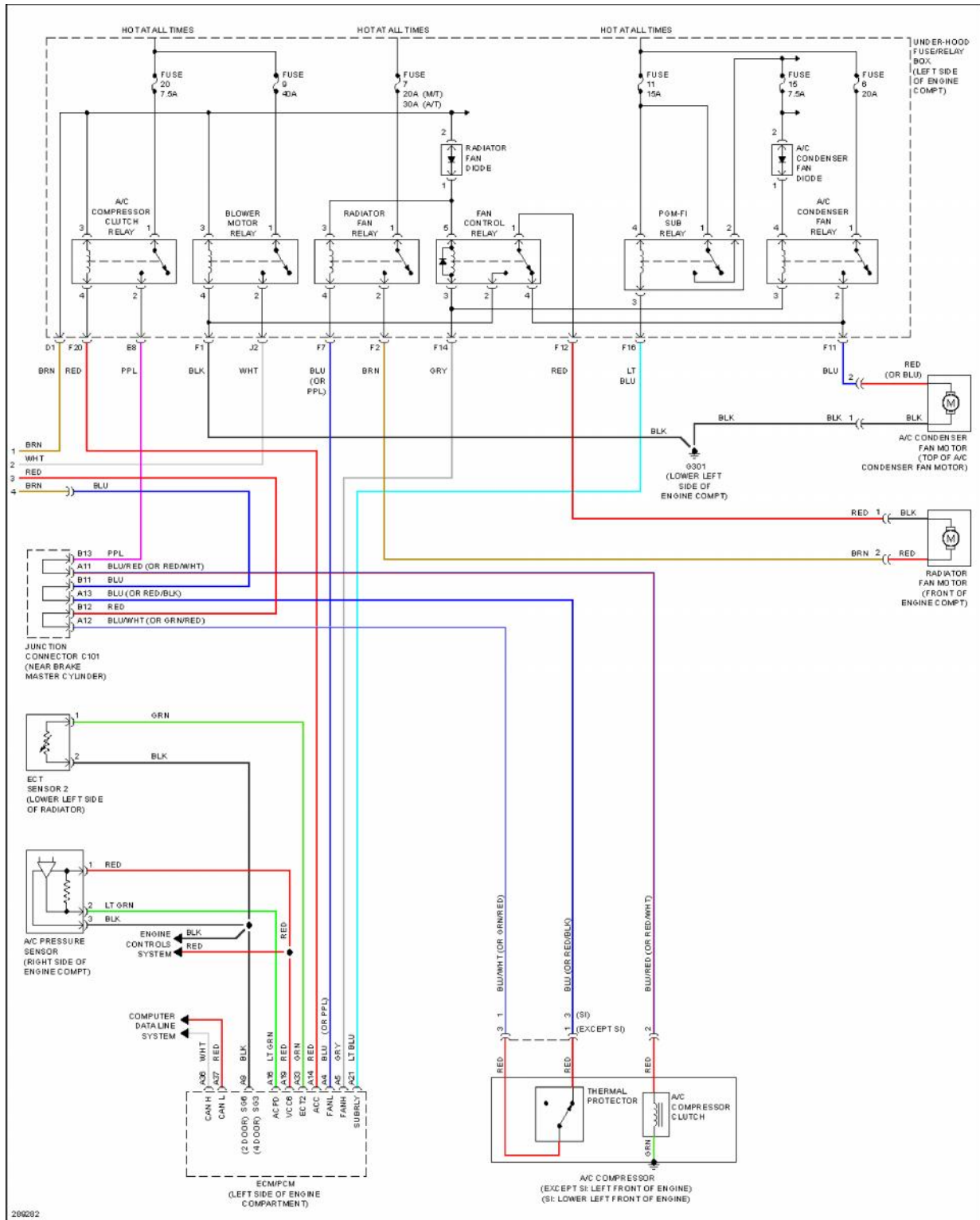
Fig. 4: Manual A/C Circuit, Except Hybrid (2 of 2)
