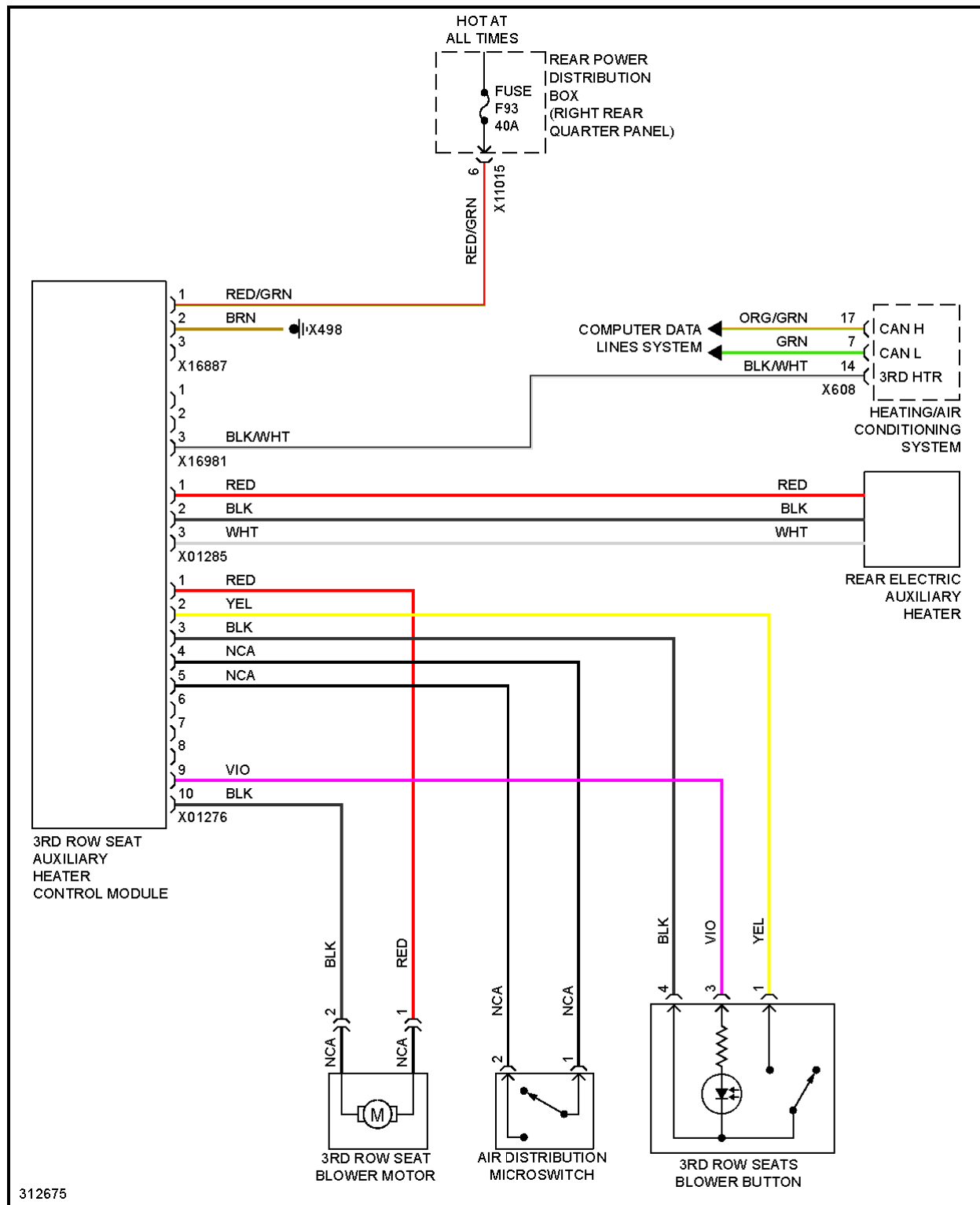
Fig. 1: 3rd Row Seat Heater Circuit
