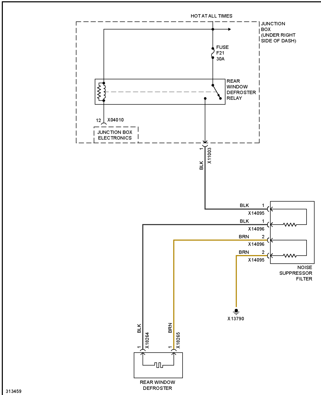
Fig. 26: Rear Defogger Circuit
