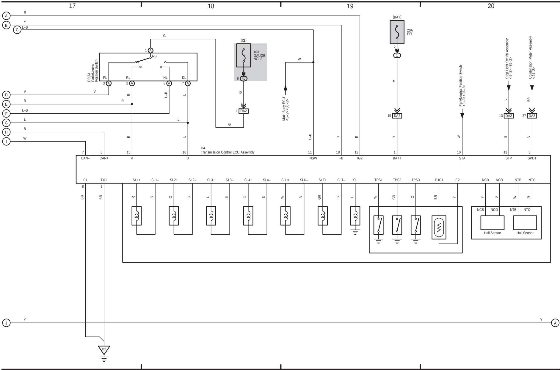
ECT and A/T Indicator (2GR-FE)
