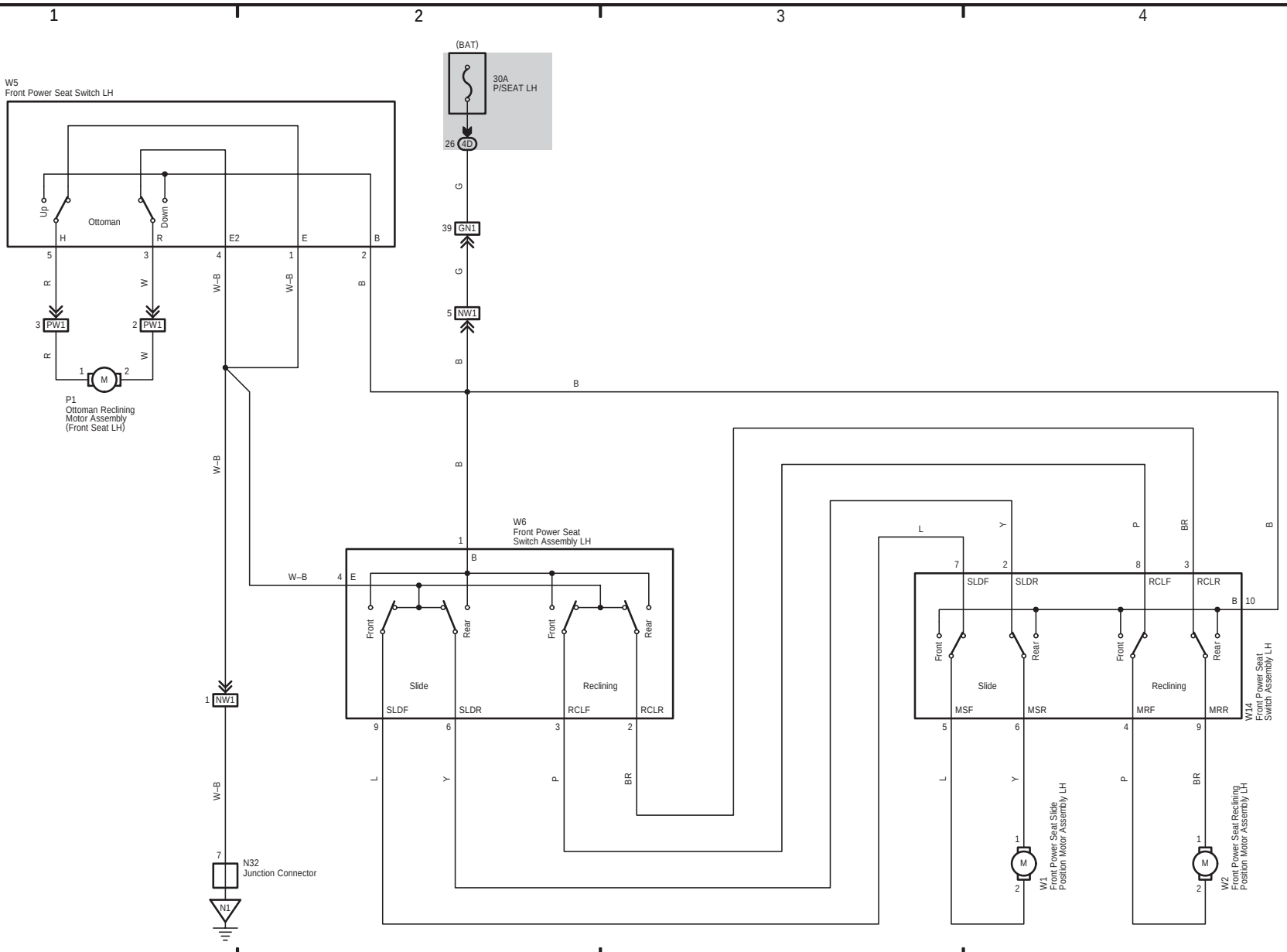
Power Seat (RHD Front Passenger' s Seat) (From Oct. 2011 Production)
