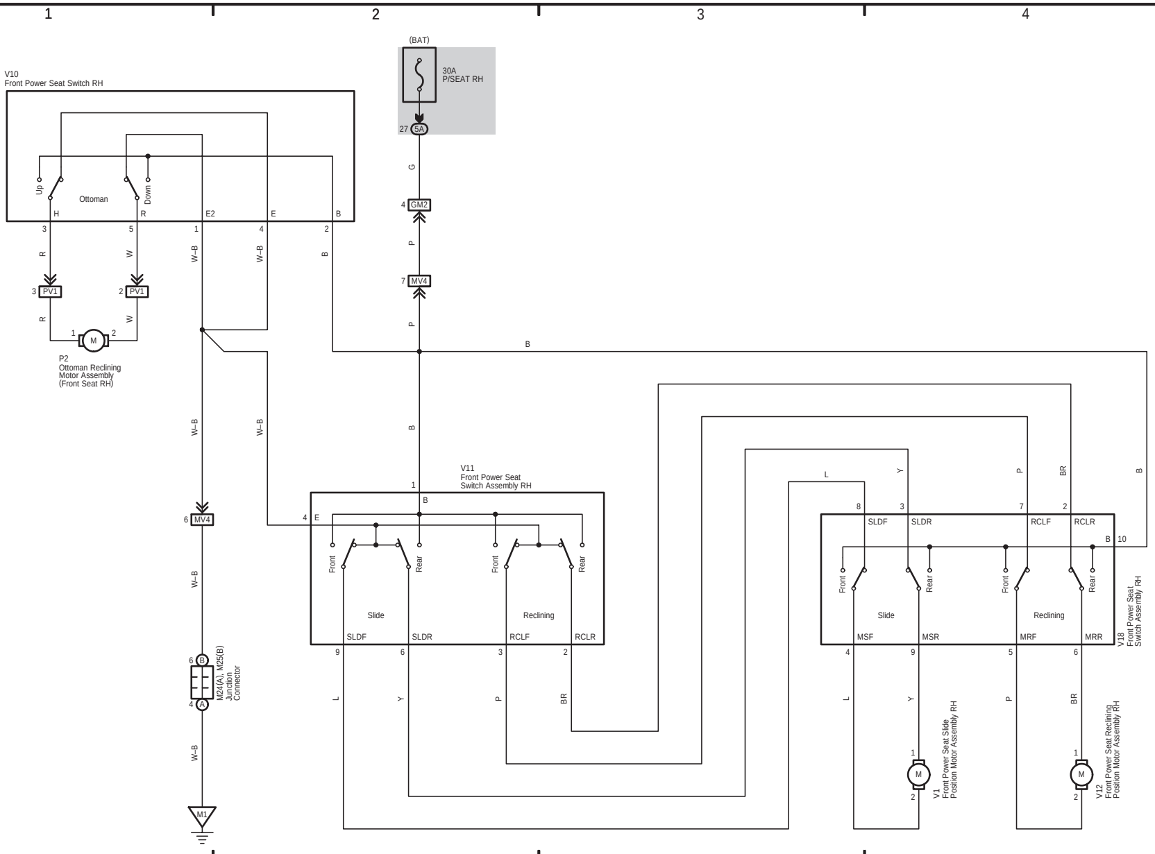
Power Seat (LHD Front Passenger' s Seat) (From Oct. 2011 Production)
