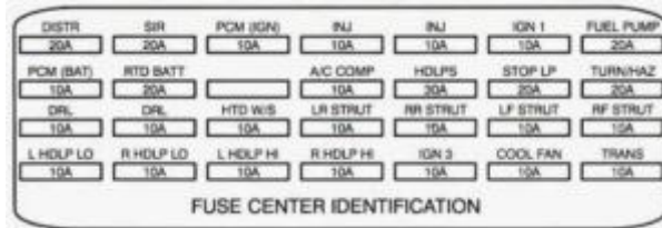
Cadillac DeVille – fuse box diagram – engine
