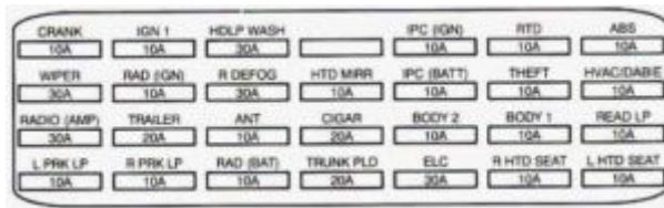
Cadillac DeVille – fuse box diagram – trunk
