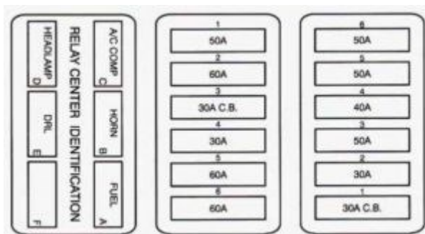
Cadillac DeVille – fuse box diagram – maxi fuse block
