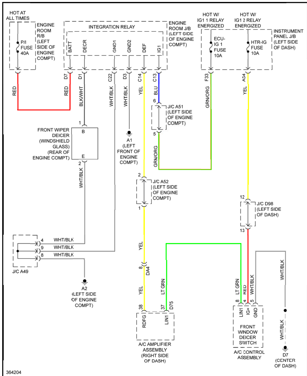
Fig. 26: Front Deicer Circuit
