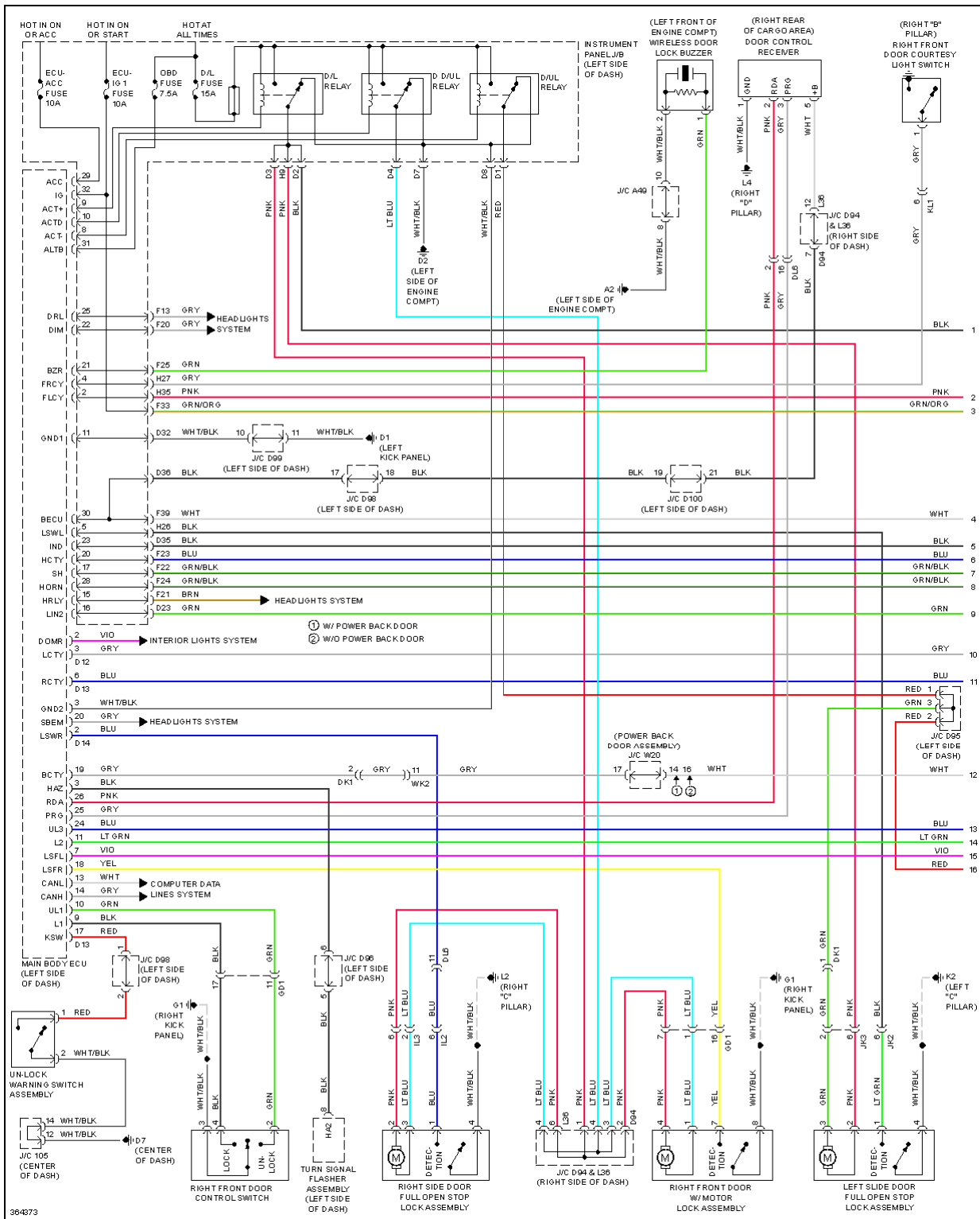
Fig. 9: Forced Entry Circuit, W/O Smart Key System (1 of 2)
