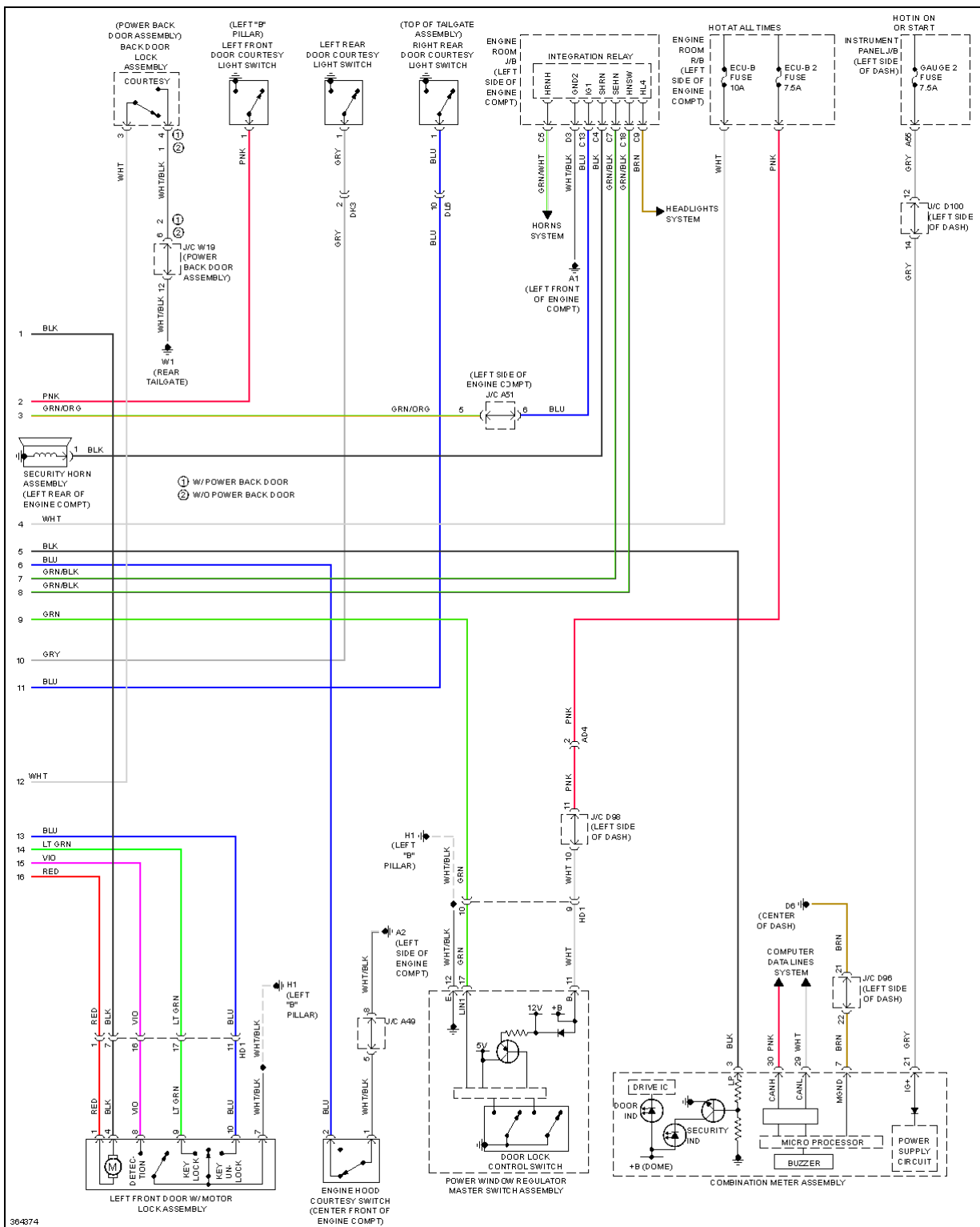
Fig. 10: Forced Entry Circuit, W/O Smart Key System (2 of 2)
