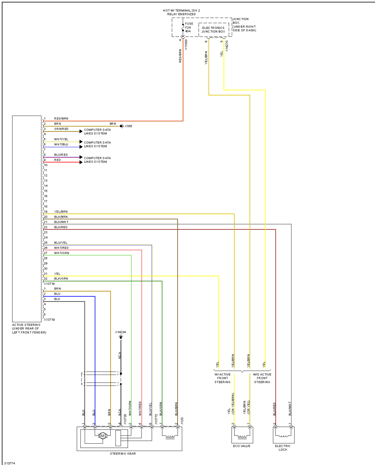
Fig. 28: Electronic Power Steering Circuit, W/O AL Active Steering
