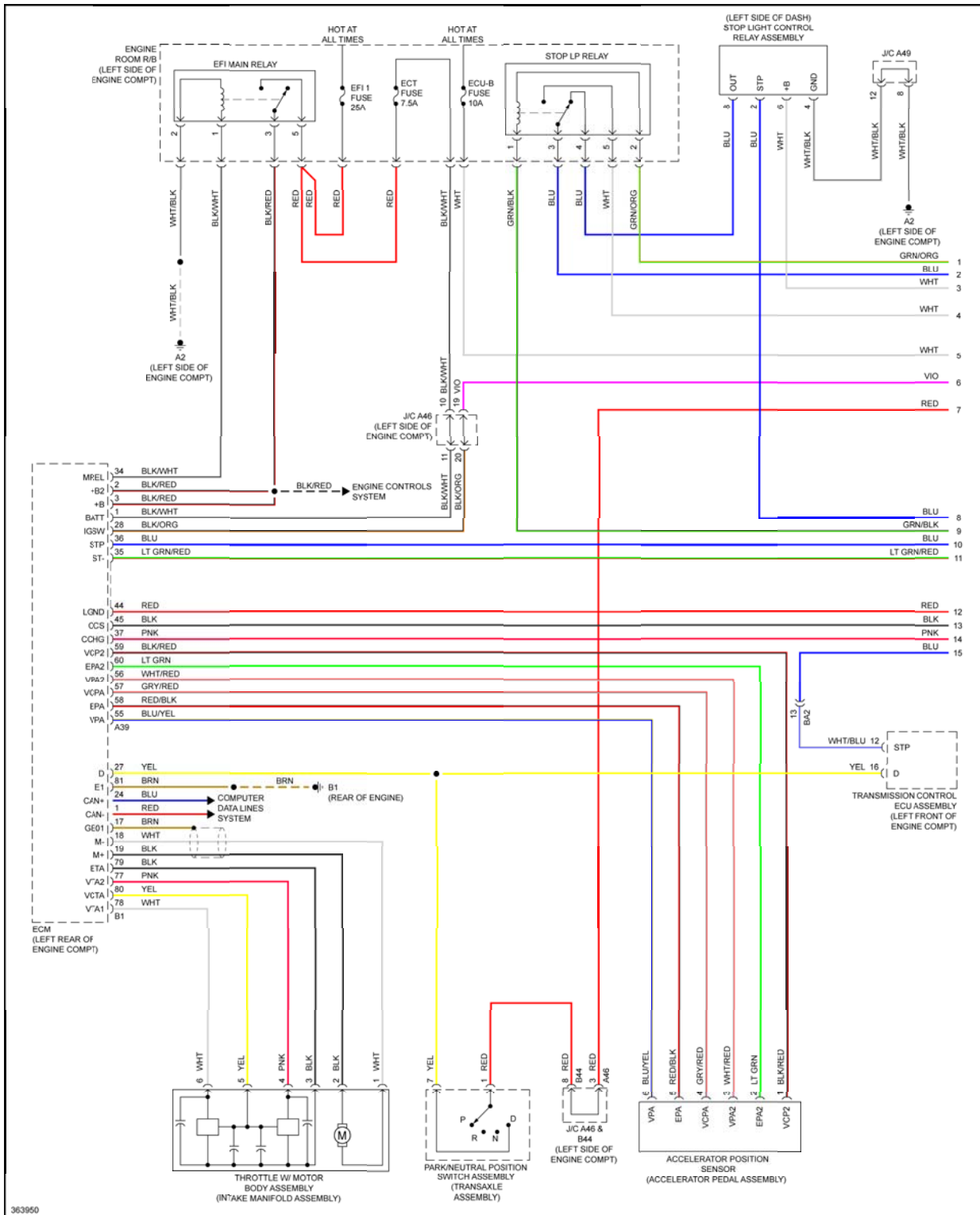
Fig. 23: 3.5L, Dynamic Laser Cruise Control Circuit (1 of 3)
