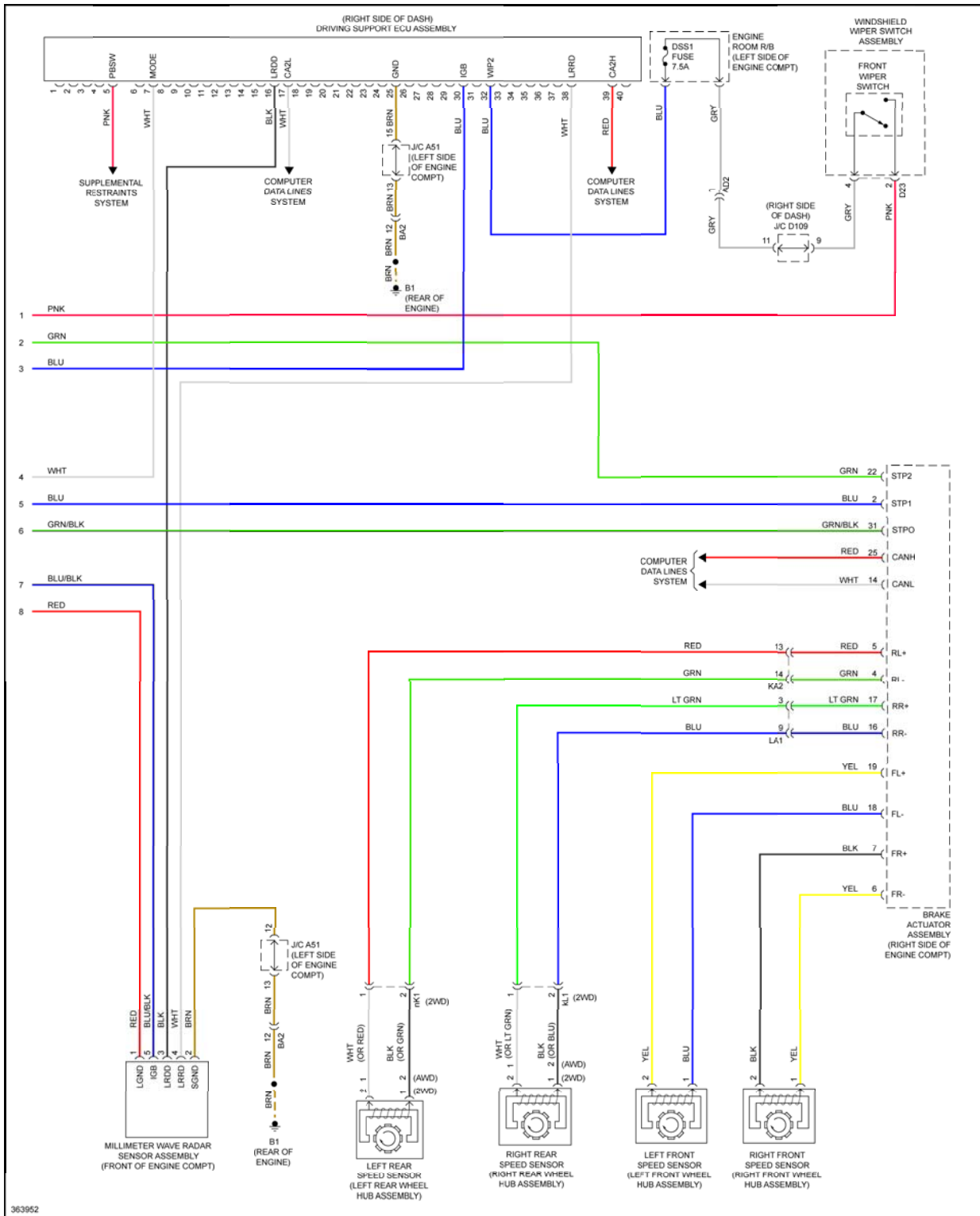
Fig. 25: 3.5L, Dynamic Laser Cruise Control Circuit (3 of 3)
