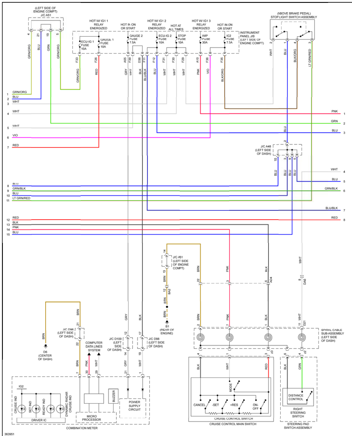
Fig. 24: 3.5L, Dynamic Laser Cruise Control Circuit (2 of 3)
