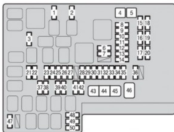
Scion FR-S – fuse box – engine compartment
