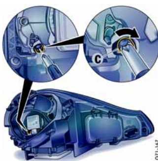
Xenon headlight
