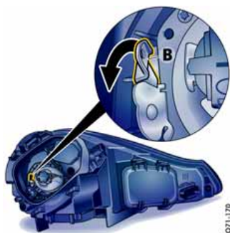
Halogen headlights
