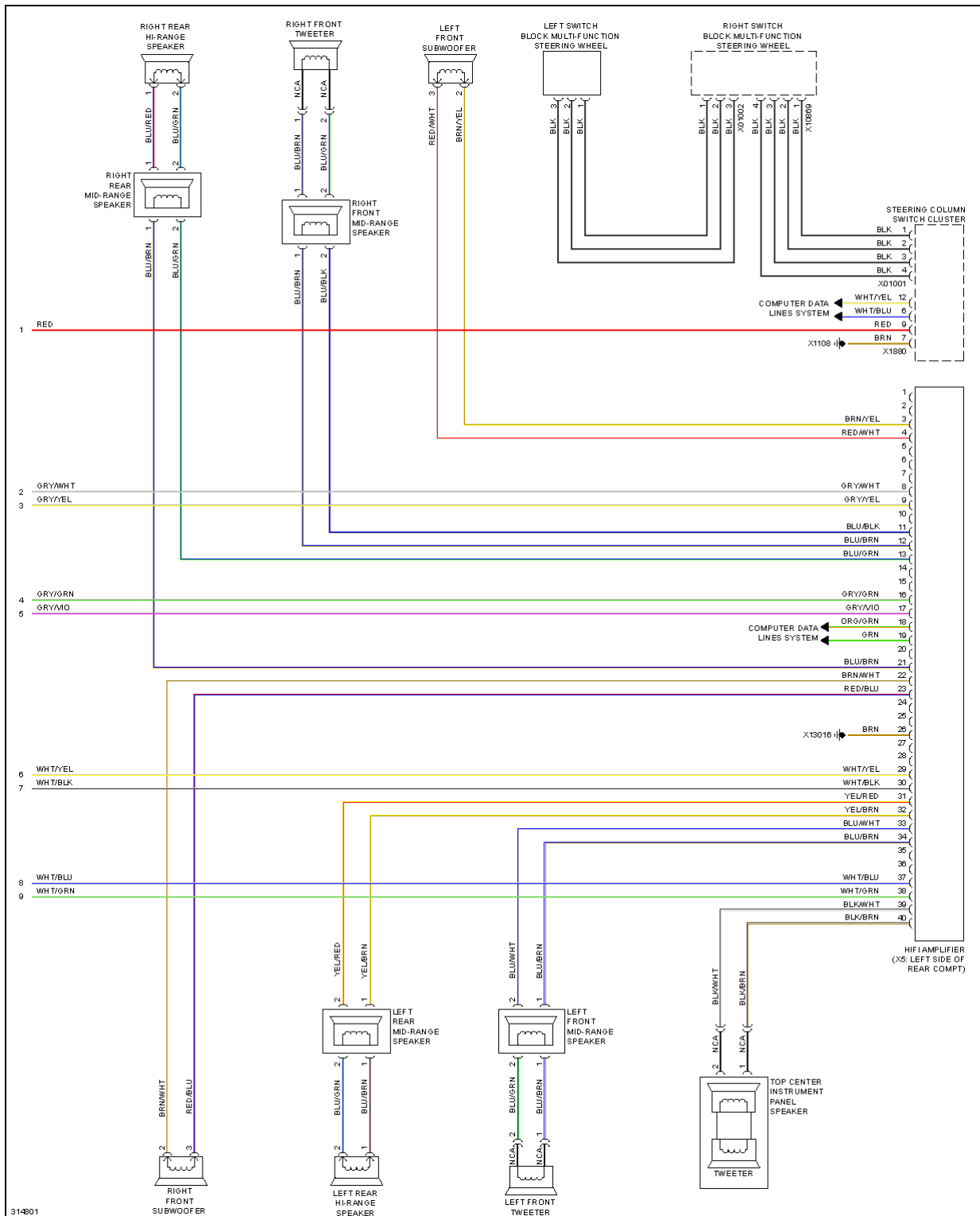
Fig. 108: Radio Circuit, W/ CIC & HIFI Radio (2 of 2)
