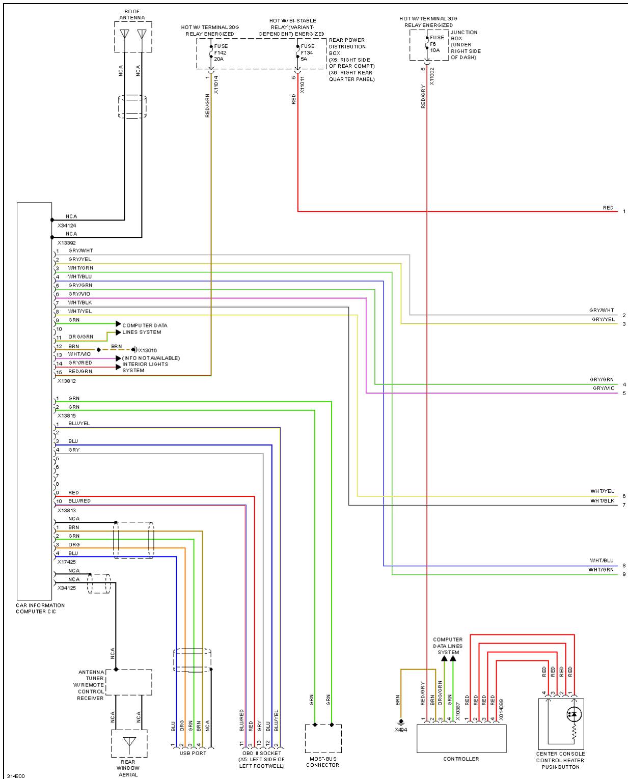
Fig. 107: Radio Circuit, W/ CIC & HIFI Radio (1 of 2)
