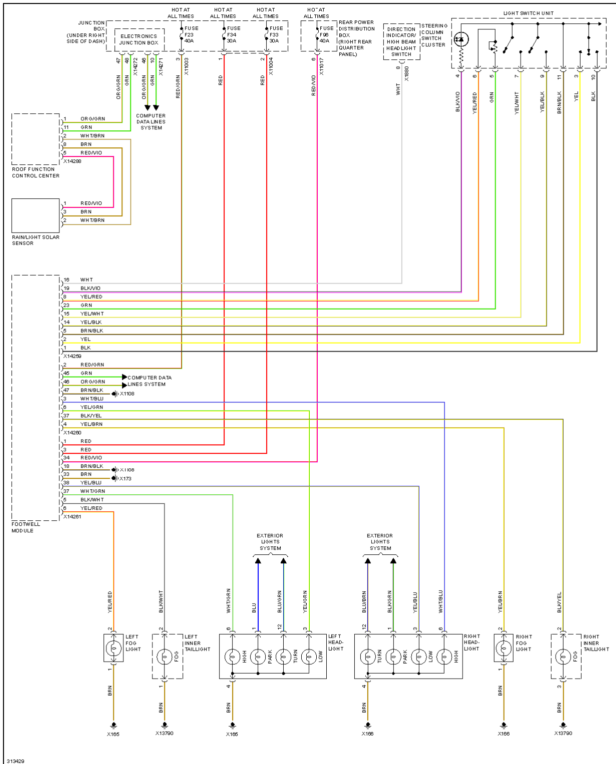
Fig. 54: Headlamps Circuit, W/O Xenon Lamps
