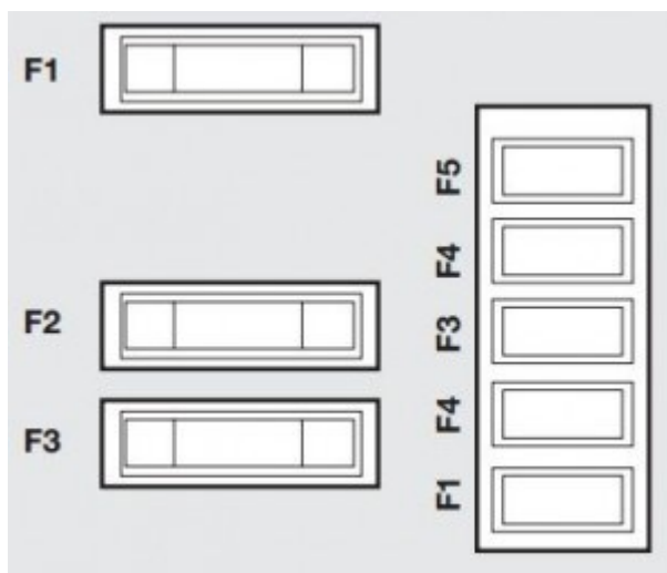
Fiat Scudo mk2 – fuse box – engine compartment
