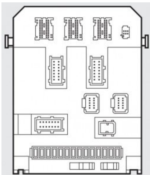
Fiat Scudo mk2 – fuse box – passenger compartment
