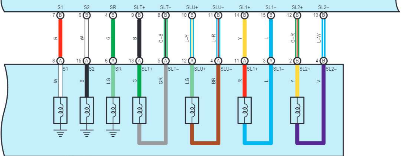
C39(A), C40(B) Electronically Controlled Transmission Solenoid
