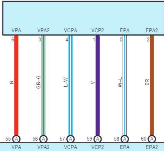
A38(A), C53(B) ECM
