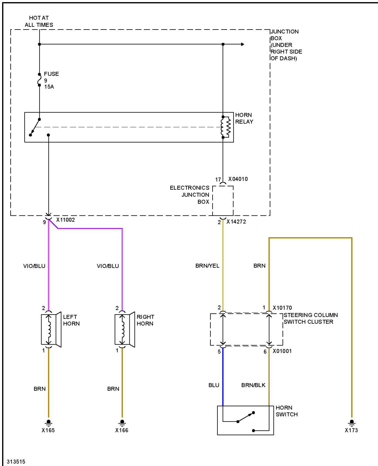
Fig. 55: Horn Circuit
