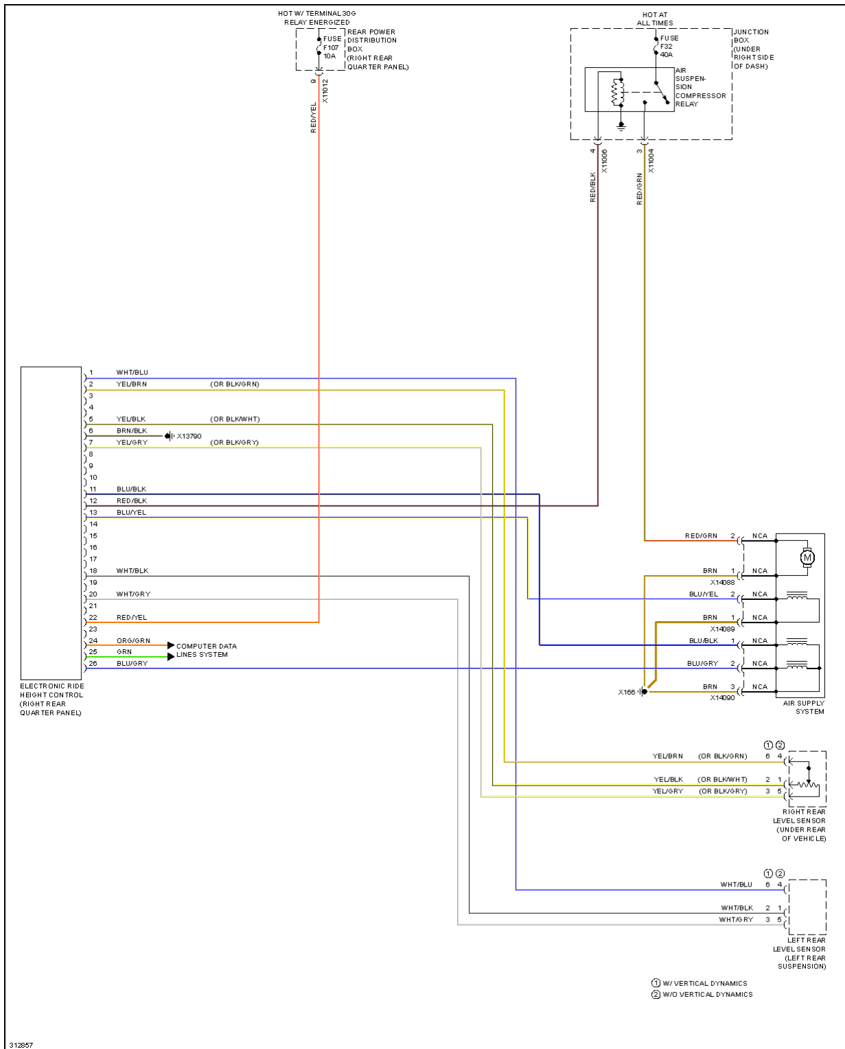
Fig. 29: Air Suspension Circuit
