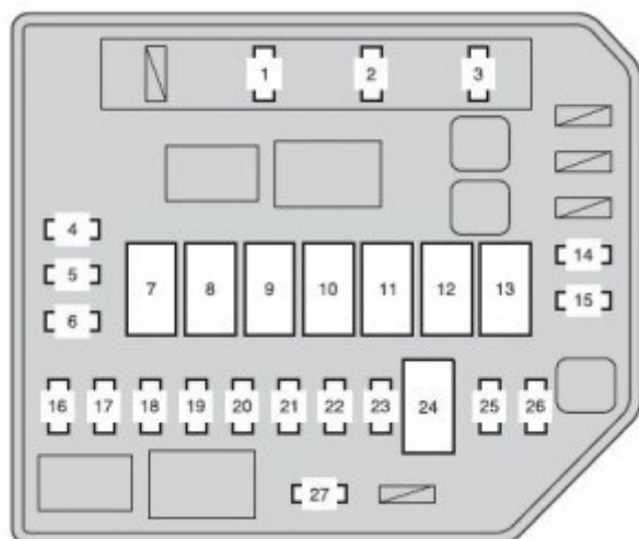
Scion xD – fuse box – engine compartment
