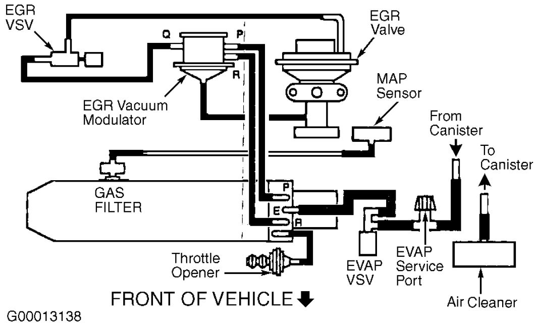
Fig. 7: Vacuum Diagram (Camry 4-Cyl. & Camry Solara 4-Cyl. - 1 Of 3) Courtesy of TOYOTA MOTOR SALES, U.S.A., INC.
