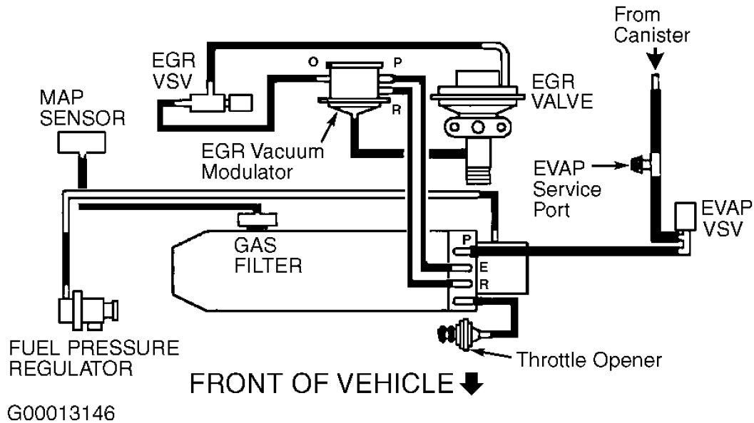
Fig. 10: Vacuum Diagram (Celica - 1 Of 3)
