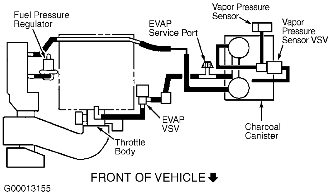
Fig. 16: Vacuum Diagram (Land Cruiser - 1 Of 3) Courtesy of TOYOTA MOTOR SALES, U.S.A., INC.
