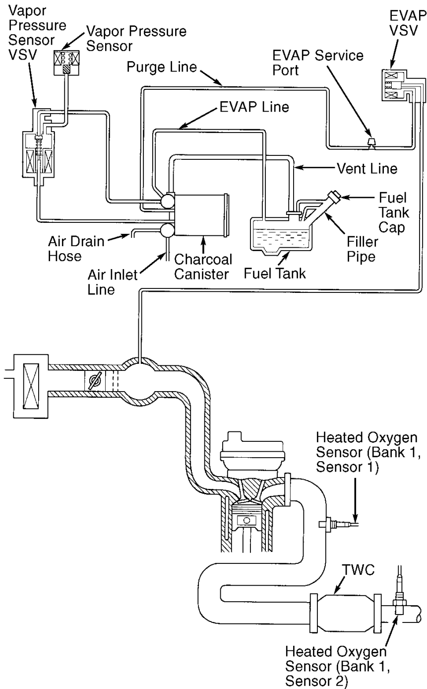
Fig. 15: Vacuum Diagram (Corolla - 3 Of 3) Courtesy of TOYOTA MOTOR SALES, U.S.A., INC.
