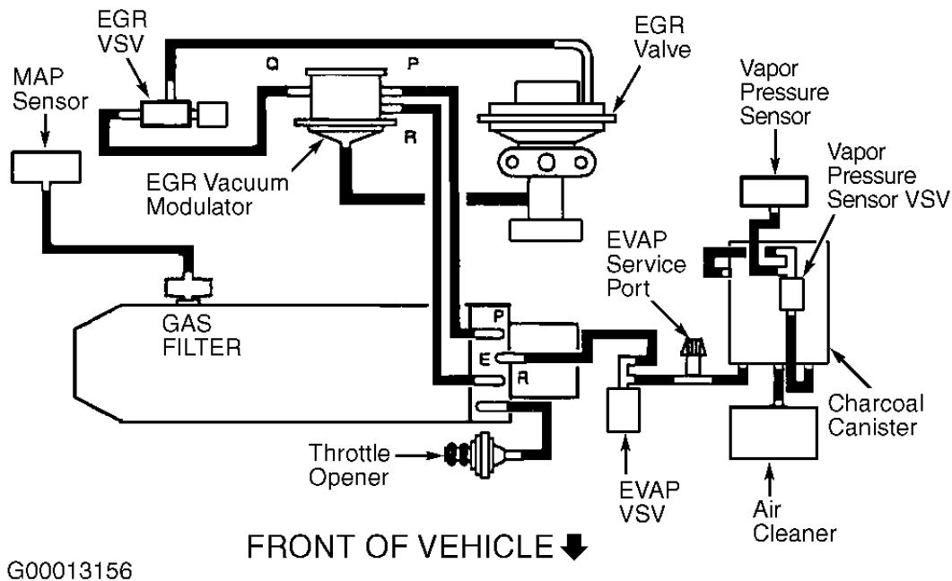
Fig. 19: Vacuum Diagram (RAV4 - 1 Of 3) Courtesy of TOYOTA MOTOR SALES, U.S.A., INC.
