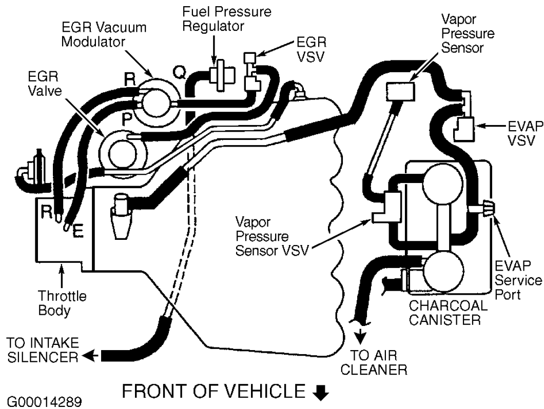
Fig. 27: Vacuum Diagram (Tacoma V6 Except Prerunner) Courtesy of TOYOTA MOTOR SALES, U.S.A., INC.
