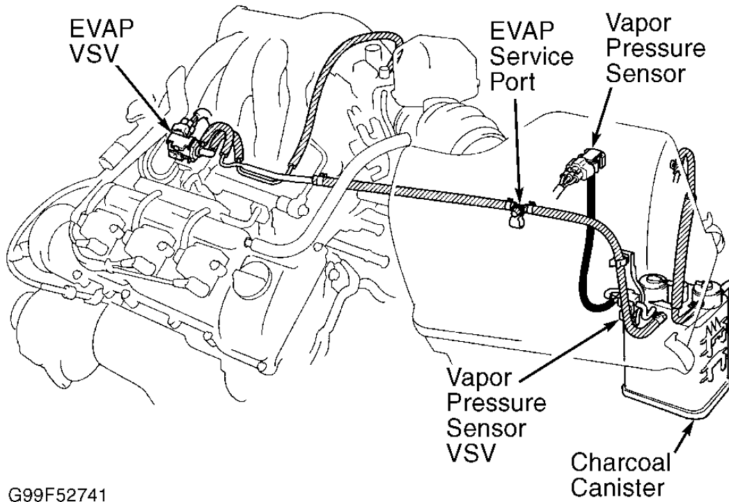
Fig. 23: Vacuum Diagram (Sienna - 2 Of 3) Courtesy of TOYOTA MOTOR SALES, U.S.A., INC.
