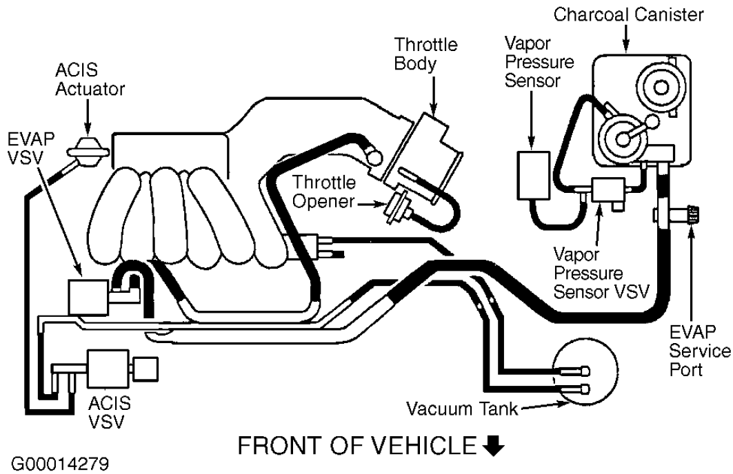
Fig. 22: Vacuum Diagram (Sienna - 1 Of 3) Courtesy of TOYOTA MOTOR SALES, U.S.A., INC.
