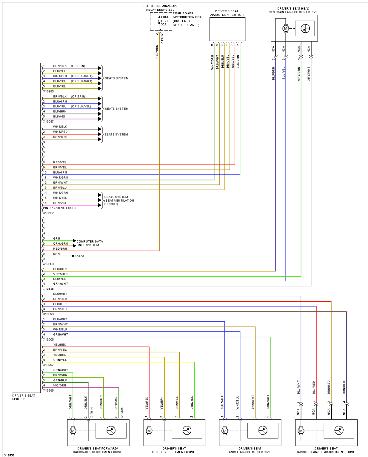
Fig. 61: Driver's Memory Seat Circuit, W/O Lumbar Support
