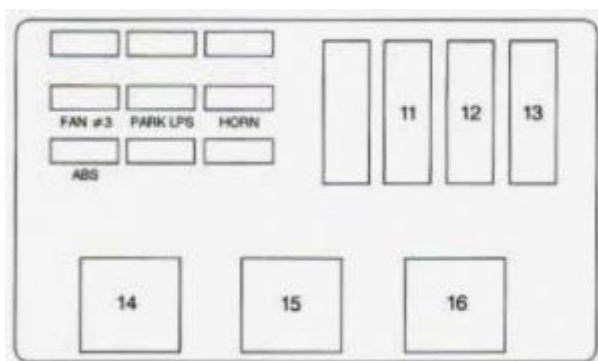
Chevrolet Monte Carlo – fuse box – underhood
