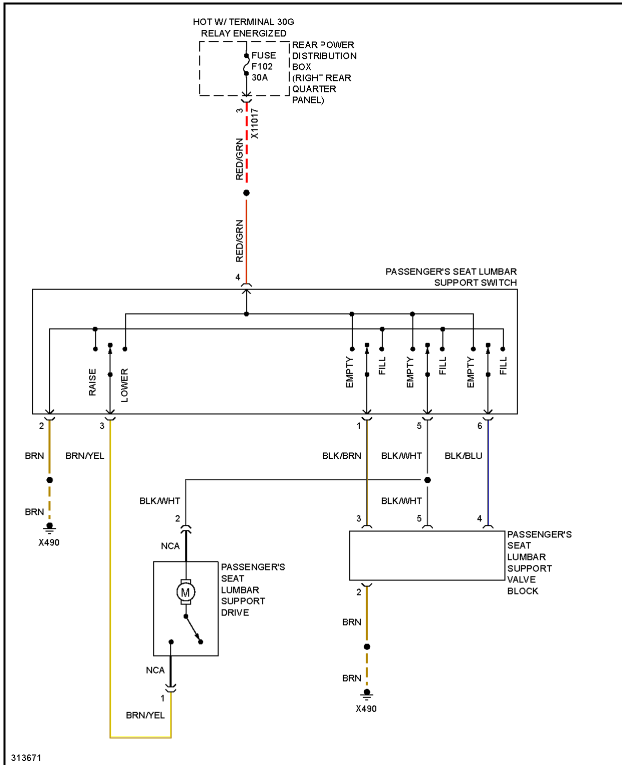
Fig. 94: Passenger's Lumbar Circuit
