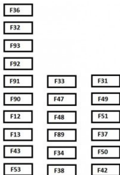
Fiat Ducato BASE CAMPER – fuse box – dashboard
