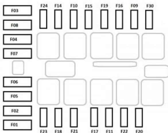
Fiat Ducato BASE CAMPER – fuse box – engine
