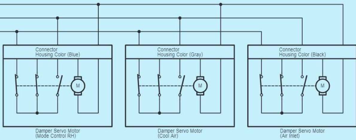
z34(C) A/C Blower Assembly
