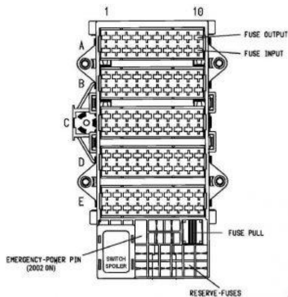
Porsche 996 – fuse box diagram
