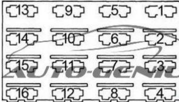
Chrysler New Yorker – fuse box diagram
