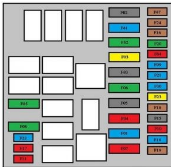
Citroen Nemo – fuse box diagram – engine
