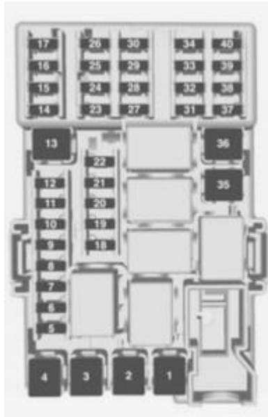
Vauxhall Adam-2014 – fuse box – instrument panel
