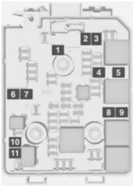
Vauxhall Adam (2014) – fuse box – engine
