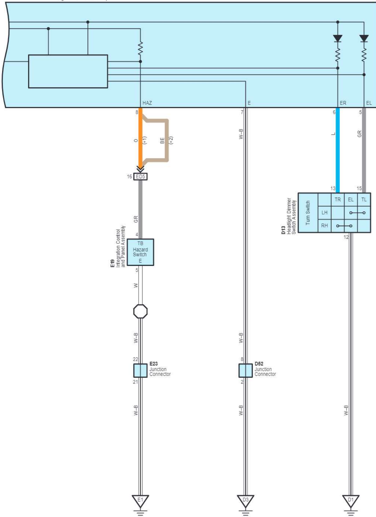
D12 Turn Signal Flasher Assembly
