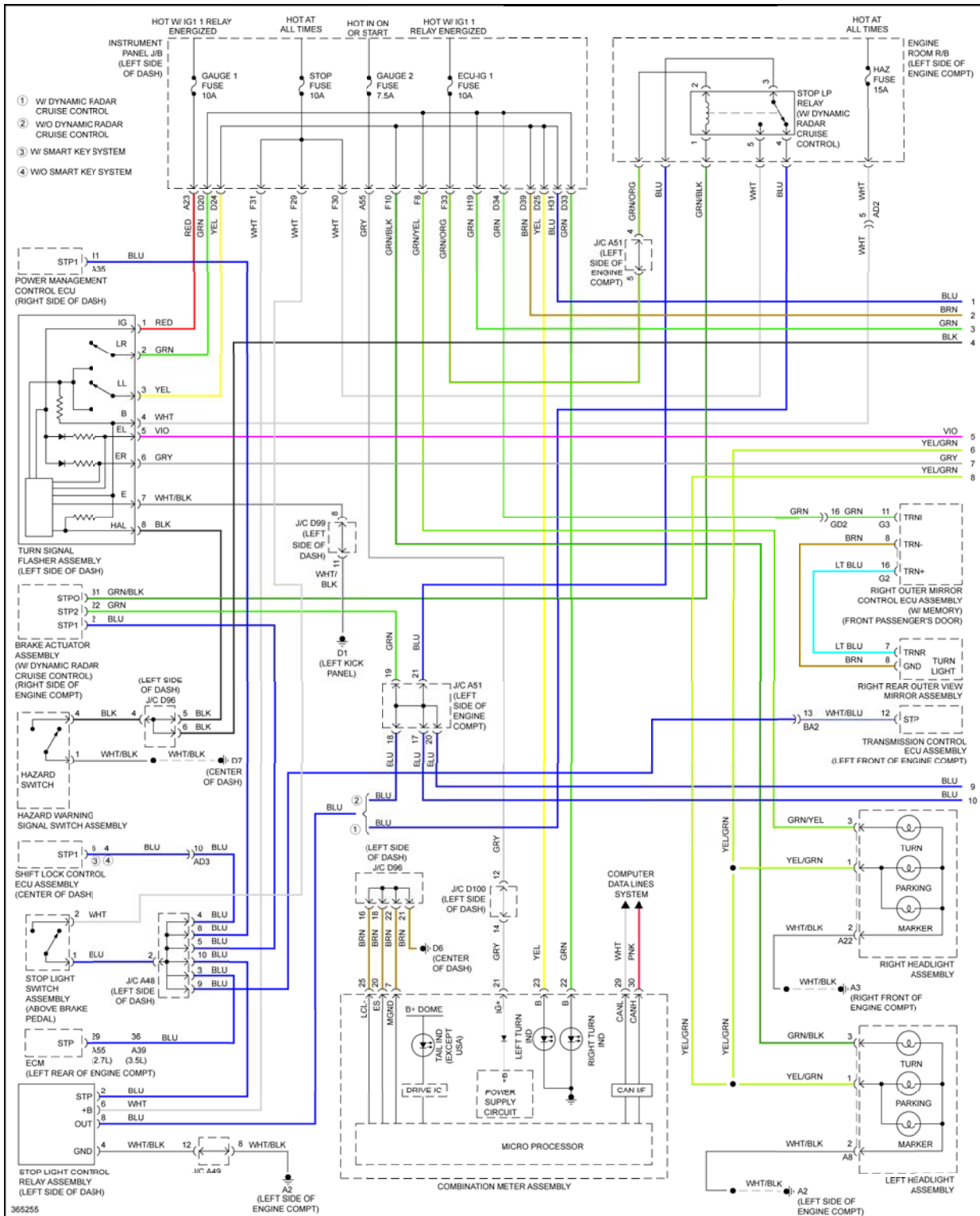
Fig. 40: Exterior Lamps Circuit (1 of 2)
