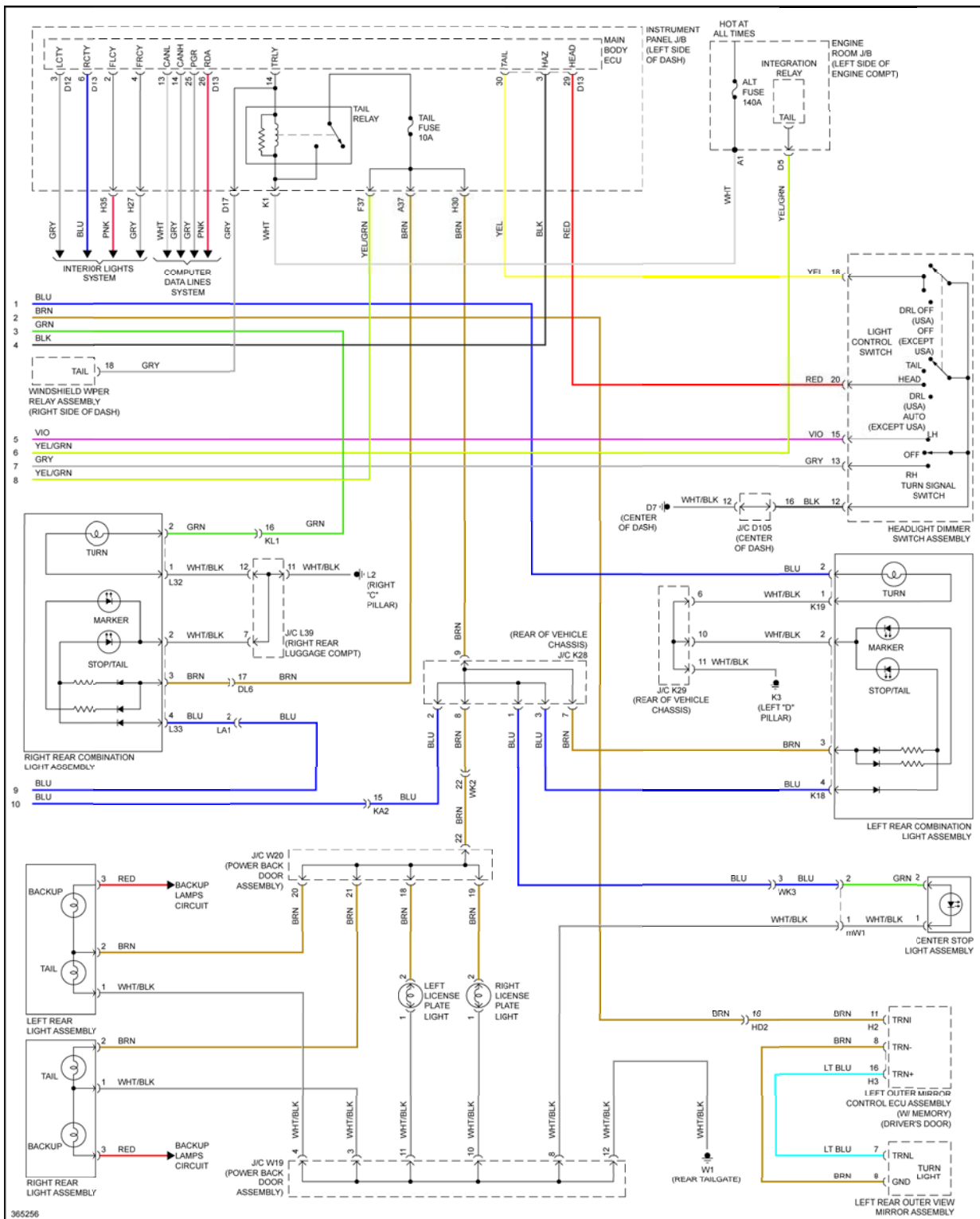
Fig. 41: Exterior Lamps Circuit (2 of 2)
