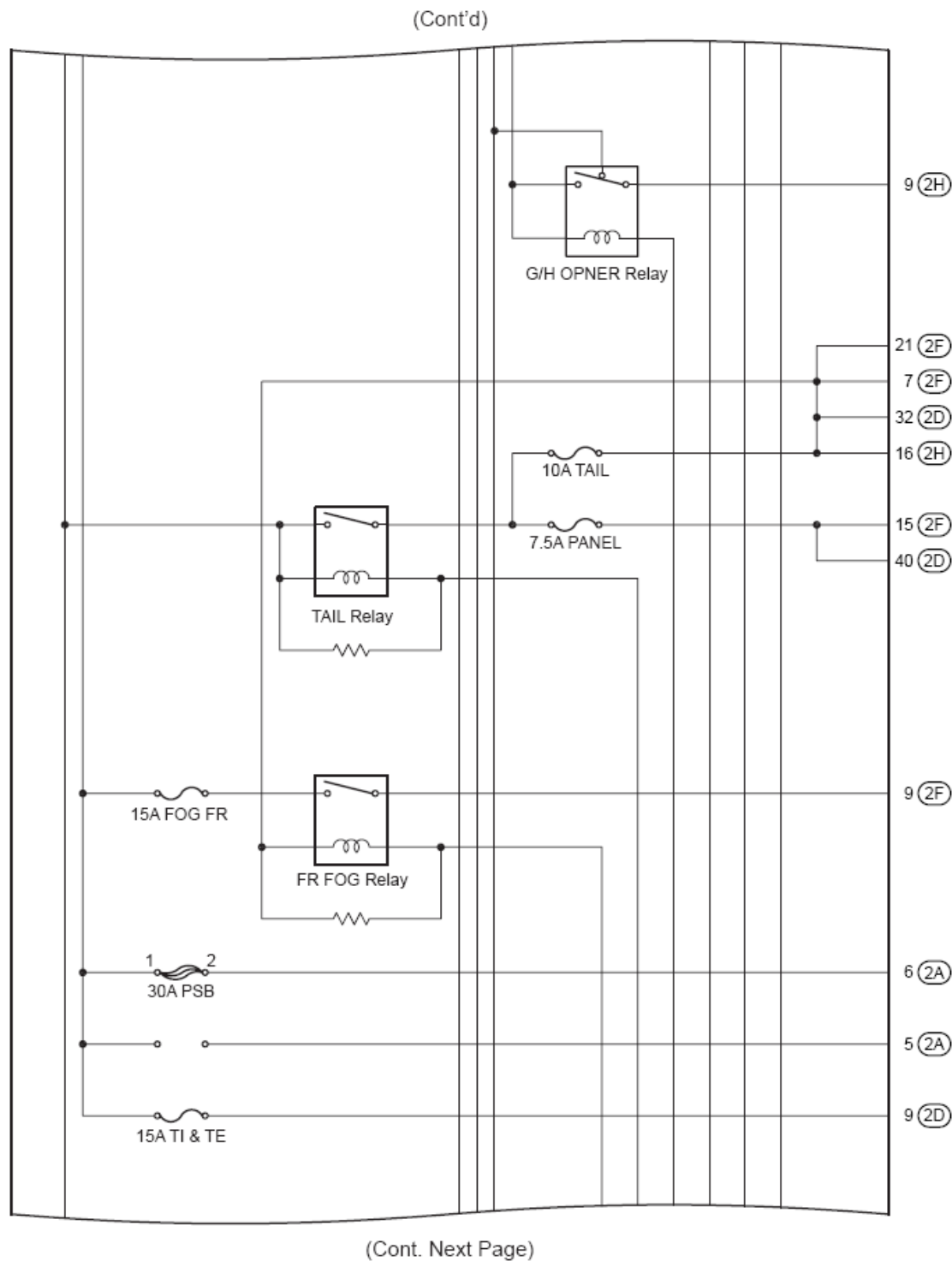
Fig. 17: Instrument Panel J/B Assembly Inner Circuit Diagram (2 Of 6)
