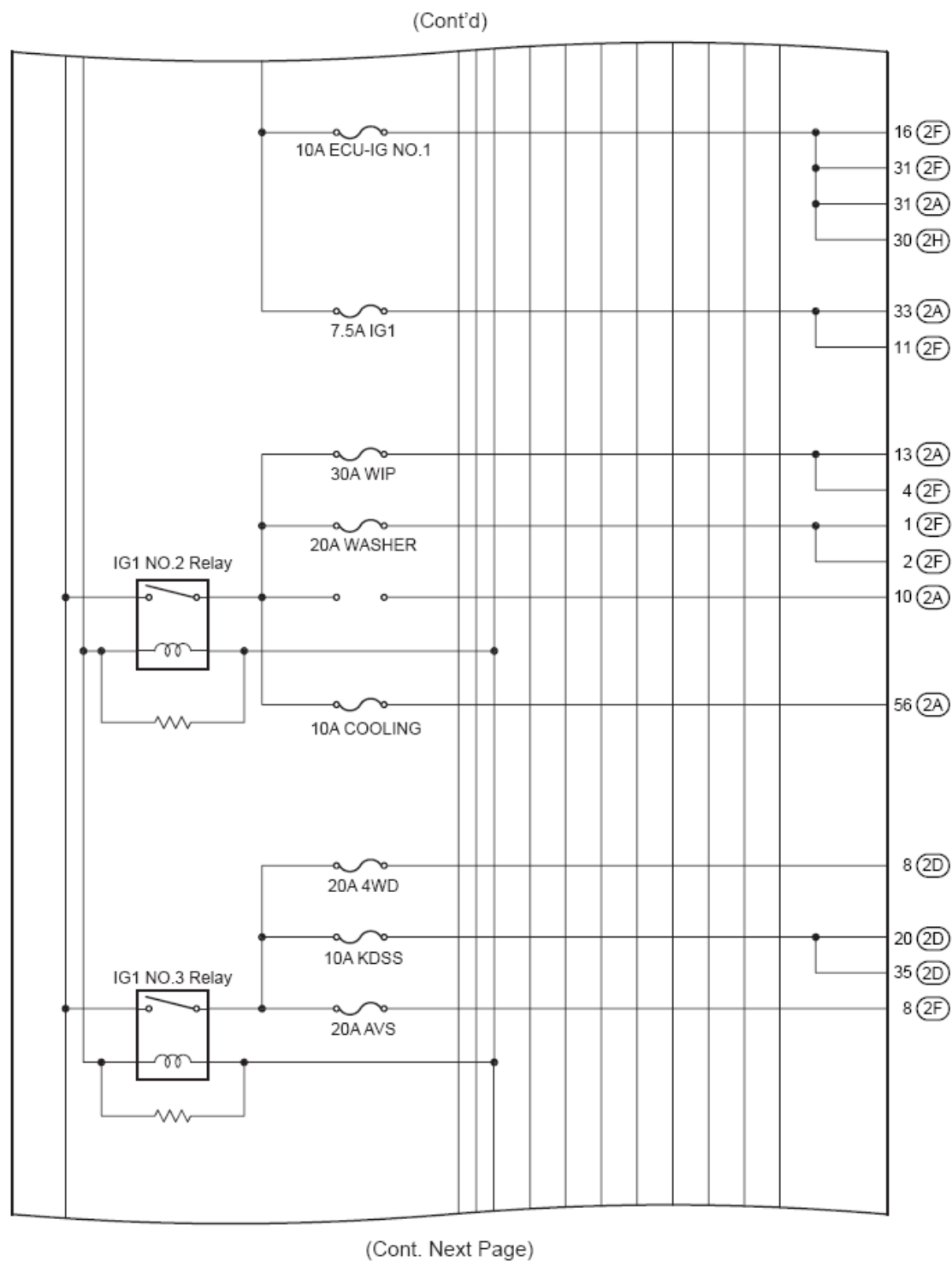
Fig. 19: Instrument Panel J/B Assembly Inner Circuit Diagram (4 Of 6)
