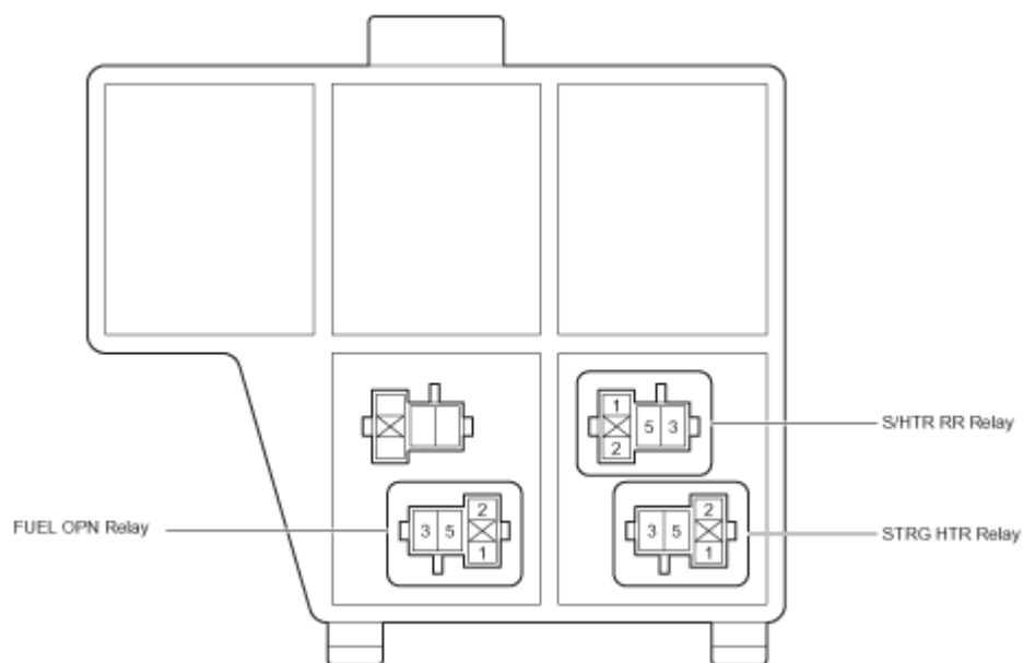
Fig. 11: Engine Room R/B No. 3 - Dash Panel Relay Locations
