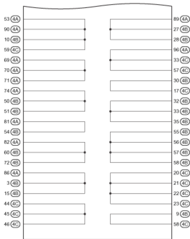
Fig. 31: J/B No. 4 Inner Circuit Diagram (4 Of 4)
