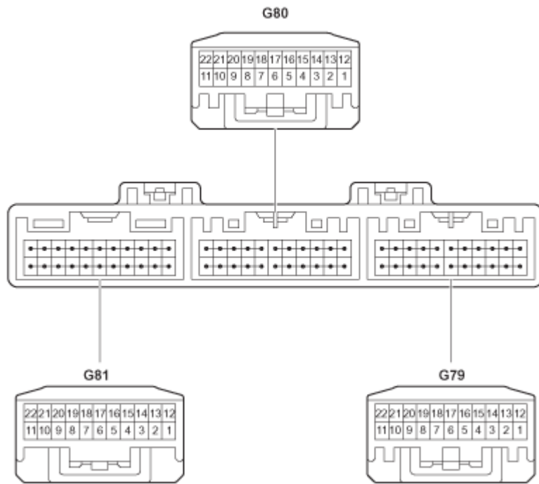
Fig. 32: Junction Connector (CAN LH) - Instrument Panel Reinforcement Connector Locations
