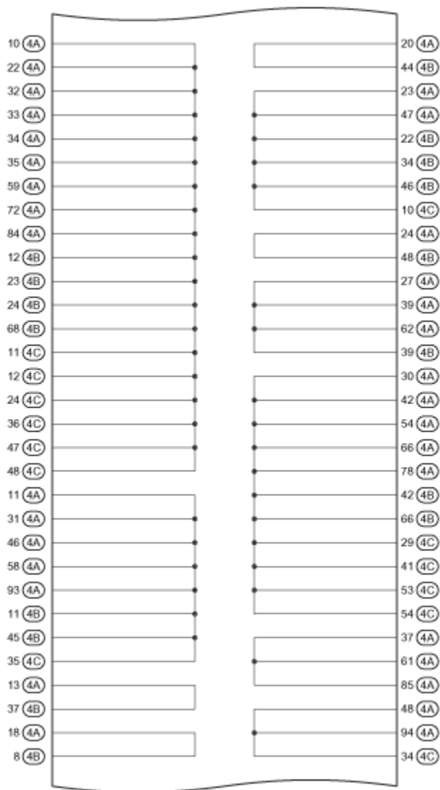
Fig. 29: J/B No. 4 Inner Circuit Diagram (2 Of 4)
