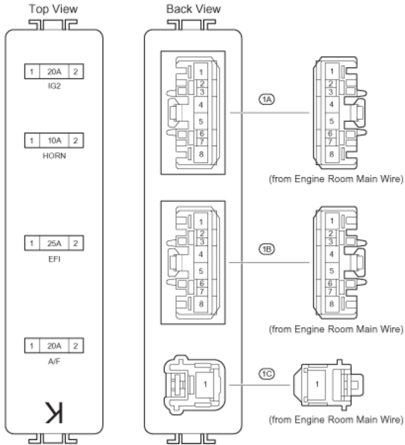
Fig. 8: Engine Room R/B And J/B Assembly - Front Fender Apron LH Connector Locations (Unit K)
