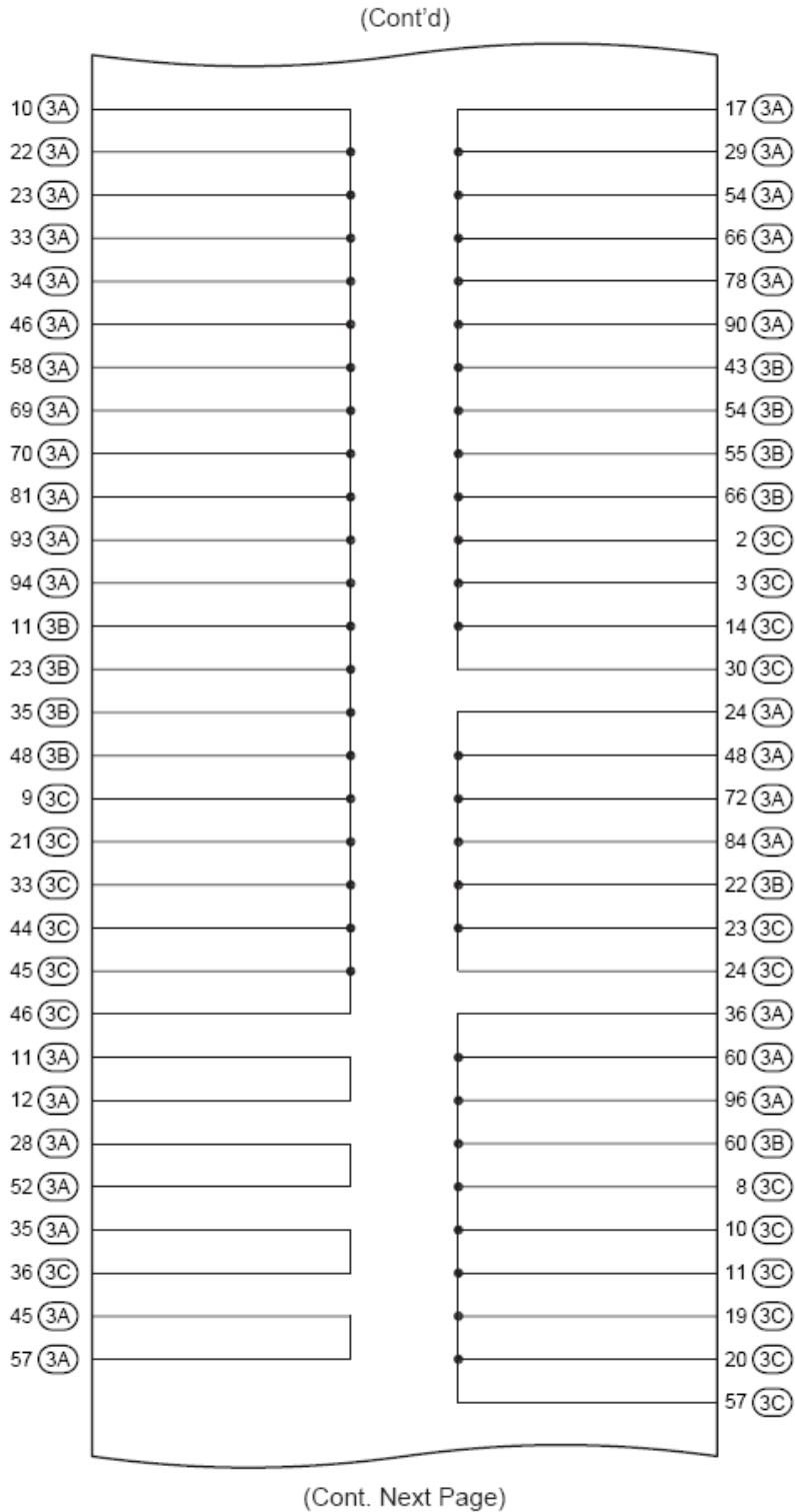
Fig. 24: J/B No. 3 Inner Circuit Diagram (2 Of 4)
