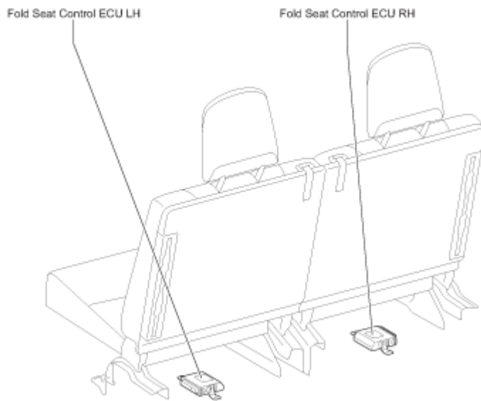
Fig. 5: Rear No. 2 Seat ECU Locations
