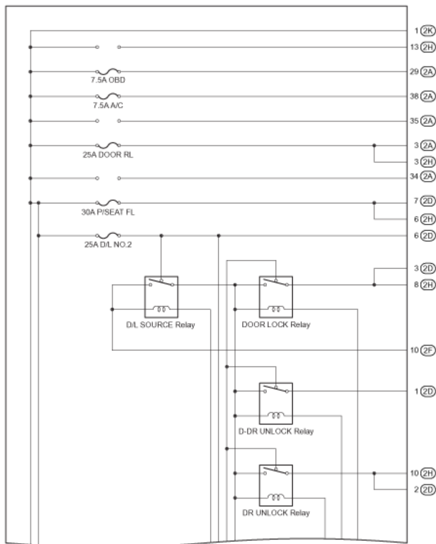
Fig. 16: Instrument Panel J/B Assembly Inner Circuit Diagram (1 Of 6)
