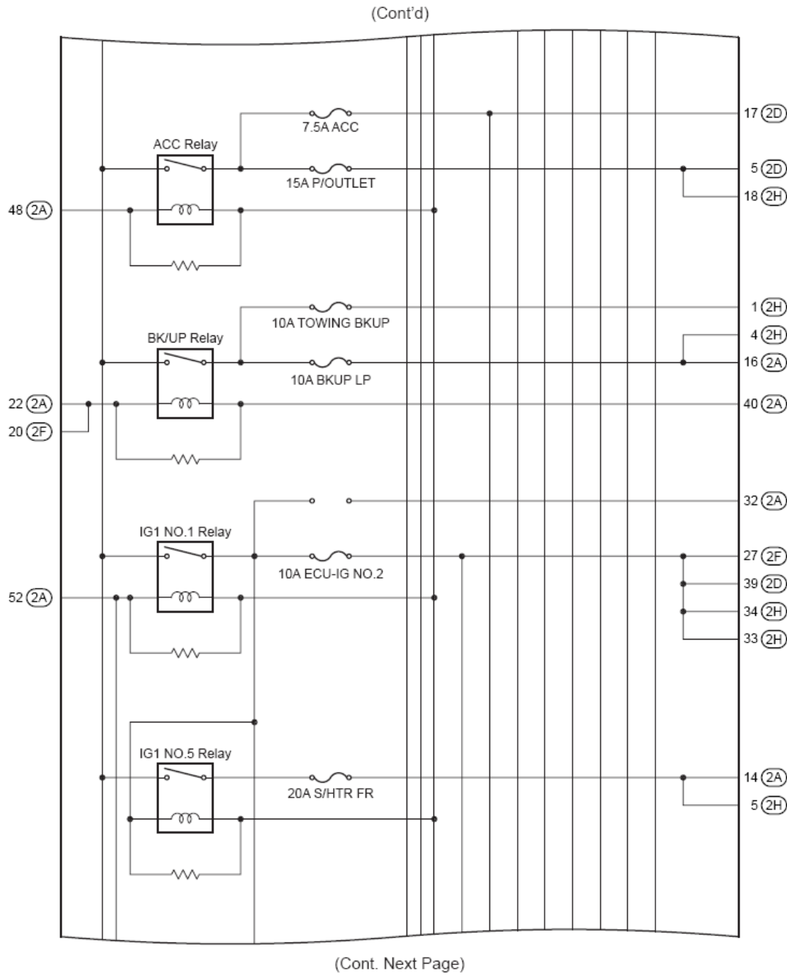
Fig. 18: Instrument Panel J/B Assembly Inner Circuit Diagram (3 Of 6)
