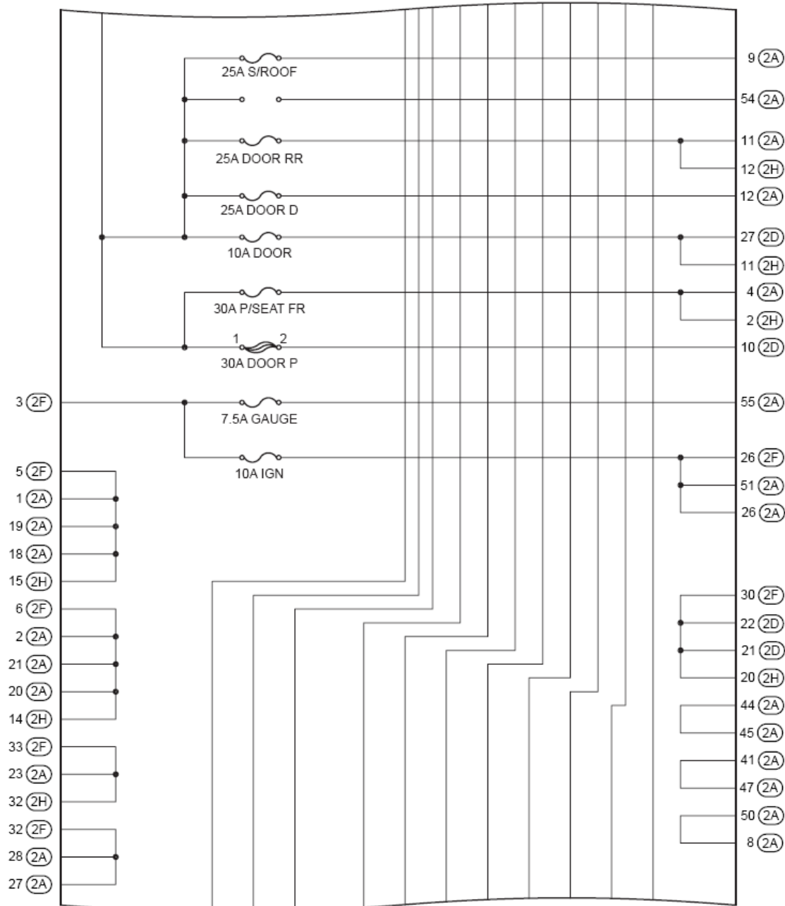
Fig. 20: Instrument Panel J/B Assembly Inner Circuit Diagram (5 Of 6)
