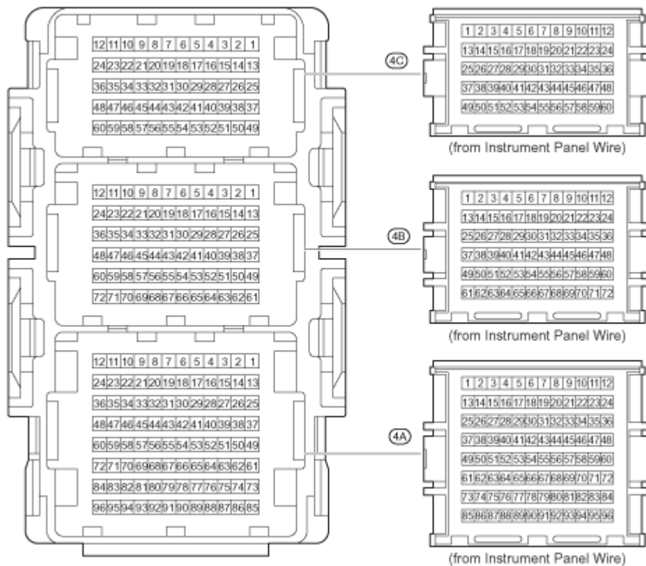
Fig. 27: J/B No. 4 - Instrument Panel Reinforcement Connector Locations
