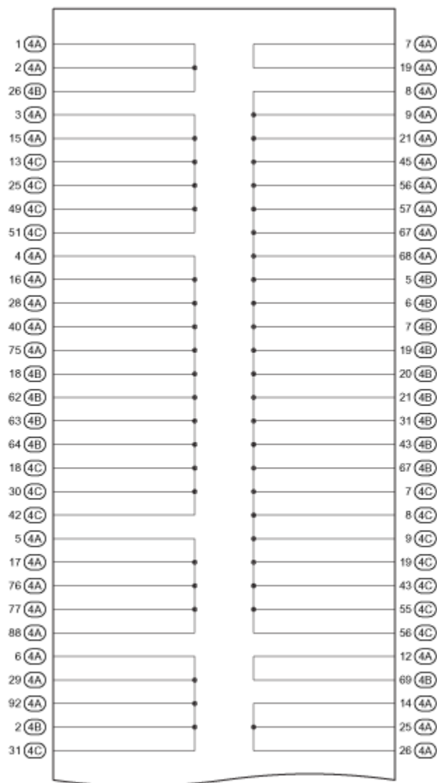
Fig. 28: J/B No. 4 Inner Circuit Diagram (1 Of 4)
