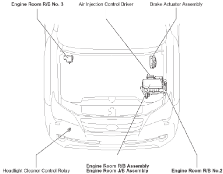
Fig. 1: Engine Compartment Junction Block, ECU & Fuse/Relay Locations
