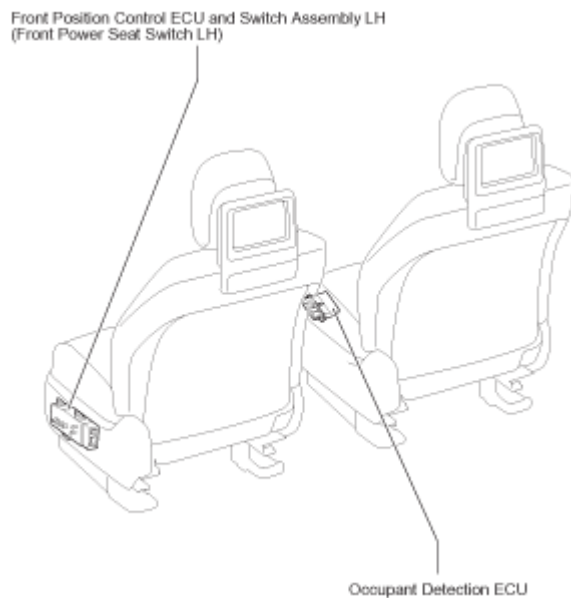
Fig. 4: Front Seat ECU Locations
