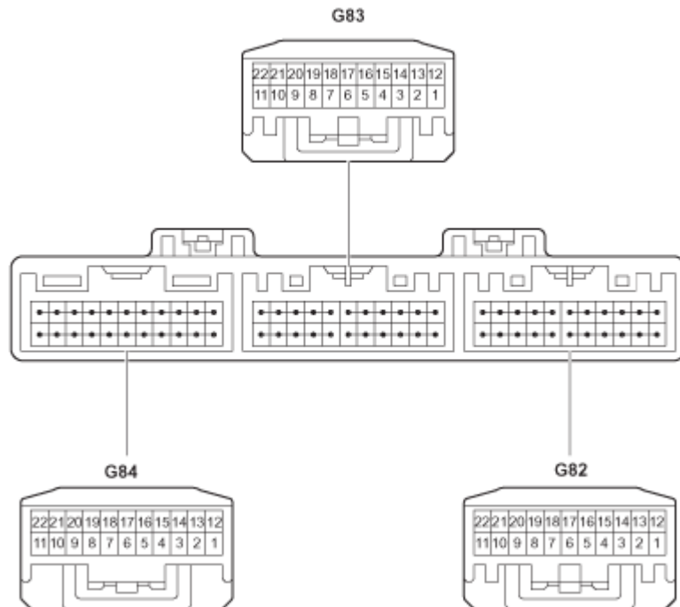
Fig. 33: Junction Connector (CAN RH) - Instrument Panel Reinforcement Connector Locations
