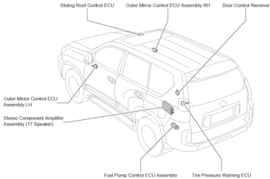
Fig. 3: Body ECU Locations
