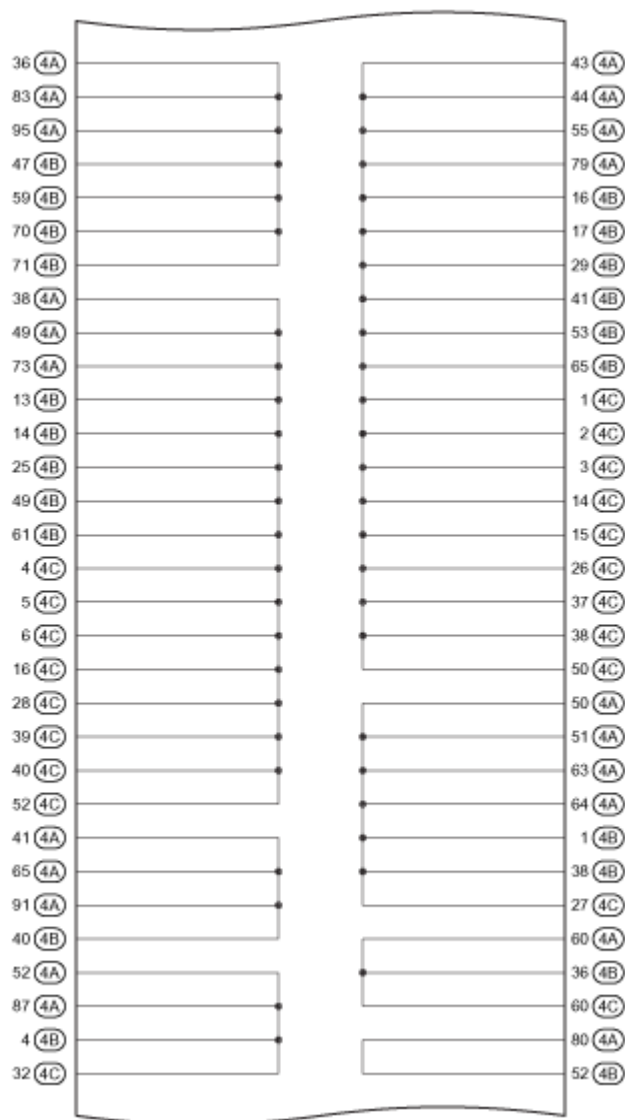
Fig. 30: J/B No. 4 Inner Circuit Diagram (3 Of 4)
