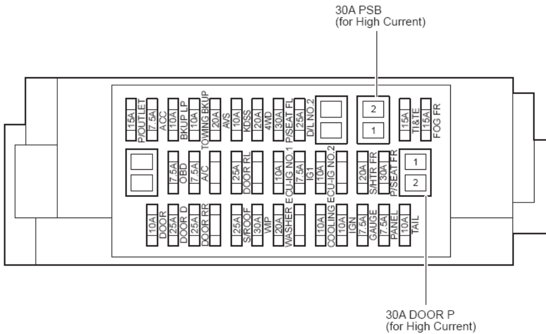
Fig. 15: Instrument Panel J/B Assembly - Instrument Panel Reinforcement Connector Locations (View C)
