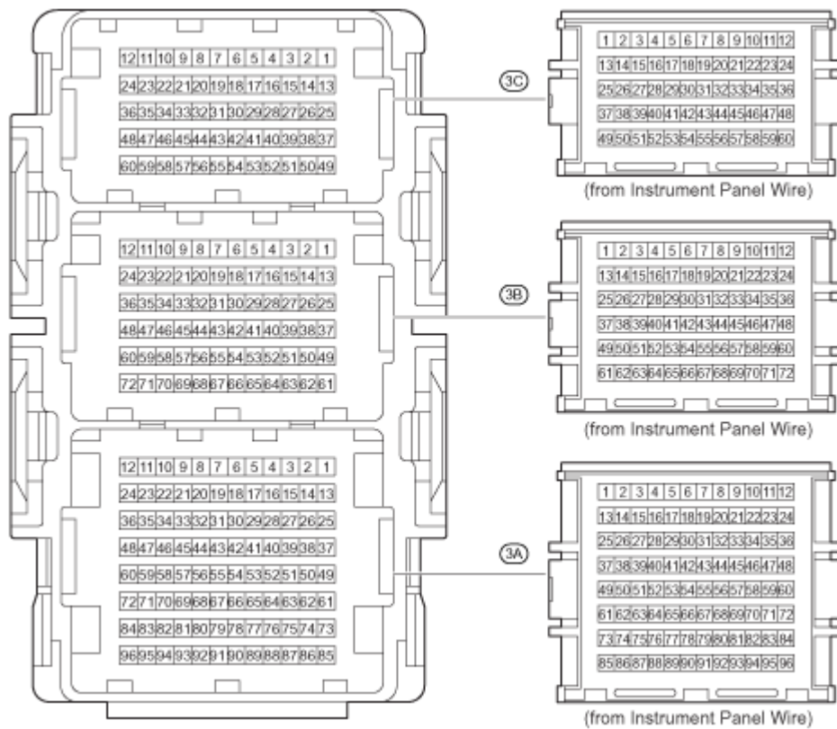
Fig. 22: J/B No. 3 - Instrument Panel Reinforcement Connector Locations
