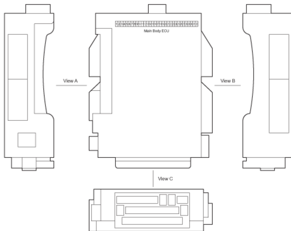
Fig. 12: Instrument Panel J/B Assembly - Instrument Panel Reinforcement Connector Locations
