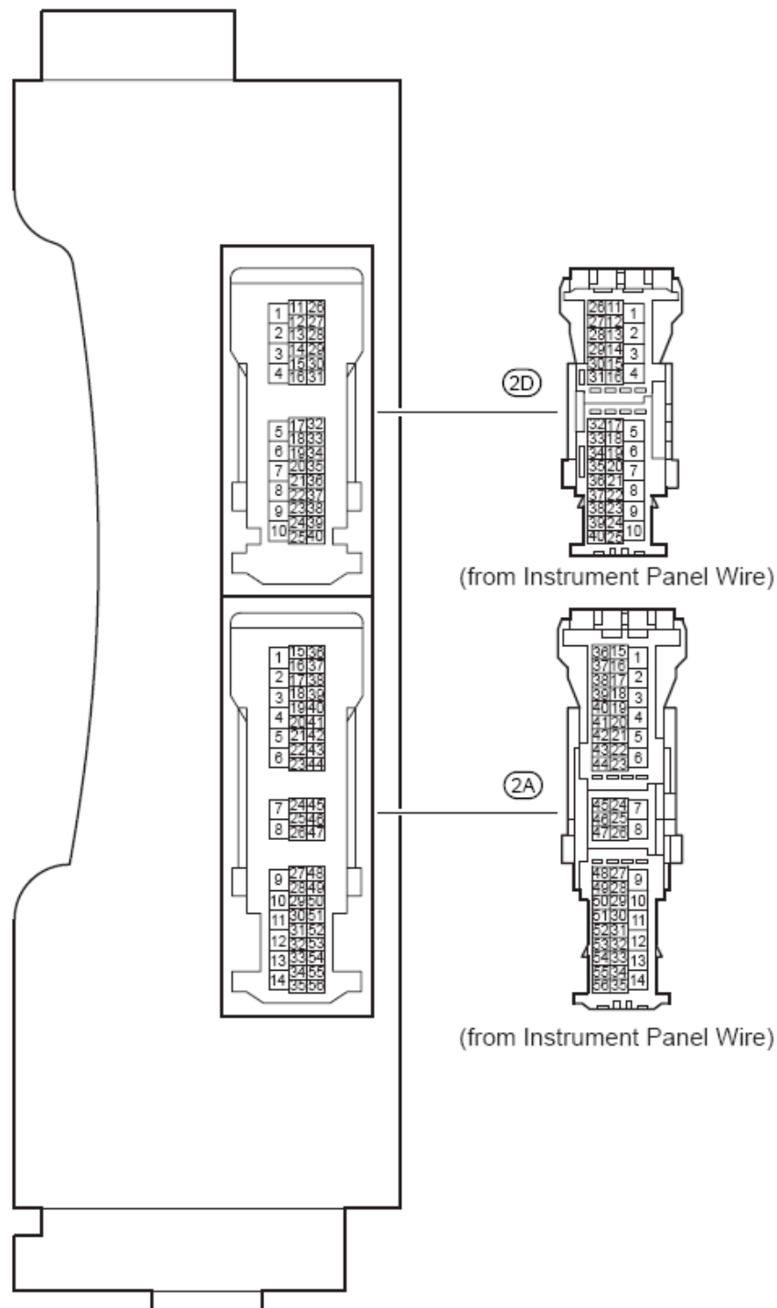
Fig. 14: Instrument Panel J/B Assembly - Instrument Panel Reinforcement Connector Locations (View B)
