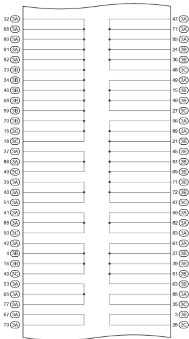
Fig. 25: J/B No. 3 Inner Circuit Diagram (3 Of 4)
