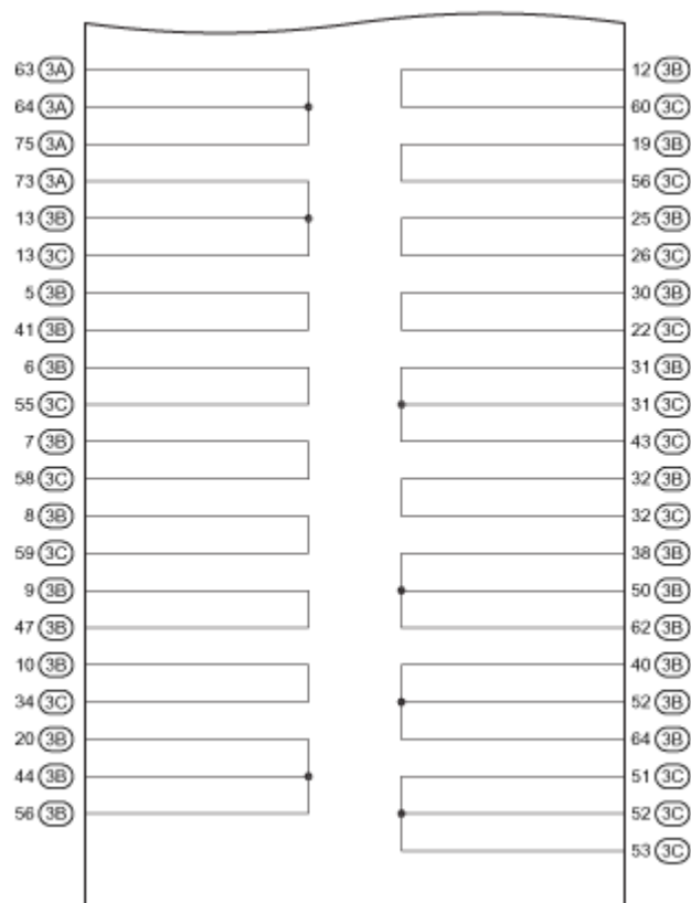
Fig. 26: J/B No. 3 Inner Circuit Diagram (4 Of 4)
