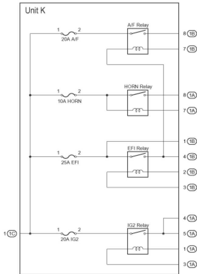
Fig. 9: Engine Room R/B Assembly And J/B Assembly Inner Circuit Diagram
