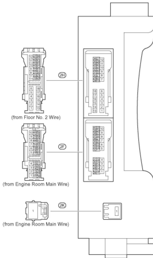
Fig. 13: Instrument Panel J/B Assembly - Instrument Panel Reinforcement Connector Locations (View A)
