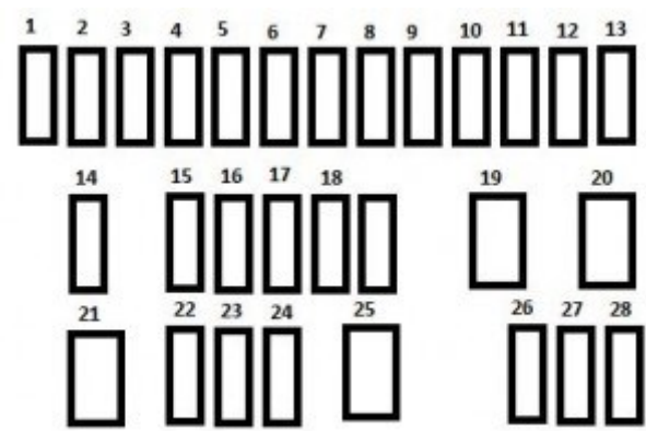
Citoren C1 mk2 – fuse box – under dashboard
