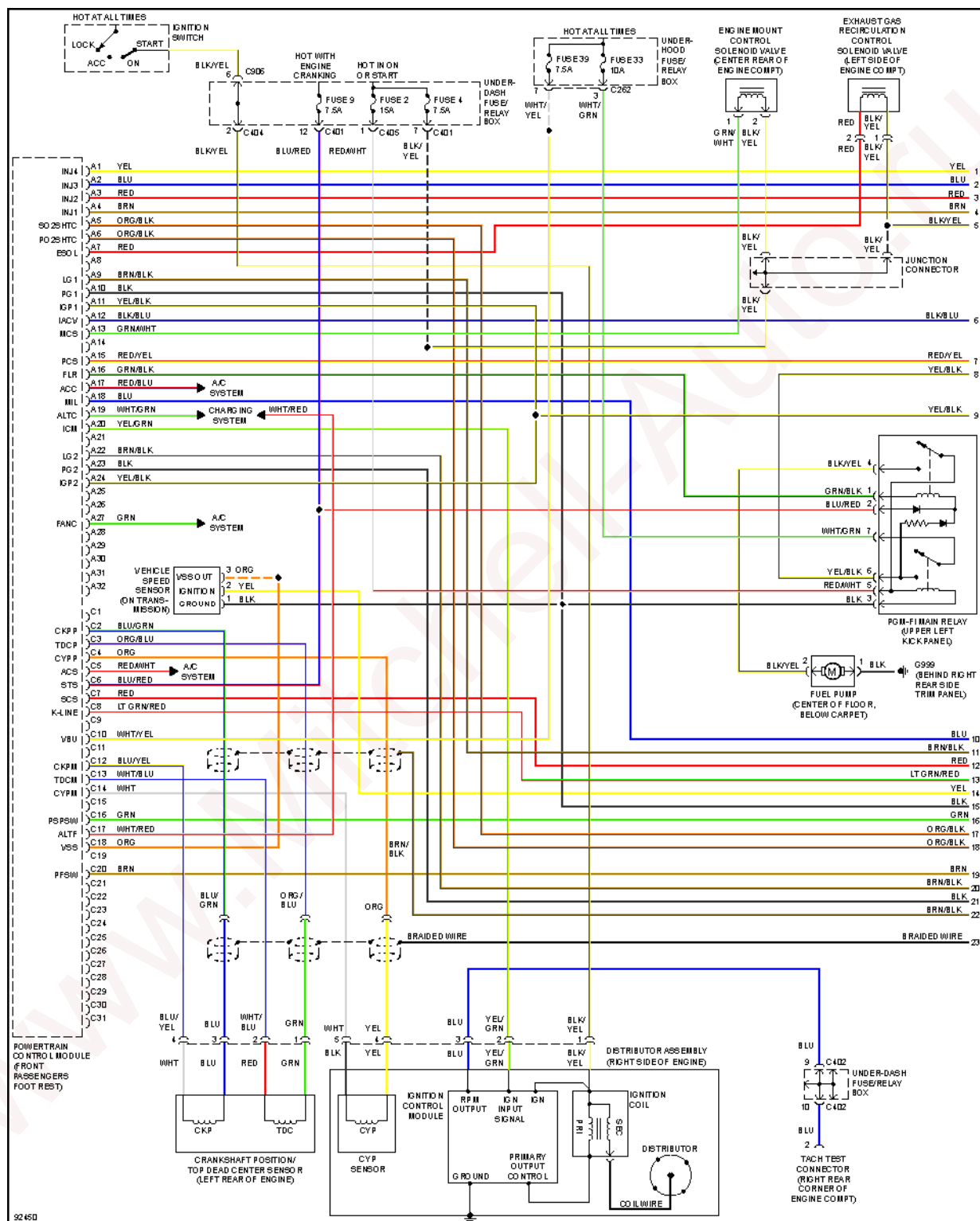
Fig. 9: 2.2L, Engine Performance Circuits (1 of 3)
