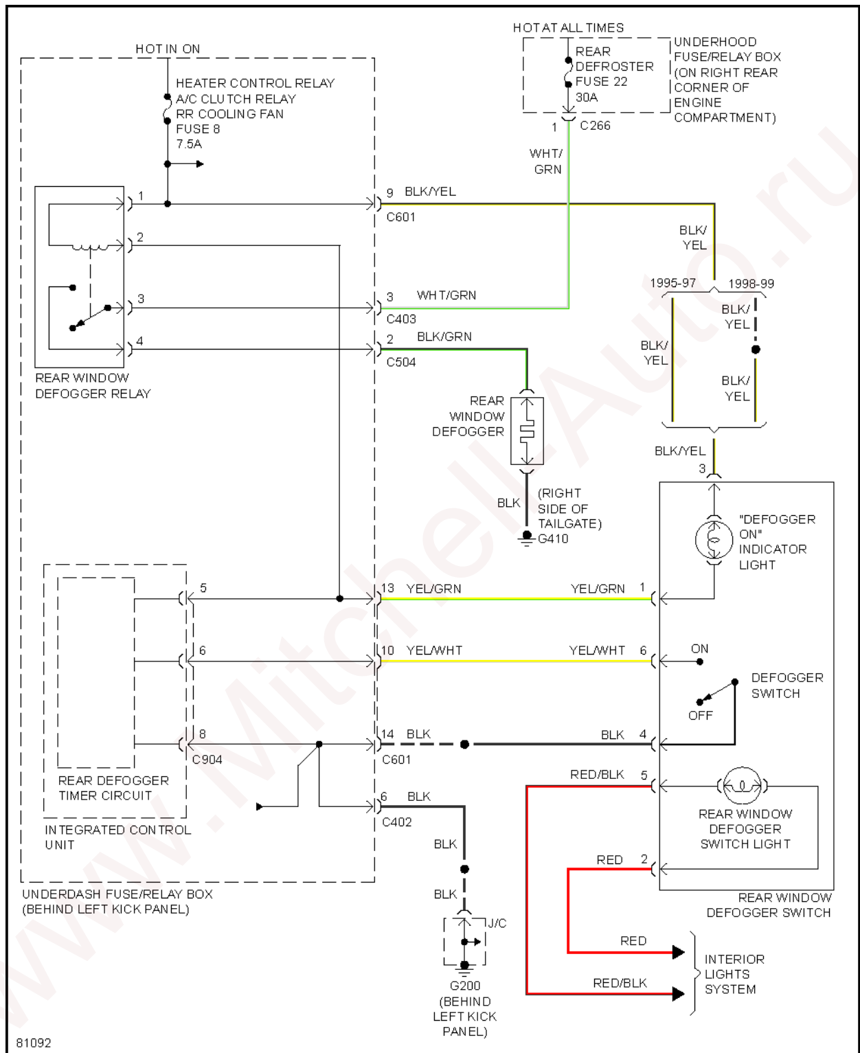
Fig. 8: Defogger Circuit
