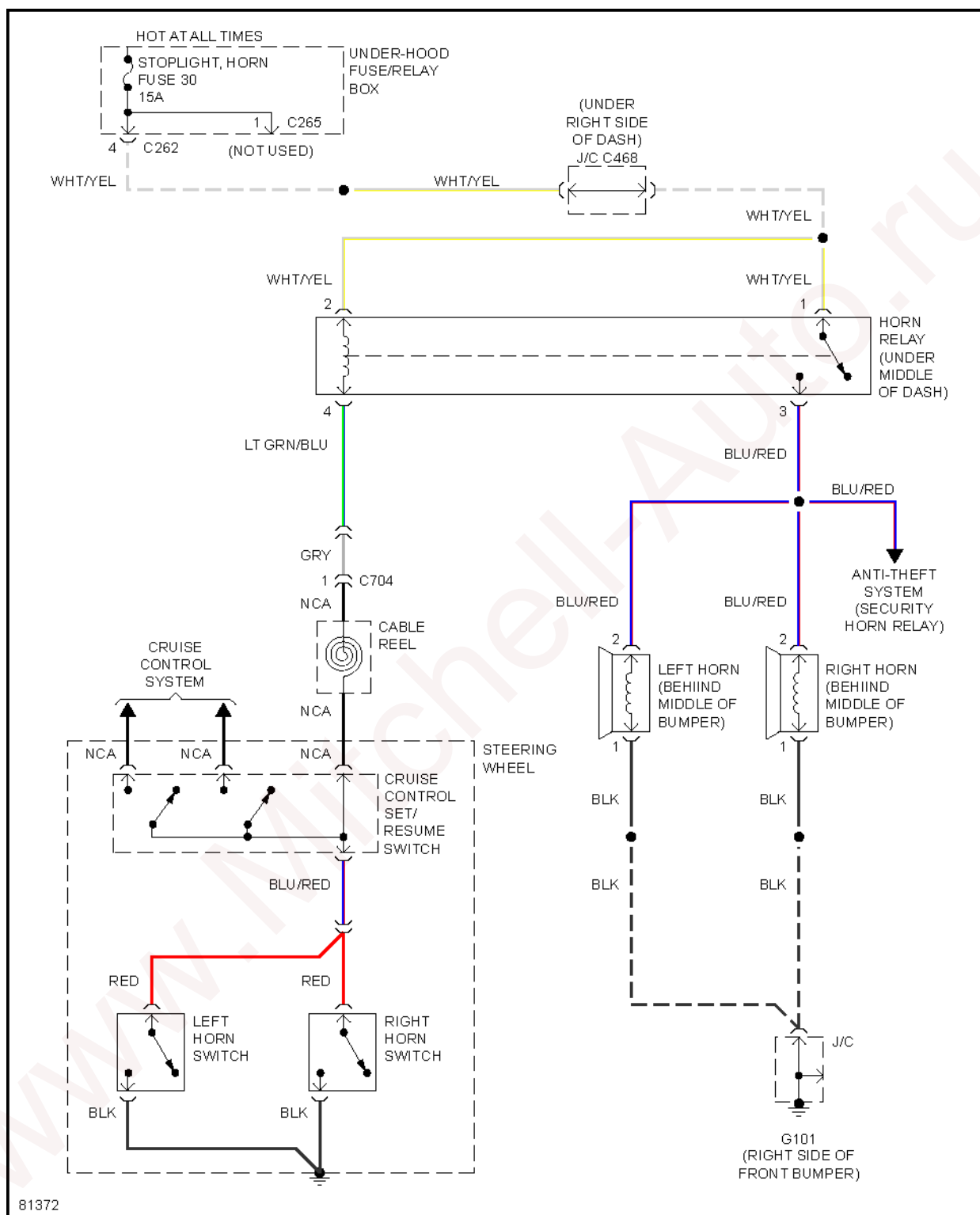
Fig. 20: Horn Circuit
