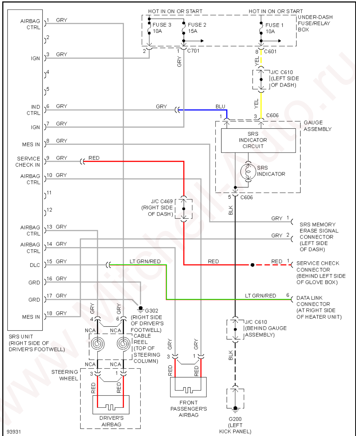
Fig. 40: Supplemental Restraint Circuit
