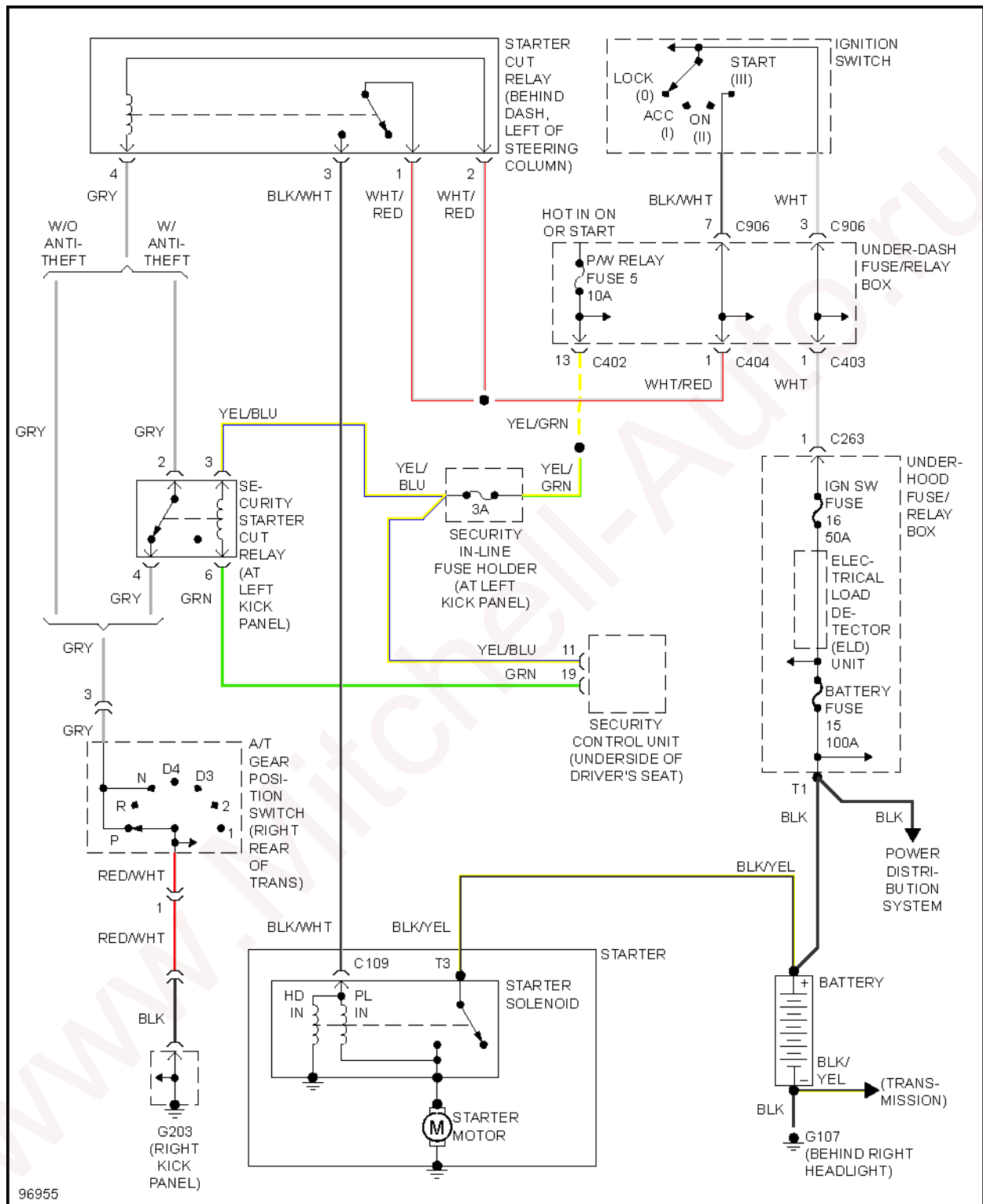
Fig. 39: Starting Circuit
