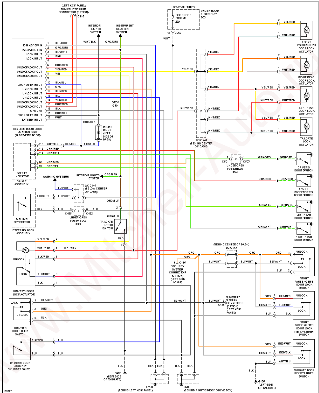
Fig. 30: Power Door Lock Circuit, W/ Keyless Entry
