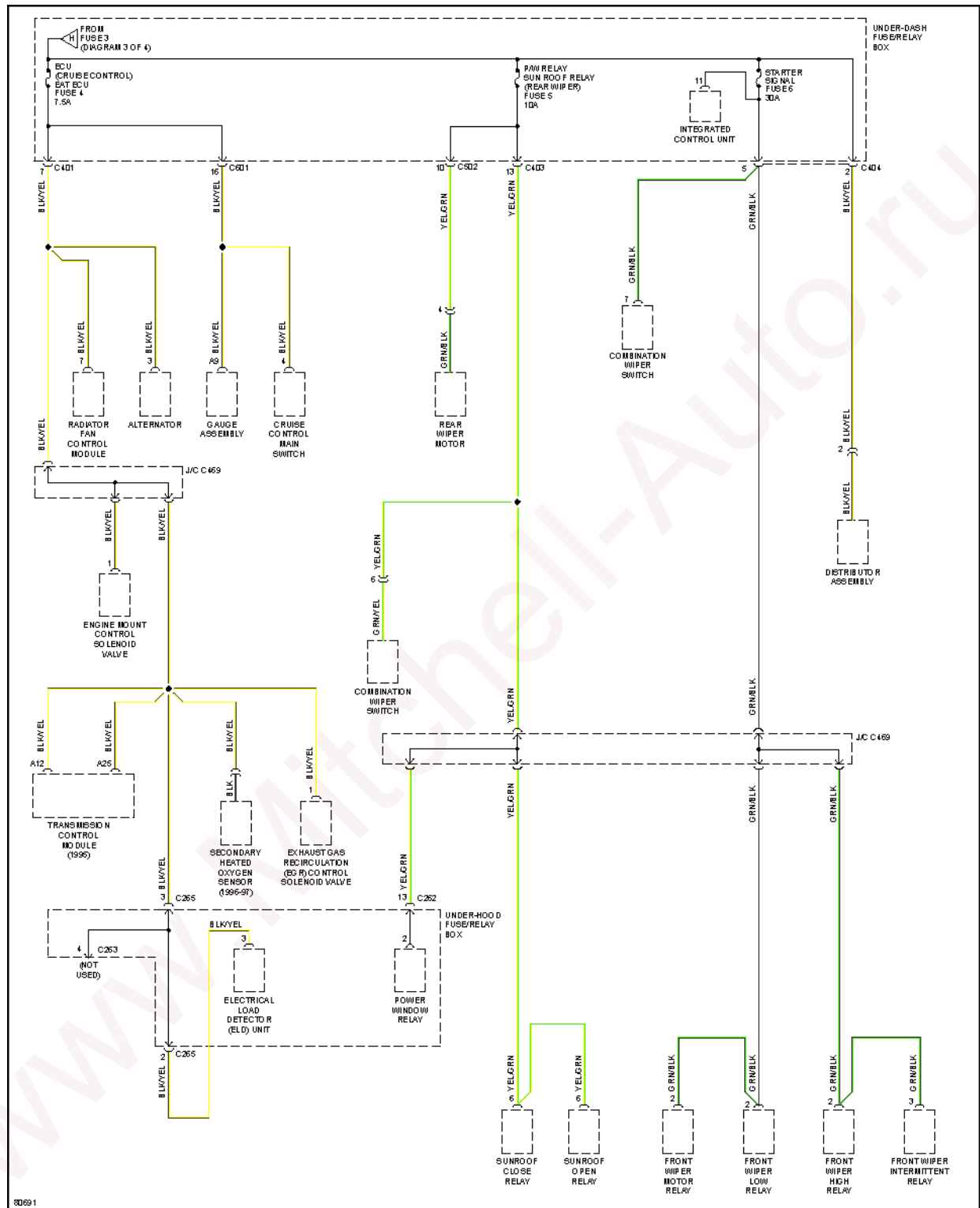
Fig. 29: Power Distribution Circuit (4 of 4)
