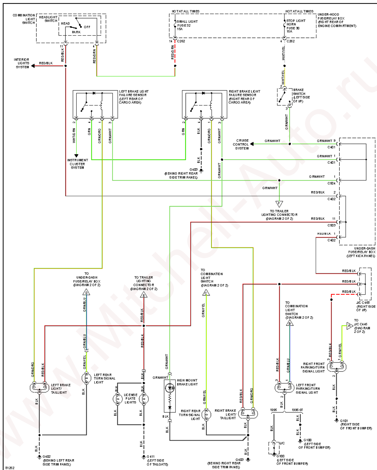
Fig. 13: Exterior Lamps Circuit (1 of 2)
