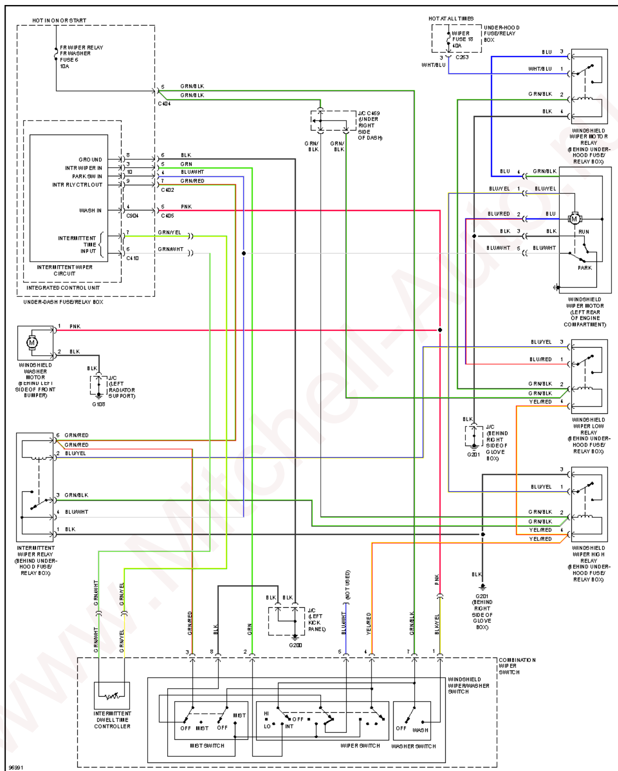
Fig. 43: Front Washer/Wiper Circuit
