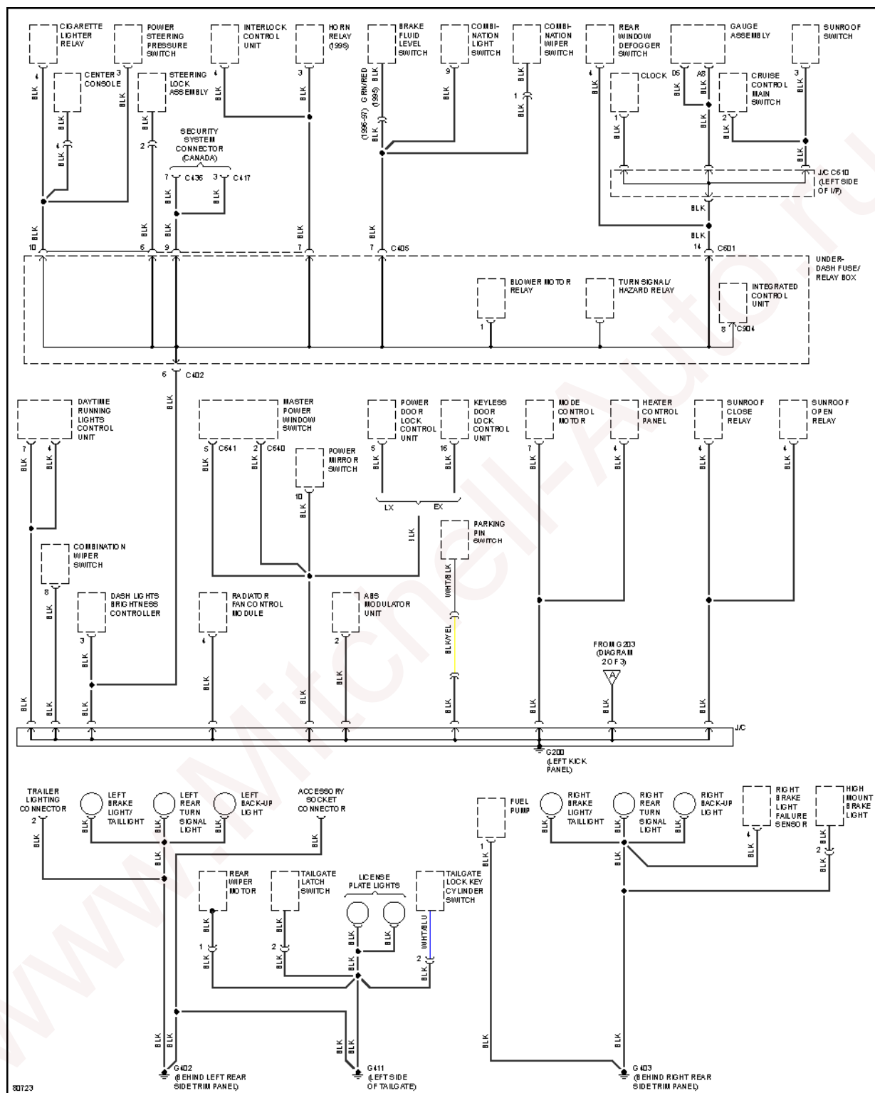
Fig. 17: Ground Distribution Circuit (3 of 3)
