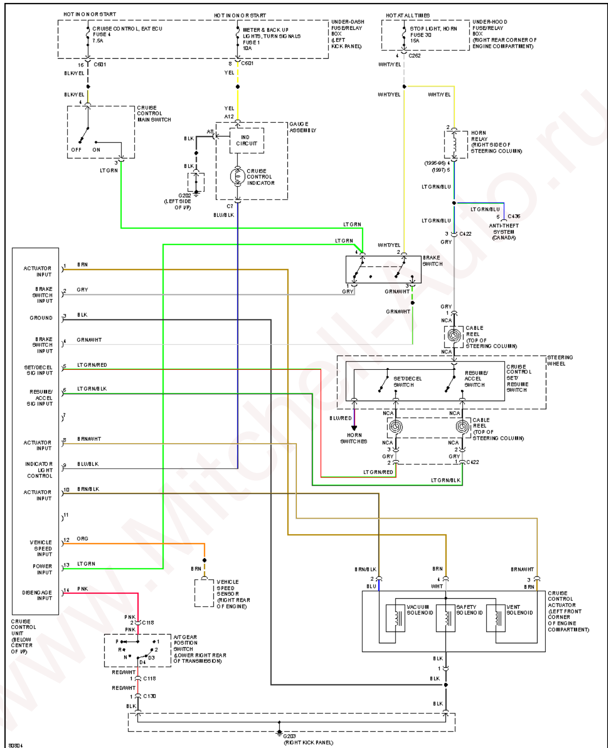
Fig. 7: Cruise Control Circuit
