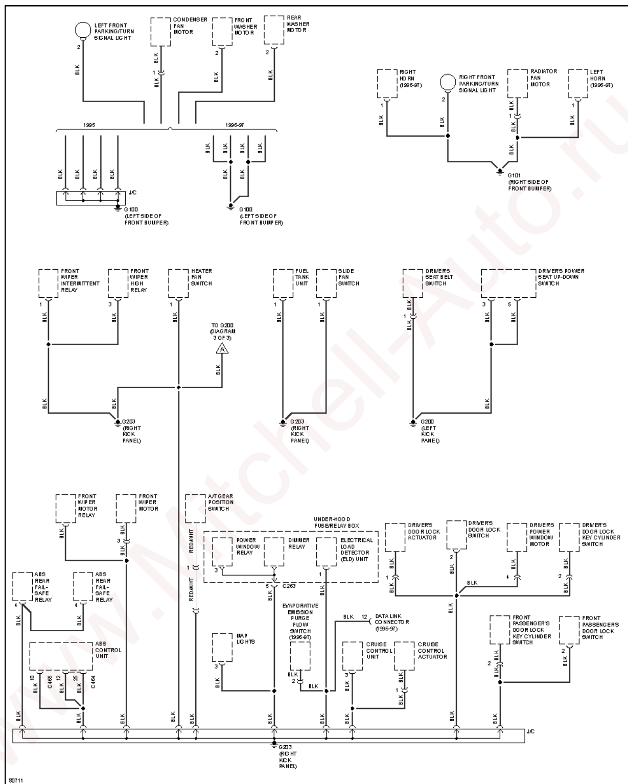
Fig. 16: Ground Distribution Circuit (2 of 3)
