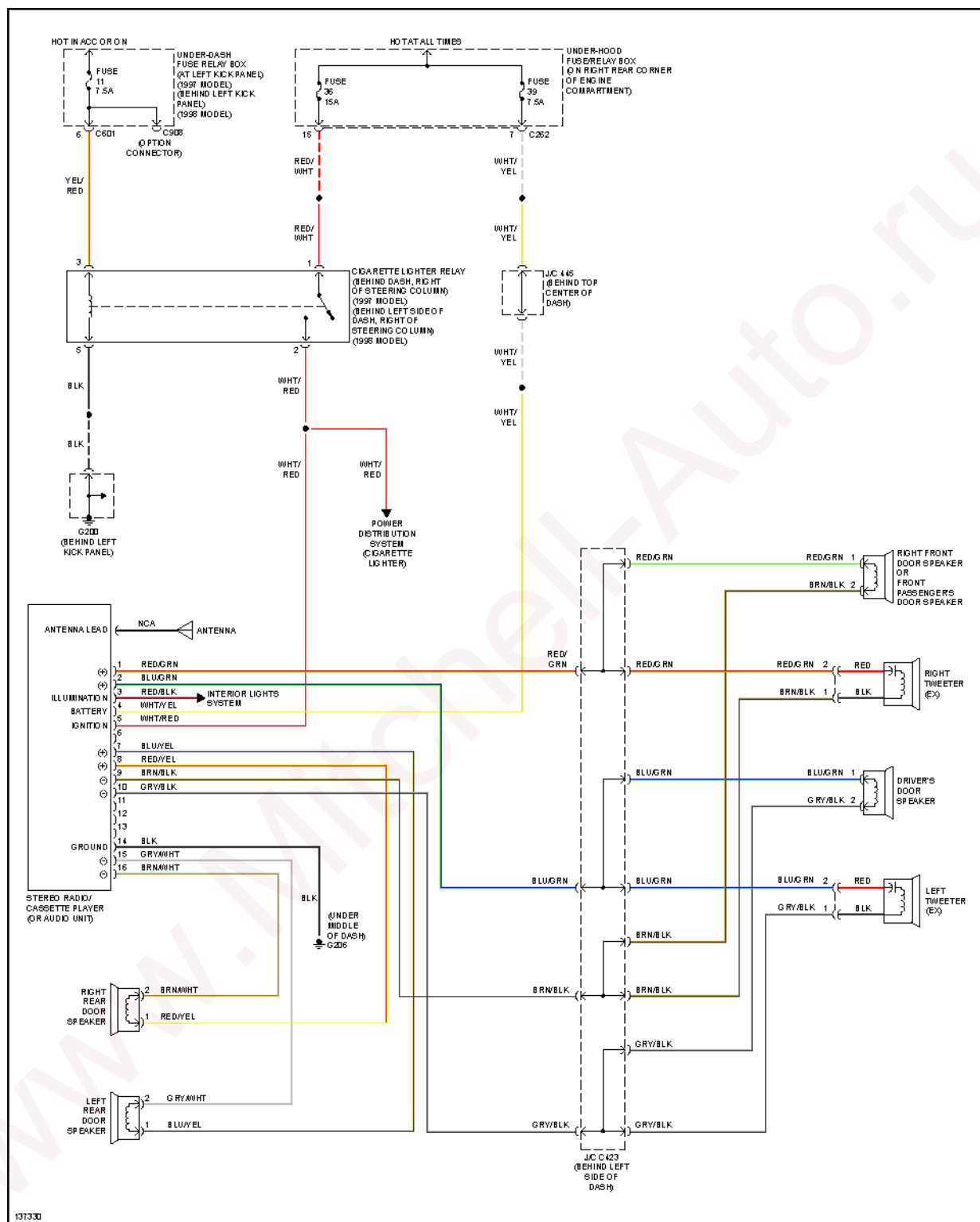
Fig. 36: Radio Circuits
