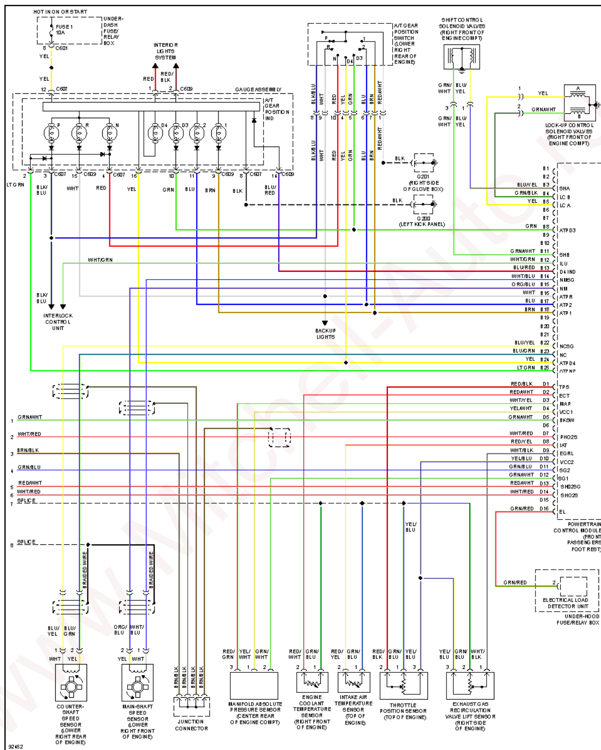
Fig. 11: 2.2L, Engine Performance Circuits (3 of 3)
