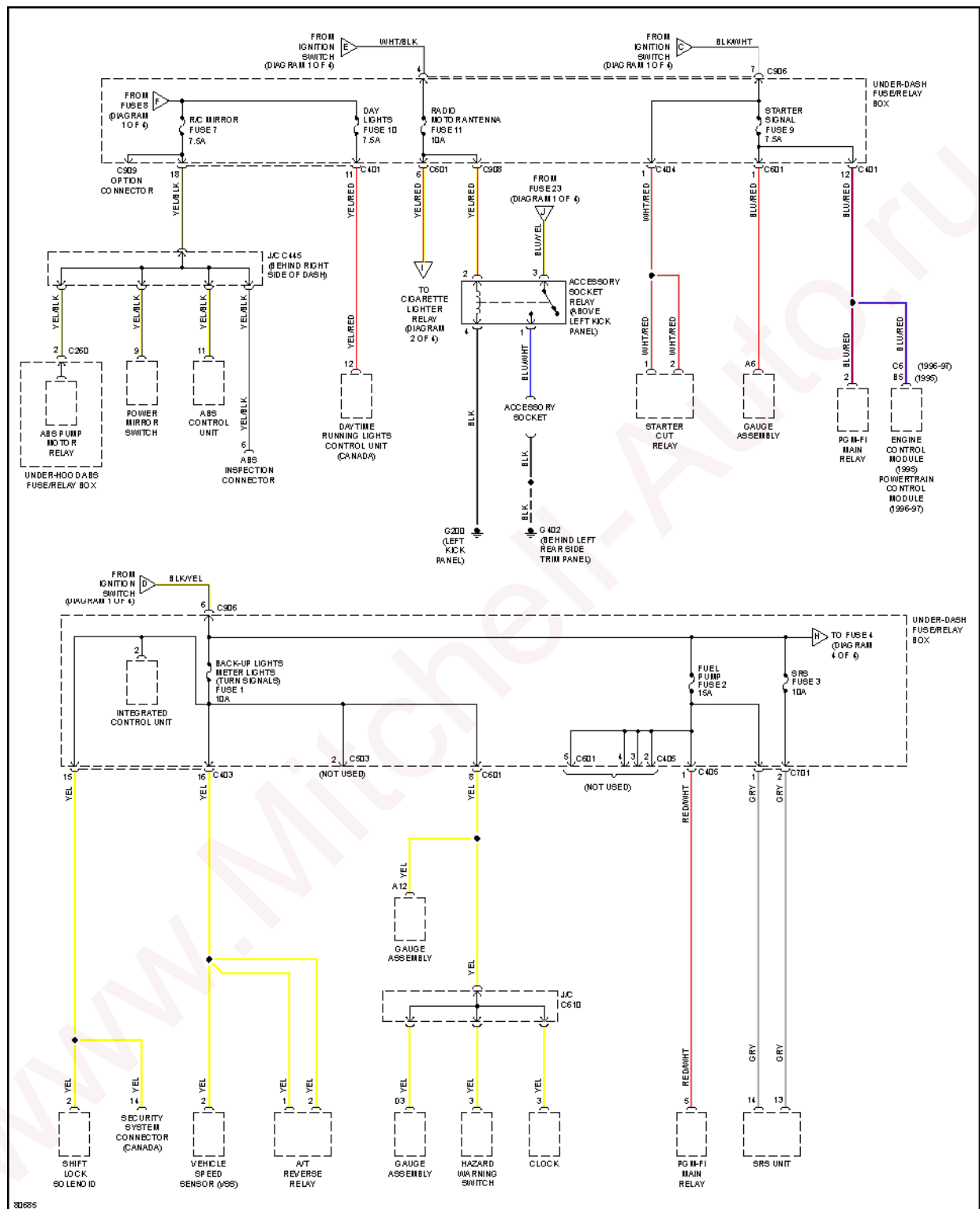
Fig. 28: Power Distribution Circuit (3 of 4)
