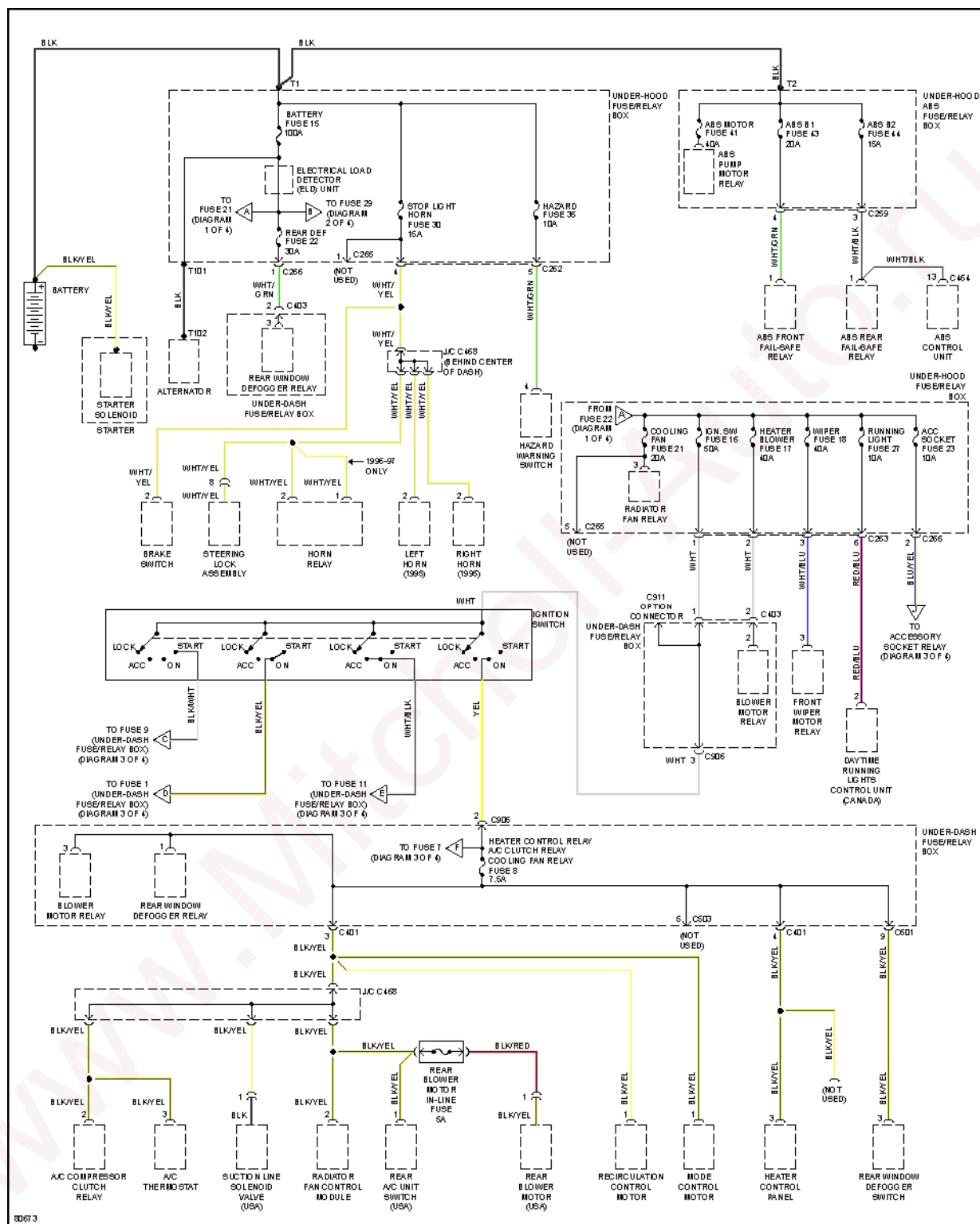
Fig. 26: Power Distribution Circuit (1 of 4)
