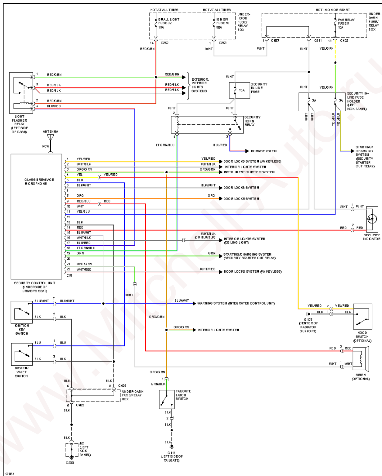
Fig. 4: Anti-theft Circuit
