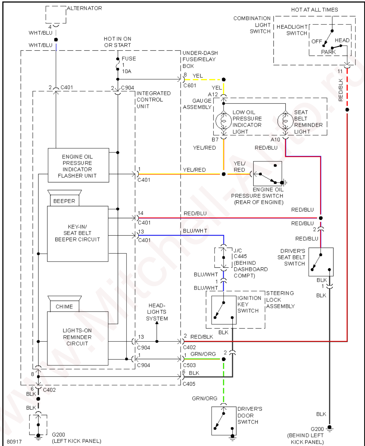
Fig. 42: Warning System Circuits
