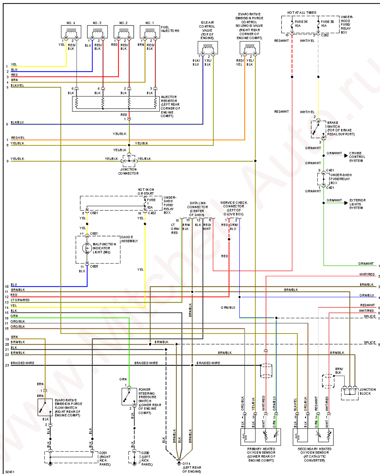
Fig. 10: 2.2L, Engine Performance Circuits (2 of 3)
