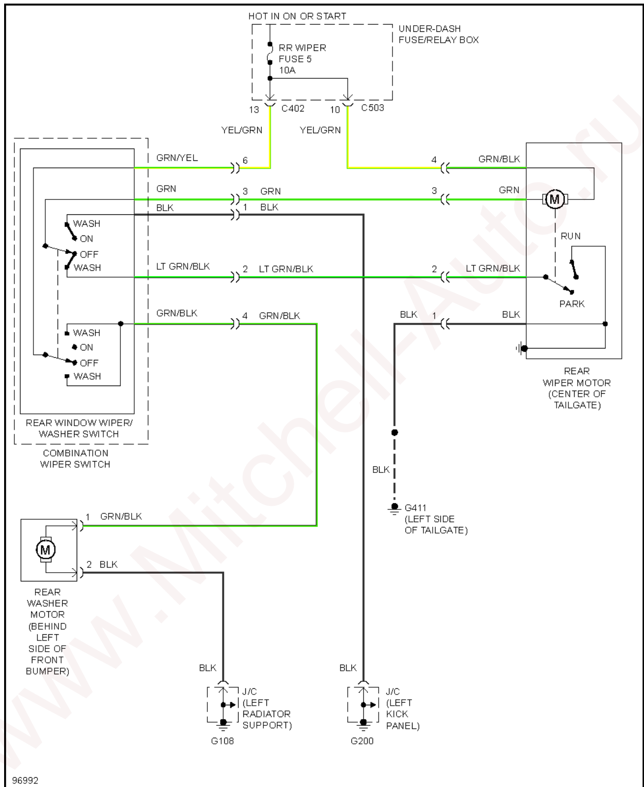
Fig. 44: Rear Washer/Wiper Circuit
