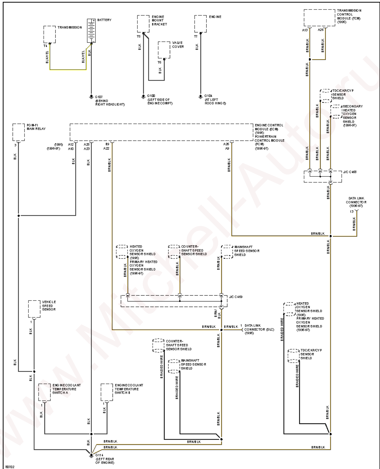
Fig. 15: Ground Distribution Circuit (1 of 3)
