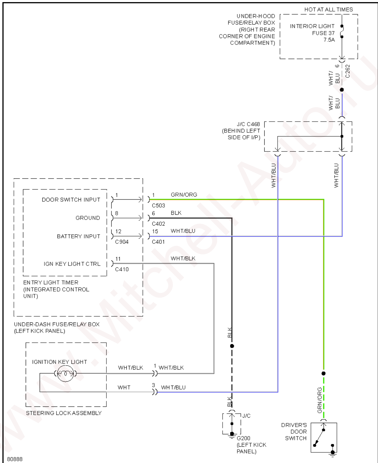
Fig. 24: Ignition Key Light Circuit
