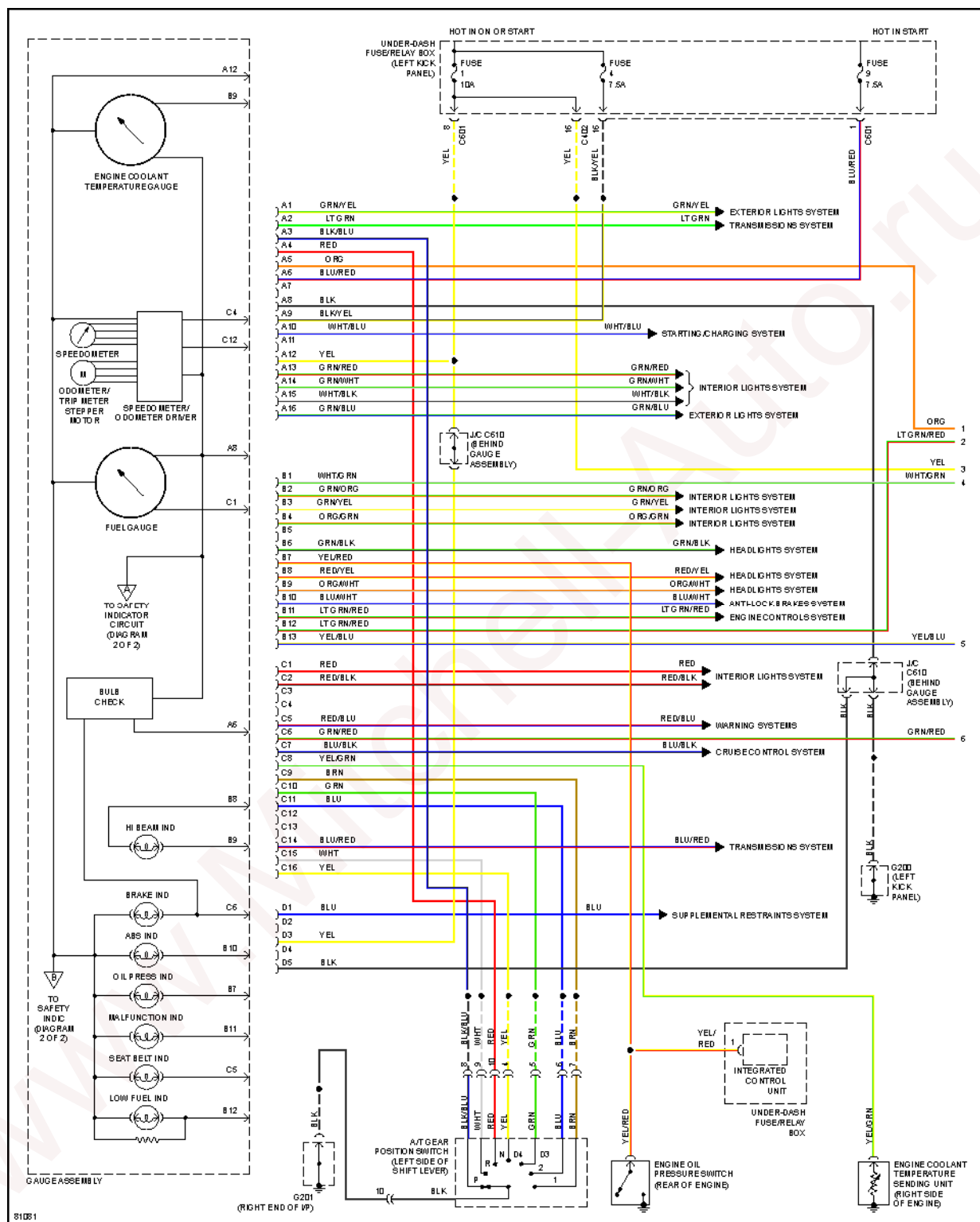
Fig. 21: Instrument Cluster Circuit (1 of 2)
