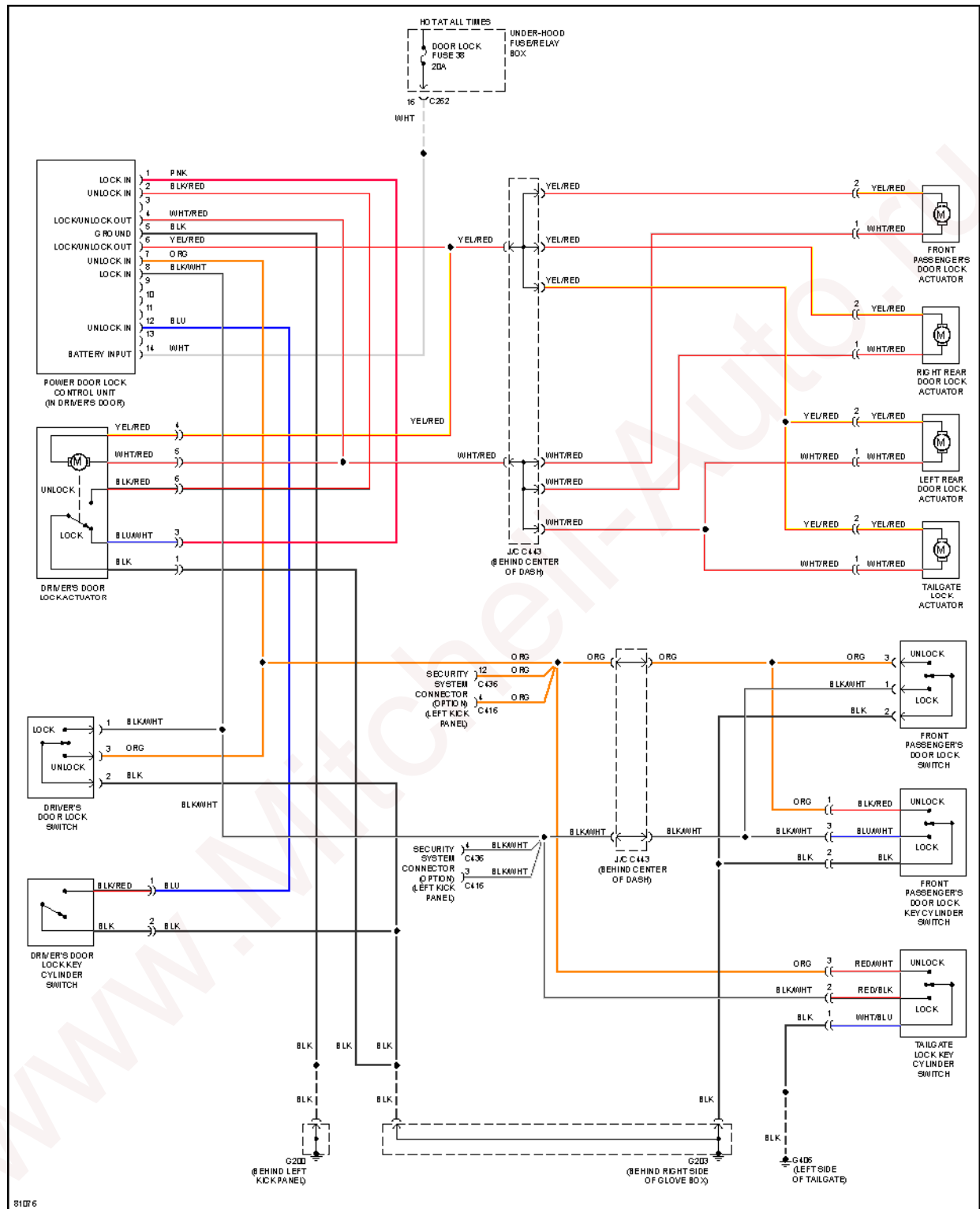
Fig. 31: Power Door Lock Circuit, W/O Keyless Entry
