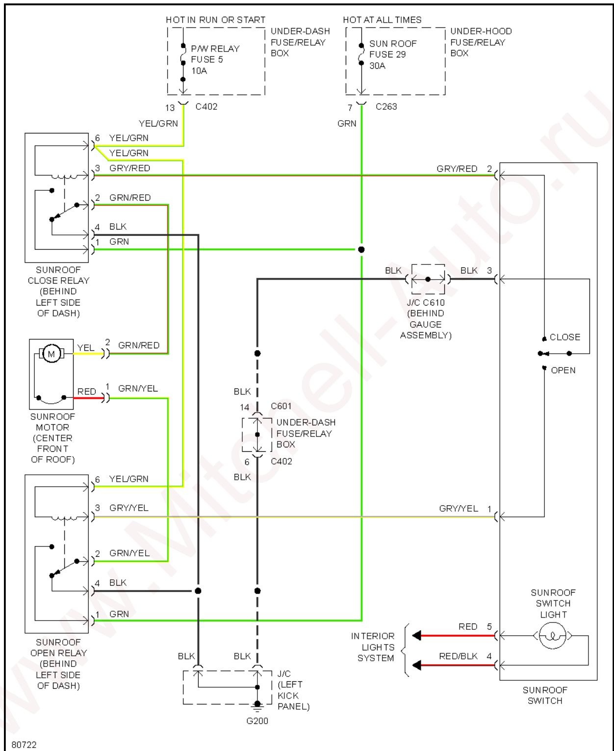
Fig. 34: Moonroof Circuit
