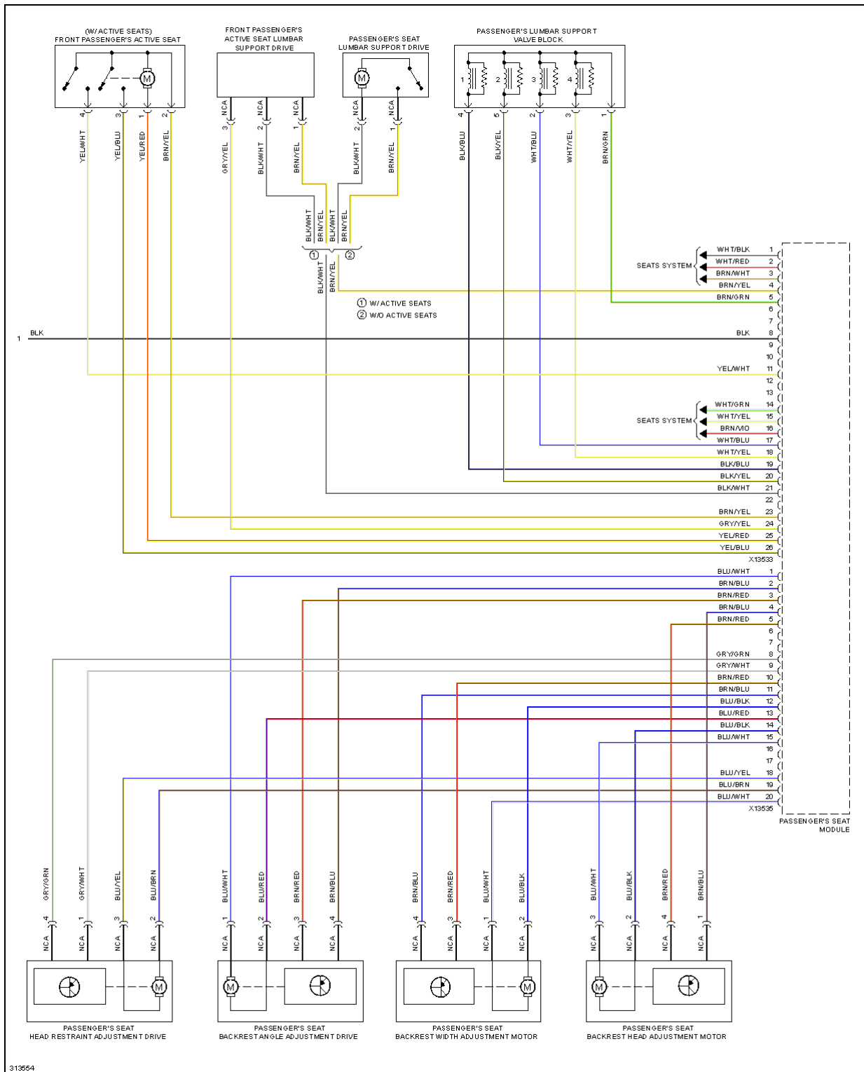
Fig. 63: Passenger's Memory Seat Circuit (2 of 2)
