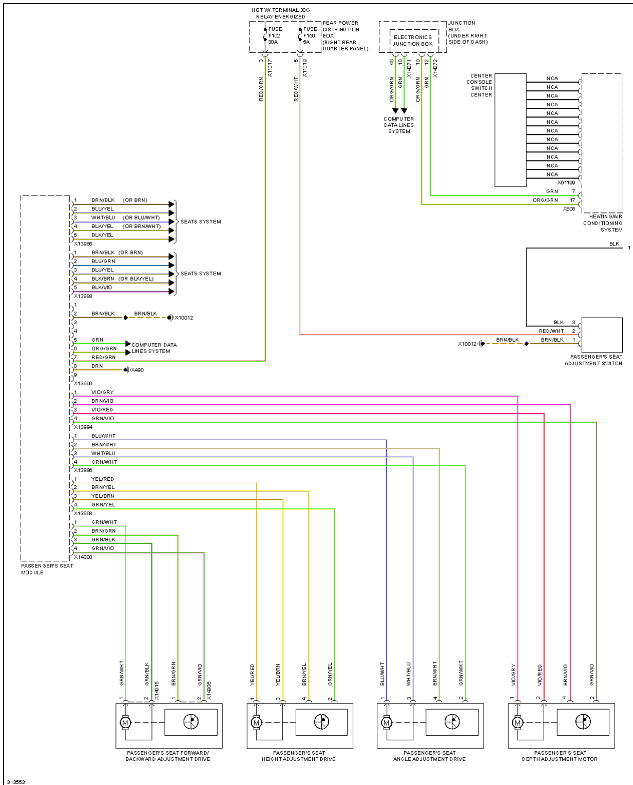
Fig. 62: Passenger's Memory Seat Circuit (1 of 2)
